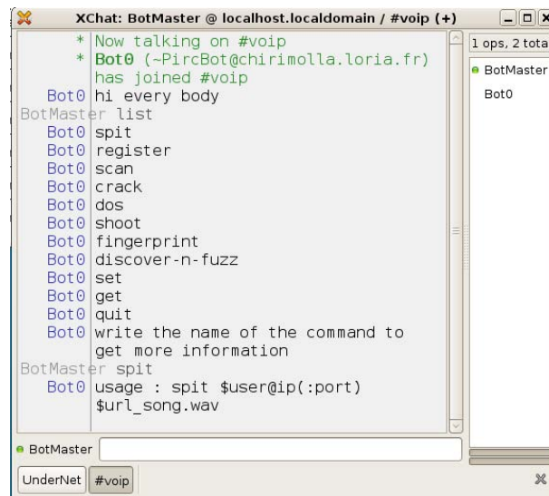
Figure 7.7: Screen view of the bot master
