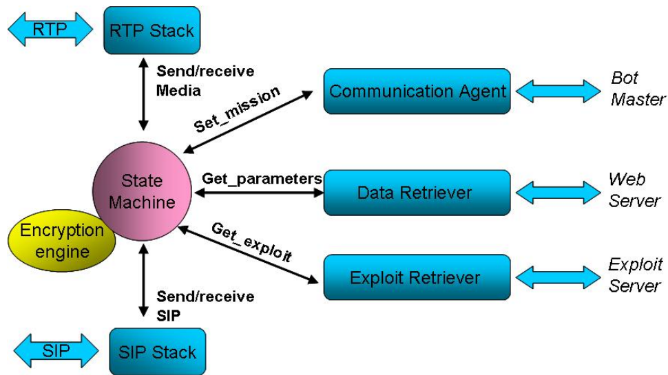
Figure 7.2: VoIP bot architecture
