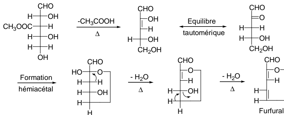
Figure 15. Formation du furfural
