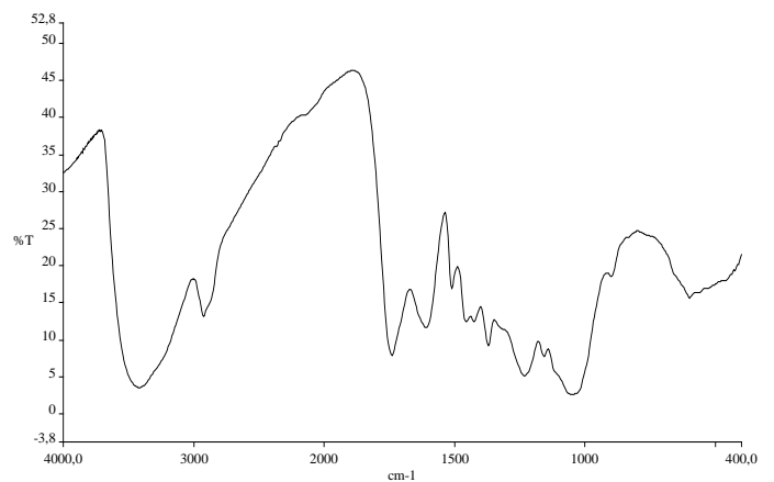
Acetylated heat treated sawdust, ML = 29.2 % WG = 0%
