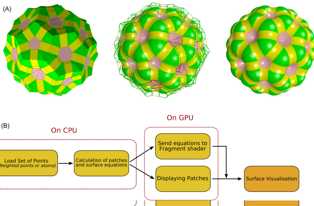
Fig. 5. (A) Visualization of the C_{60} fullerene molecule. On the left, the primitive envelope of patches. On the right, the ray-casted result. At the center, the combined ray-casted and primitive representations. Colors on the surface correspond to the different mixed cells: green = shrunk Voronoï cells, red = shrunk tetrahedra, yellow = H1 patches and pink = H2 patches. (B) Pipeline of our algorithm.
