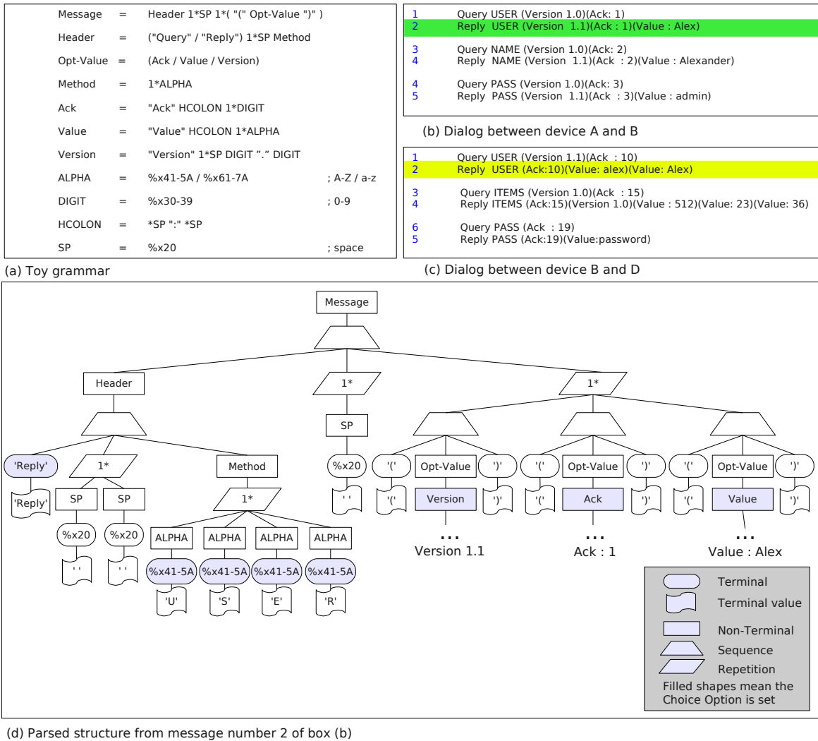
Figure 6.2: Parsed structure grammar
