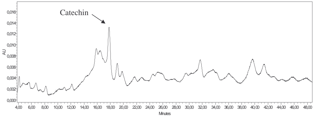
Figure 3: Acetonic extractives chromatogram at 280nm of wood beech dried at 55°C
