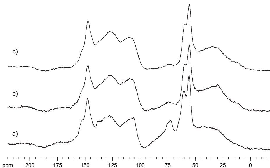
Fig. 4. CP/MAS ^{13}\text{C} NMR spectra of thermally modified or not beech lignin fraction: (a) unmodified lignin fraction; (b) heat treated at 240\text{ }^{\circ}\text{C} during 5 h30, WL = 16.9%; (c) heat treated at 240\text{ }^{\circ}\text{C} during 21 h, WL = 17.7%.
