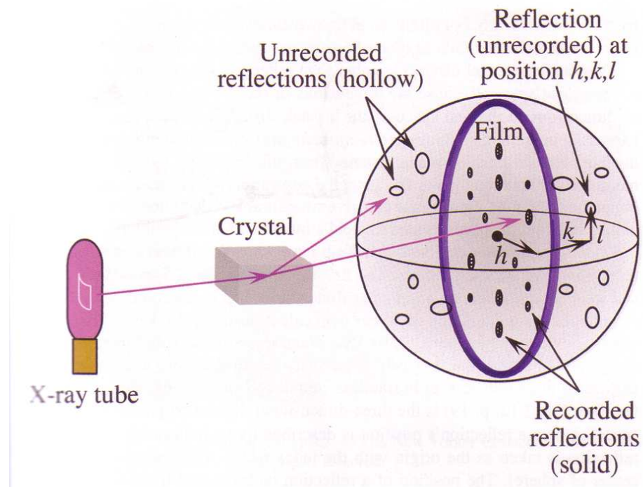
Figure 1.5 Crystallographic data collection, showing reflections measured at one particular crystal orientation (solid, on the film) and those that could be measured at other orientations (hollow, within the sphere but not on the film). Each reflection is located by its indices h , k and l . The relationship between measured and unmeasured reflections is more complex than shown here (Rhodes 2006).
