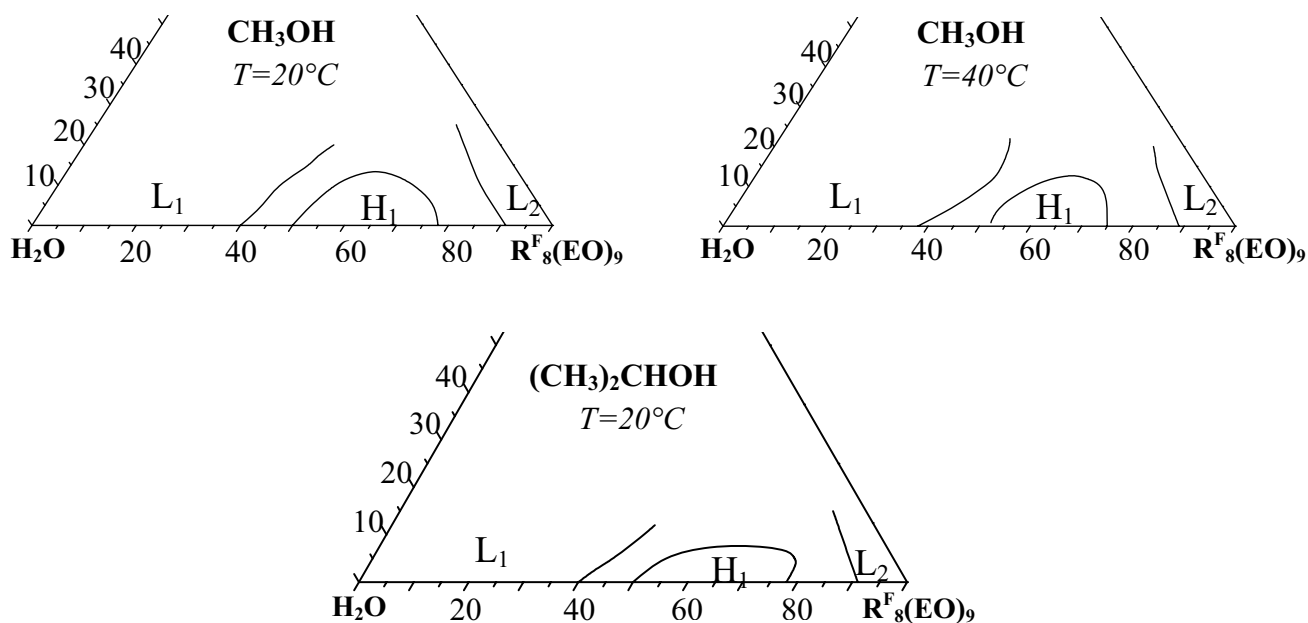
Figure V-1. Phase diagrams (wt %) of R^F_8(EO)_9/CH_3OH /water systems at 20^\circ C and 40^\circ C , and R^F_8(EO)_9/(CH_3)_2CHOH /water system at 20^\circ C .
