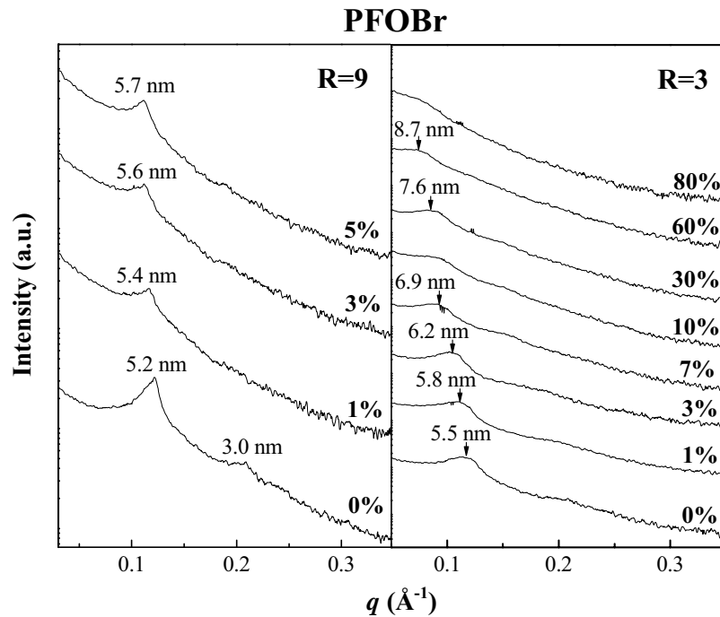
Figure IV-II. SAXS patterns of the material prepared from R_8^F(EO)_9 with different of concentrations of PFOBr for R=9 and 3.
