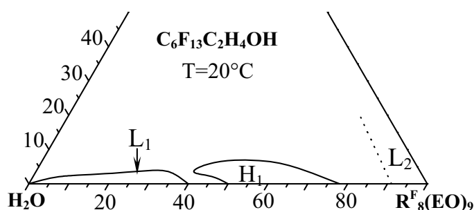
Figure V-28. Phase diagram (wt %) of R^F_8(EO)_9 / C_6F_{13}C_2H_4OH /water system at 20 °C.
