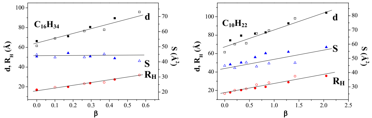
Figure III-7. Evolution of the structural parameters of the hexagonal liquid crystal phase with C_{16}H_{34} ( \blacksquare , \blacktriangle and \bullet : R = 1 ; \square , \triangle and \circ : R = 0.82 ) and C_{10}H_{22} ( \blacksquare , \blacktriangle and \bullet : R = 1.50 ; \square , \triangle and \circ : R = 0.82 ): d (repetition distance), R_H (hydrophobic radius), S (cross-sectional area).
