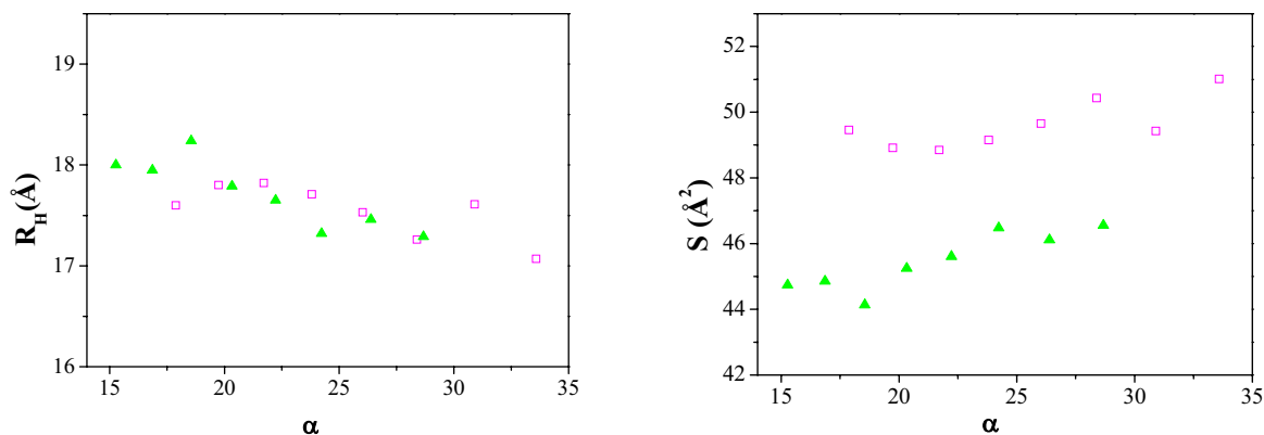
Figure V-25. Evolution of the hydrophobic radius ( R_H ) and cross sectional area ( S ) as a function of \alpha in H_1 for R_S = 32.3 (▲) and the pure surfactant (◻)
