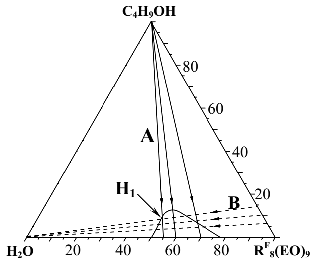
Figure V-8. Schema of two independent series of experiments (pathway A and B) for the hexagonal liquid crystal phase domain of R^F_8(EO)_9 / n -butanol /water system
