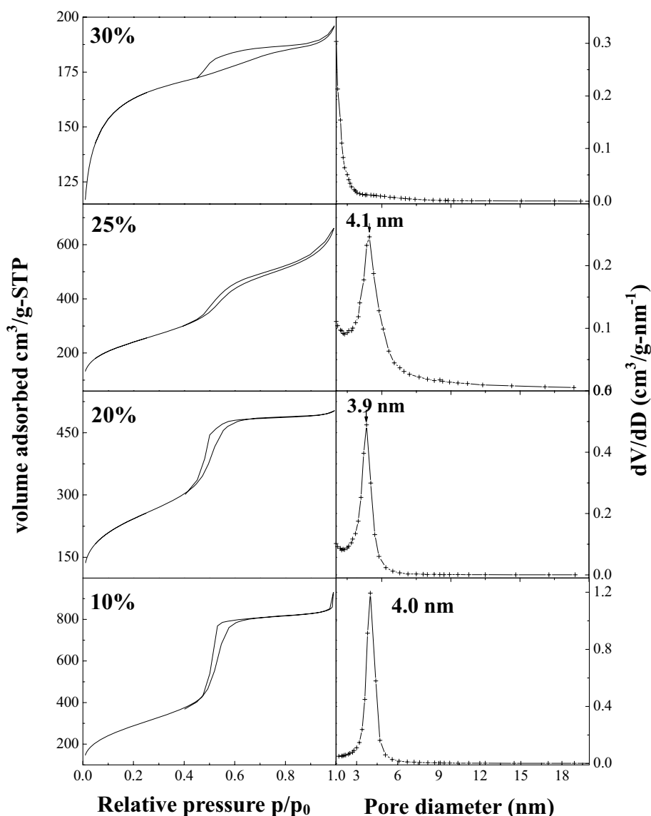
Figure III-4. Evolution of nitrogen adsorption- desorption isotherm and the corresponding BJH pore size distribution curve with different concentrations of R^H_{12}A(EO)_9
