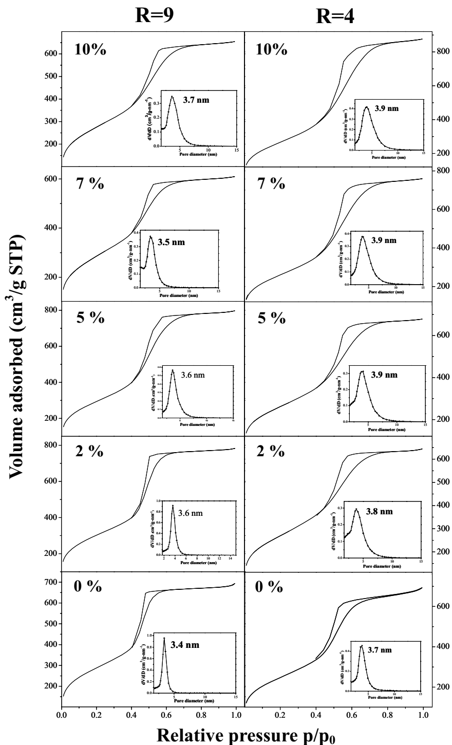
Figure V-20. Evolution of nitrogen adsorption-desorption isotherm and the corresponding BJH pore size distribution curve (insert) with different concentrations of n -butanol for R=9 and R=4 at pH 0.025 and 40 °C.
