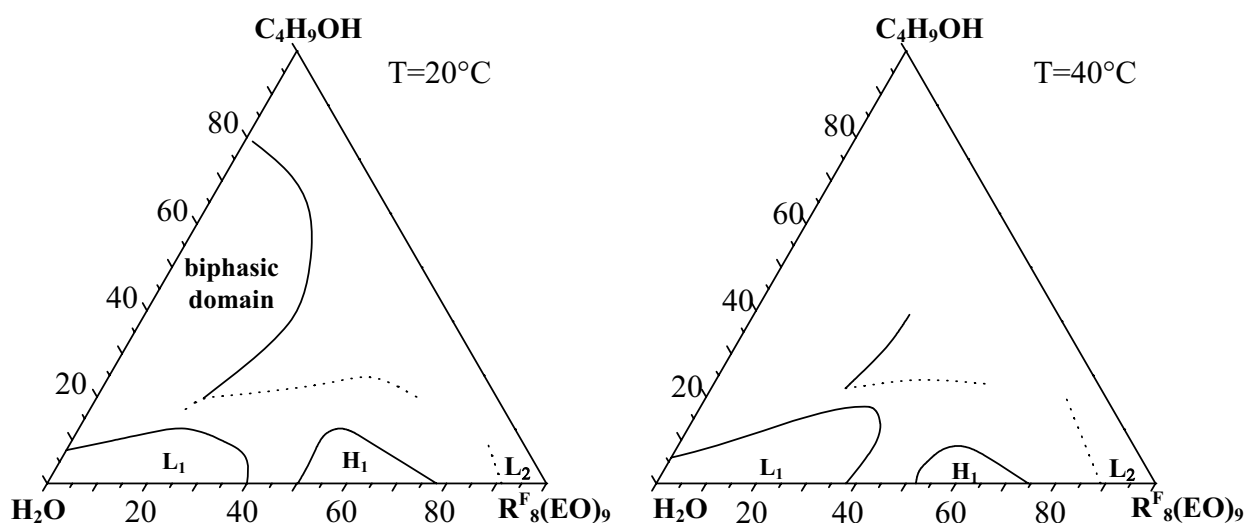
Figure V-7. Phase diagram (wt %) of R_8^F(EO)_9/C_4H_9OH/water system at 20^\circ C and 40^\circ C .
