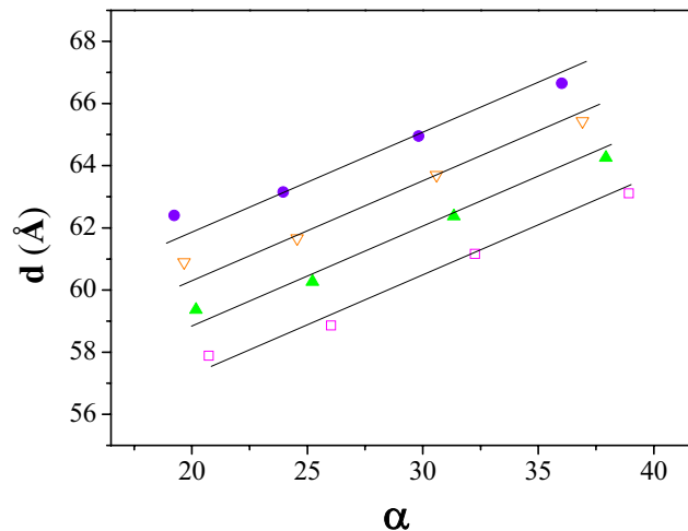
Figure V-31. Evolution of the d -spacing ( d ) as a function of \alpha (molar number of water per surfactant) in H_1 for □: R_S = 0.02 ; ▲: R_S = 0.04 ; ▽: R_S = 0.06 ; ●: R_S = 0.09 .
