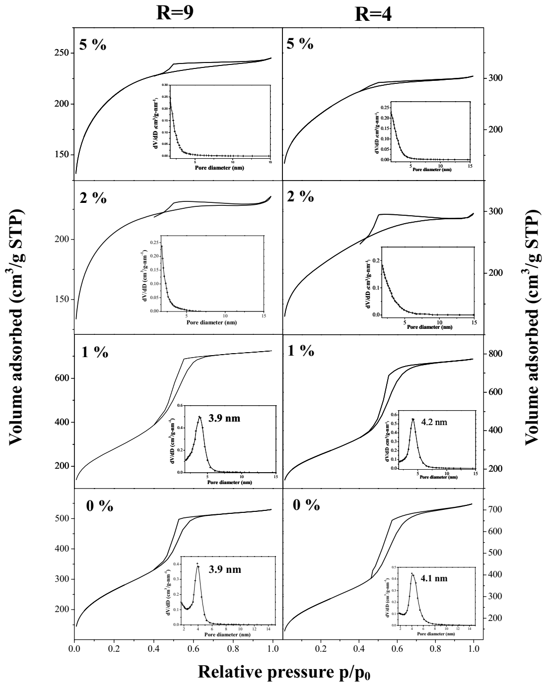
Figure V-34. Evolution of nitrogen adsorption-desorption isotherm and the corresponding BJH pore size distribution curve (insert) with different concentrations of fluorinated octanol for R=9 and R=4 ; TMOS is added at 20^\circ\text{C} and \text{pH}=2
