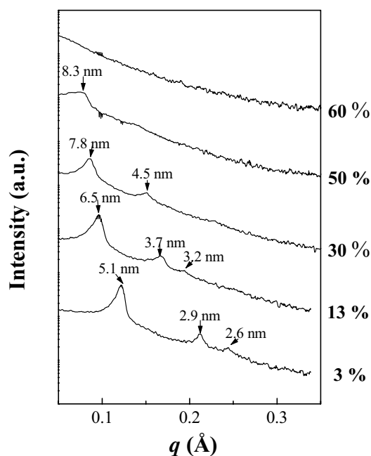
Figure IV-29. SAXS pattern of the material prepared from \text{R}^{\text{F}}_7(\text{EO})_8 with PFOBr at pH 0.025 and 20 ^{\circ}\text{C}
