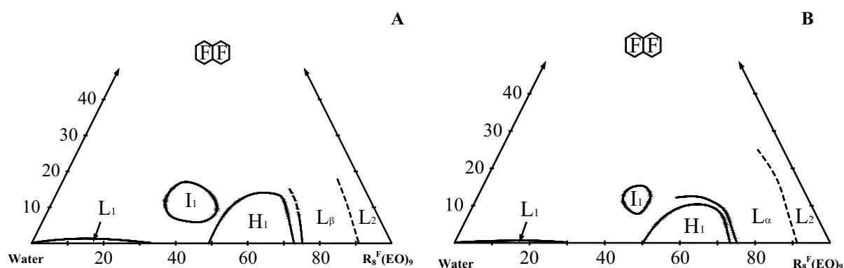
Figure IV-4. Partial ternary diagram of R^F_8(\text{EO})_9 /Perfluorodecalin/ \text{H}_2\text{O} at 25^\circ\text{C} (A) and 50^\circ\text{C} (B) L_1 =micellar solution; I_1 =cubic phase; H_1 =hexagonal phase; L_\beta =gel phase; L_2 =reverse micelle [195]
