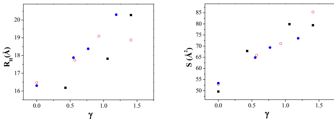
Figure V-23. Evolution of the hydrophobic radius ( R_H ) and cross sectional area ( S ) as a function of \gamma in H_1 for ■ : R = 1.00 ; ○ : R = 0.67 ; ● : R = 0.43
