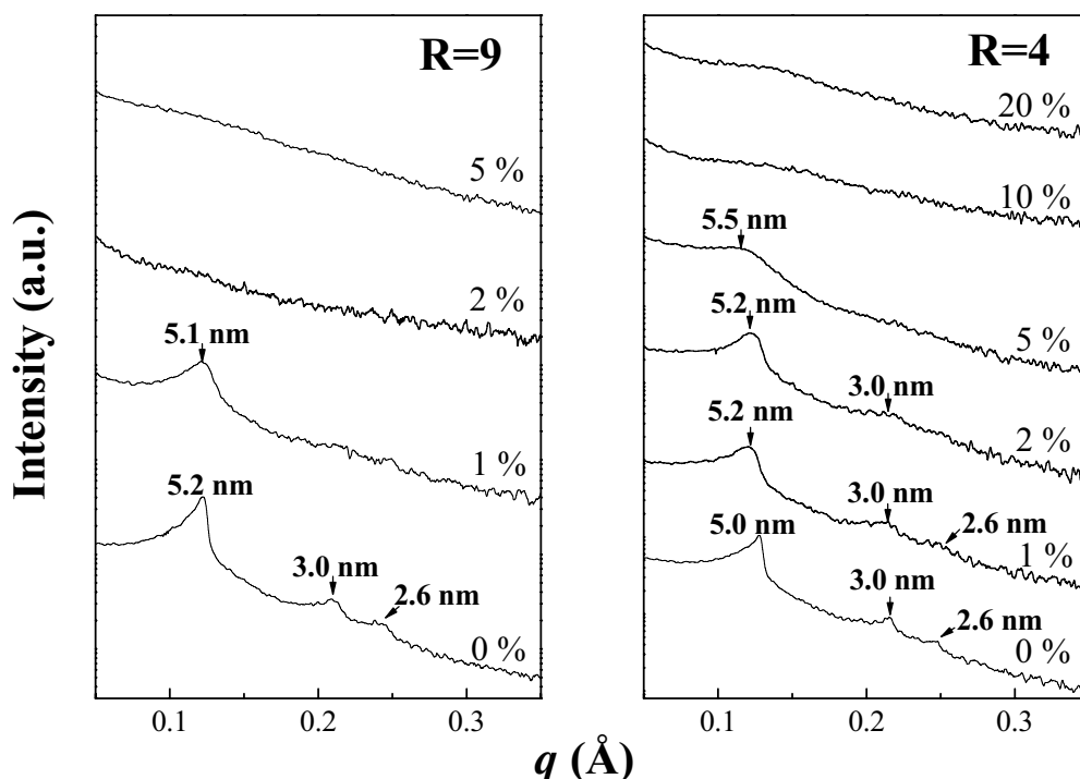
Figure V-26. SAXS patterns of the materials prepared from the R^F_8(\text{EO})_9 -based system with different concentrations of octanol for R=9 and 4 at pH 2 and 40 °C.
