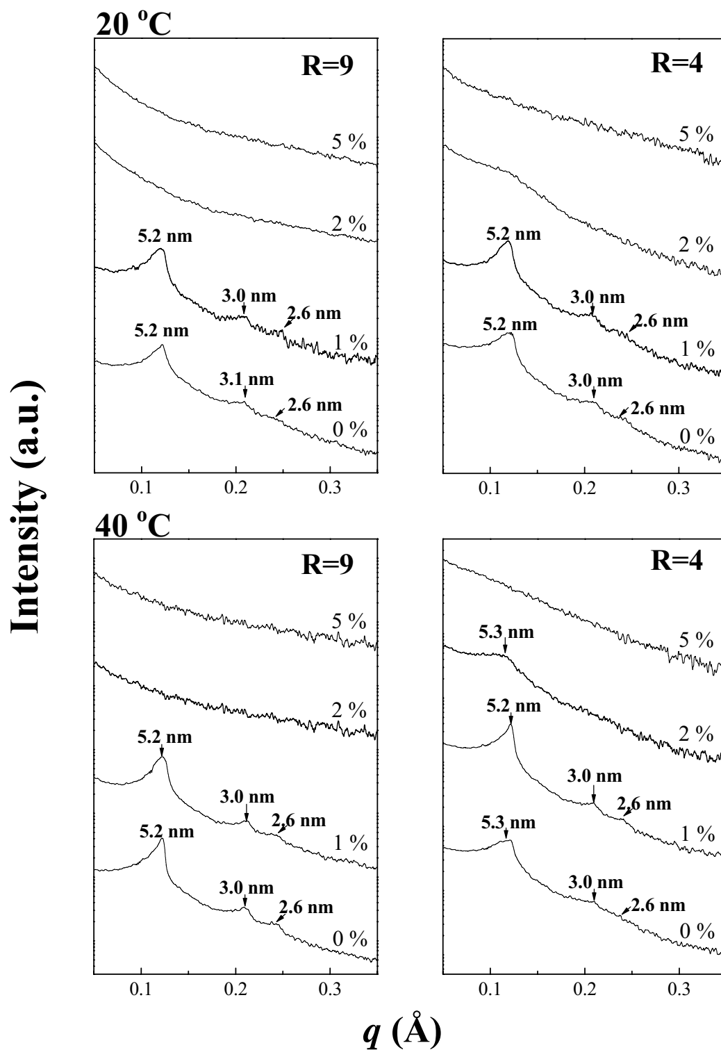
Figure V-33. SAXS patterns of the materials prepared from the R^F_8(EO)_9 -based system with different concentrations of fluorinated octanol for R=9 and R=4 ; TMOS is added at 20 °C or 40 °C at pH=2
