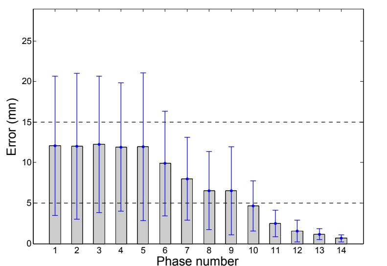
Figure 6.11: Average errors in remaining time prediction, per phase.
