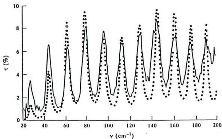
Fig. 11. FIR spectra at 10 K in the 20 – 200 \text{cm}^{-1} range.
