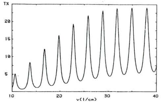
Fig. 5. Calculated spectrum for \Theta = 5 \text{ K} , assuming a 30 Å surface layer and a small number of quasi-particles with \nu_c = 1 \text{ cm}^{-1} . This number is given by a \Theta^{1.5} law. The agreement with observation (Fig. 2) is quite good.
