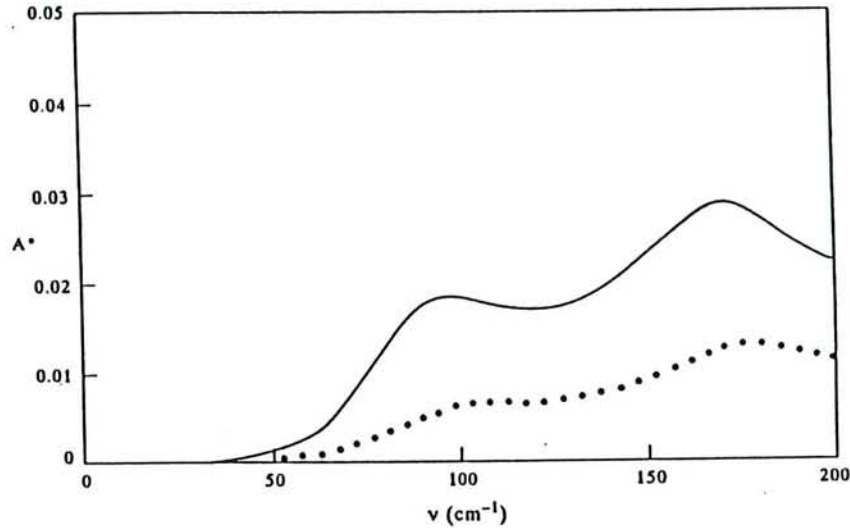
Fig. 15. Absorptivity A^* of bulk of ideal GdBaCuO at T = 10 K and of the ideal YBaCuO considered in Ref. (7); R_1 = A^* \times 94.2 \Omega .
