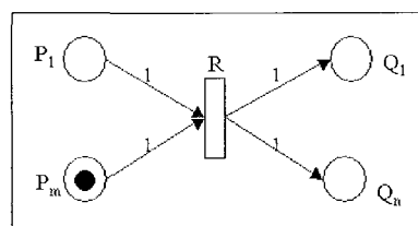
Figure 52: A Rule in Petri net representation.
