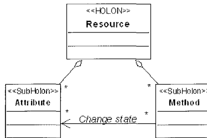
Figure 27: Attributes and Methods Holonic-Classes.
