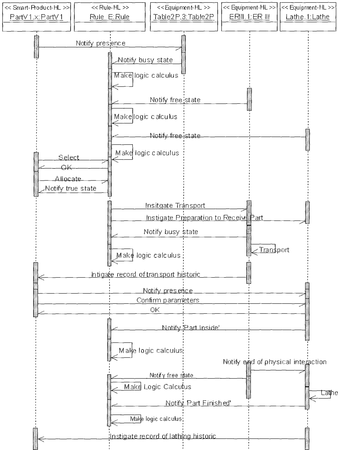
Figure 62: Smart-Product-HL allocating Rule E'.
