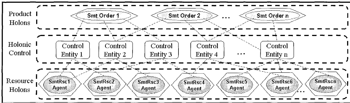
Figure 6: Holonic Discrete Control System (HDCCS) functions.
