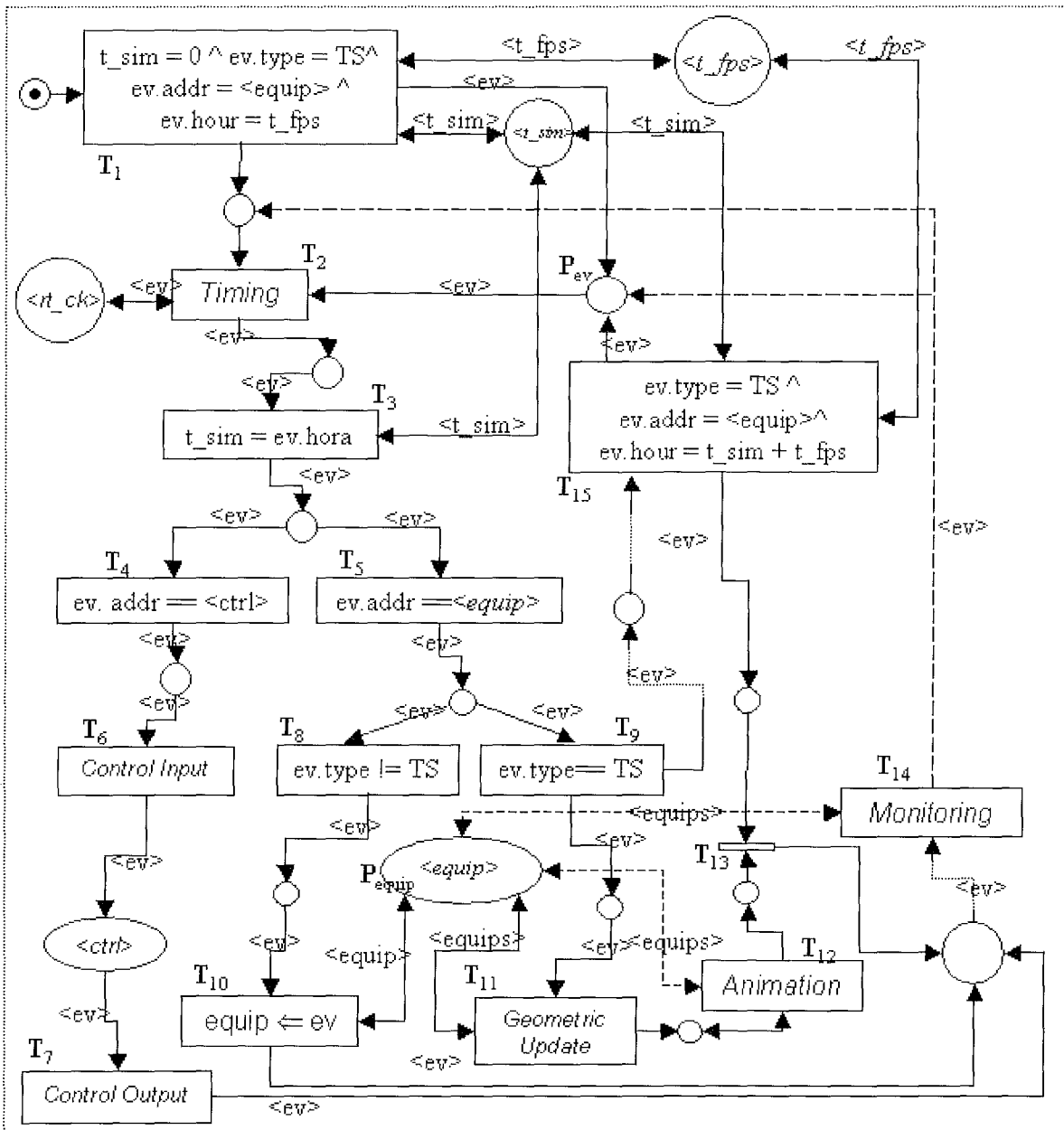
Figure 20: Petri Net of the Simulator Kernel.
