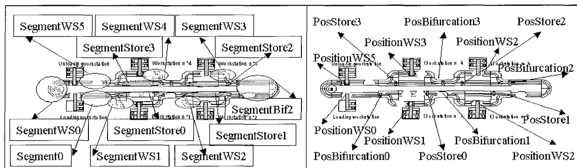
Figure 73: Segments and positions in the conveyor.
