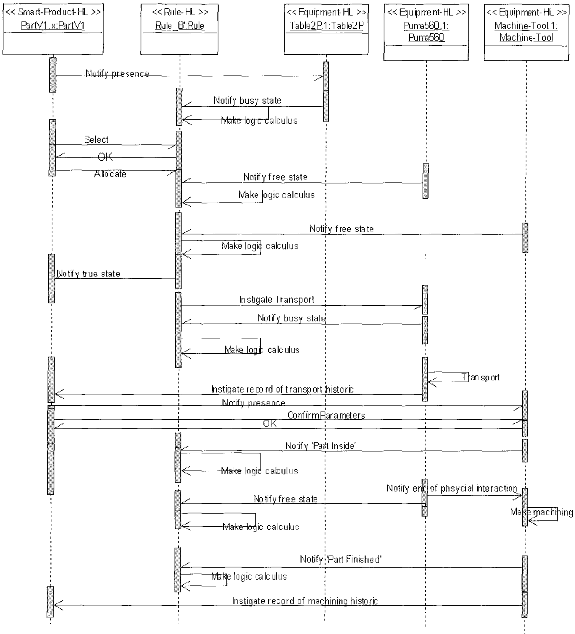
Figure 63: Smart-Product-HL allocating Rule B'.
