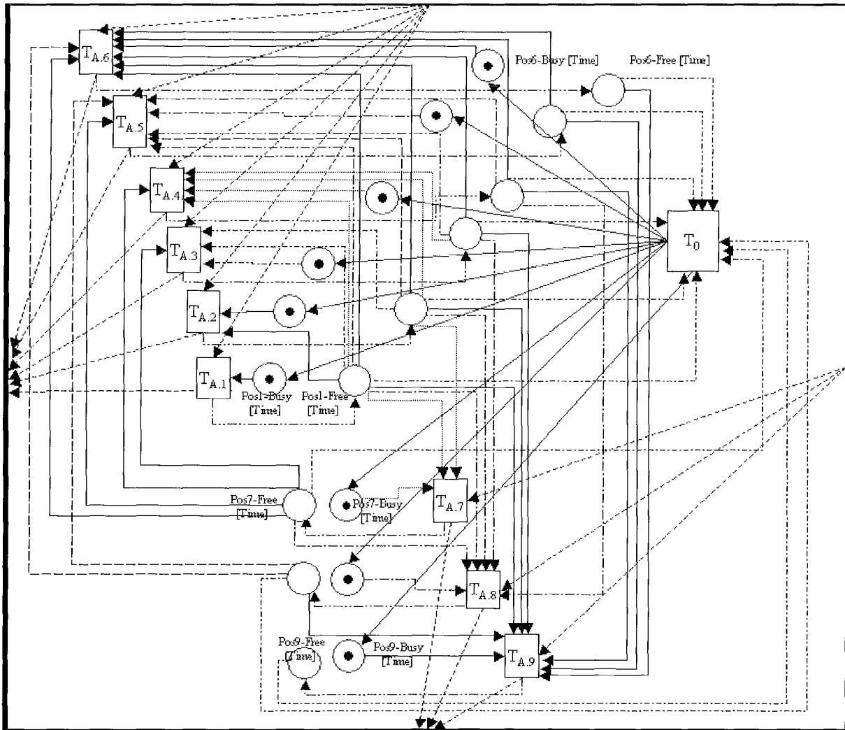
Figure 54: Complementary subnet 102 .
