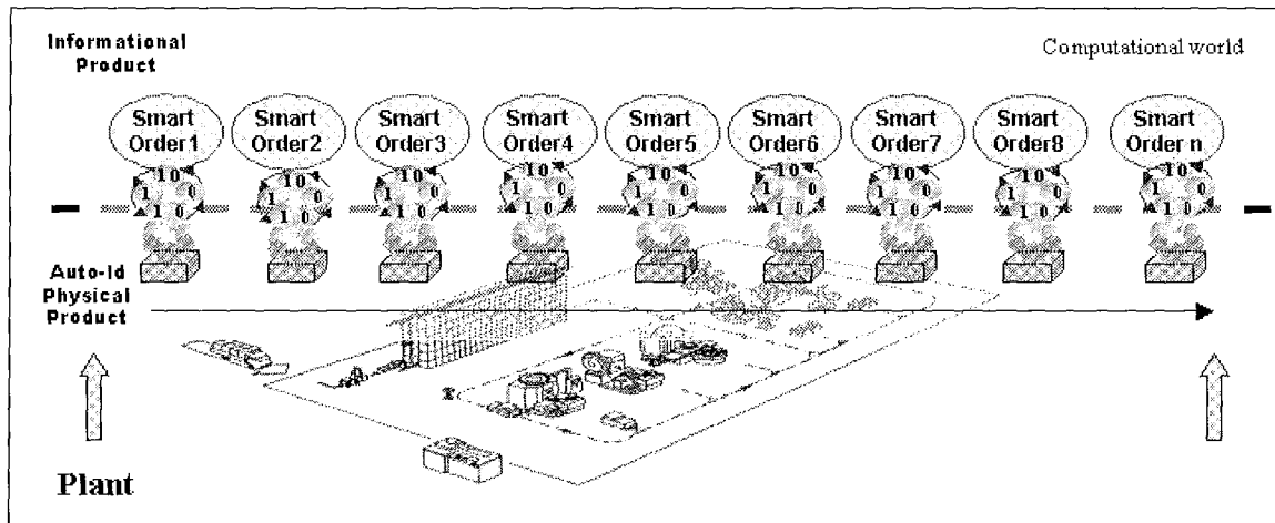
Figure 5: Flows consistence.
