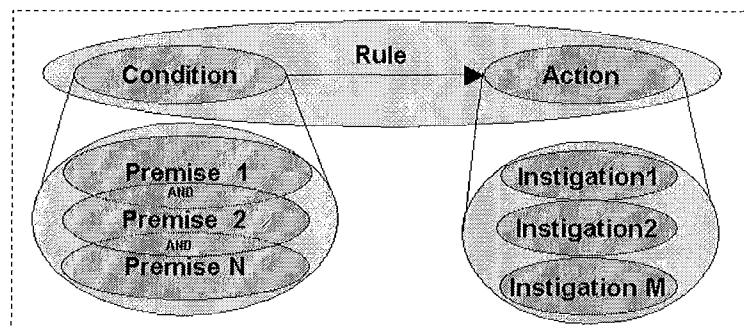
Figure 32: Control Entity.
