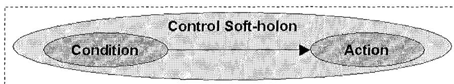
Figure 29: Control Entity.
