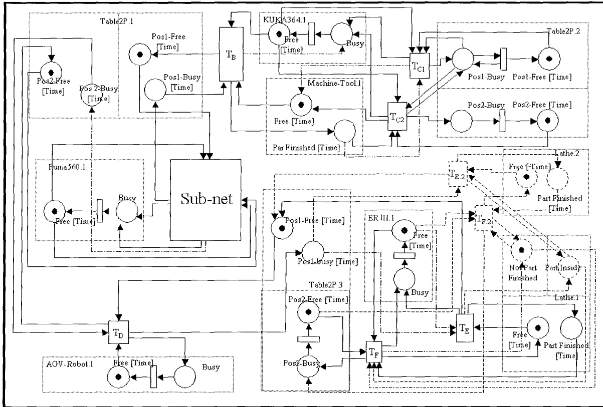
Figure 56: Control Improved.
