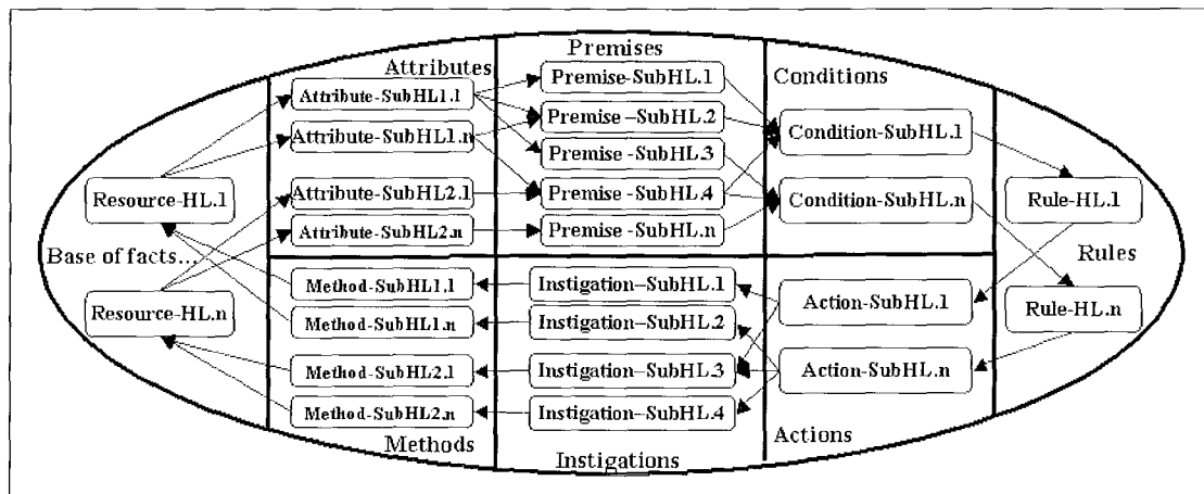
Figure 35: Notification mechanism.
