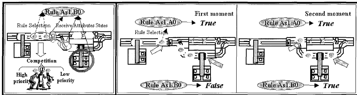
Figure 78: Flow issues.
