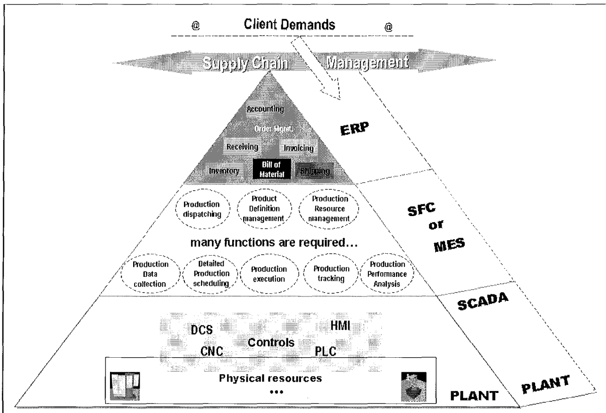
Figure 3: Enterprise Integration 4 .
