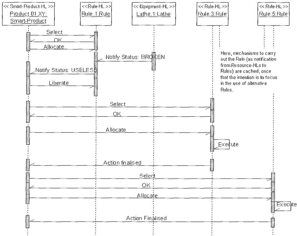
Figure 70: Alternative Rule.
