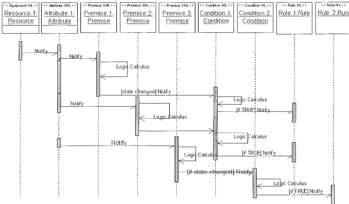
Figure 46: Sequence diagram to exemplify a notification chain.
