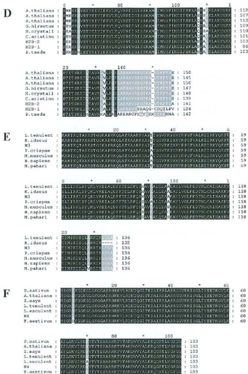
Fig. 1. Amino acid sequence alignment. Multiple alignment was done using Clustal-W. D ): Sequences of Pinus pinaster histone H2B-1 (clone Pp.ap22) and H2B-2 (clone RN02A03) with their orthologues from Arabidopsis thaliana (T47538), Arabidopsis thaliana (CAB88327), Arabidopsis thaliana (BAB08359), Gossypium hirsutum (O22582), Mesembrythemum crystallinum (BE037288), Cicer arietinum (CAB88668) and Pinus taeda (ST04G05). E ): Sequence of Pinus pinaster histone H3 (clone RN05H05) with its orthologues from Lolium temulentum (P11105), Rubus idaeus (AAG22548), Petroselinum crispum (P05203), Mus musculus (NP_038576), Homo sapiens (NP_003520) and Mus pahari (I49395). F ): Sequence of Pinus pinaster histone H4 (clone RN03C09) with its orthologues from Pisum sativum S60475, Arabidopsis thaliana S06904, Zea mays HSZM4, Lolium temulentum P02308, Lycopersicon esculentum P35057 and Triticum aestivum HSWT41. Dashes indicate gaps introduced to maximise the alignment. Identical and similar residues are shaded.
