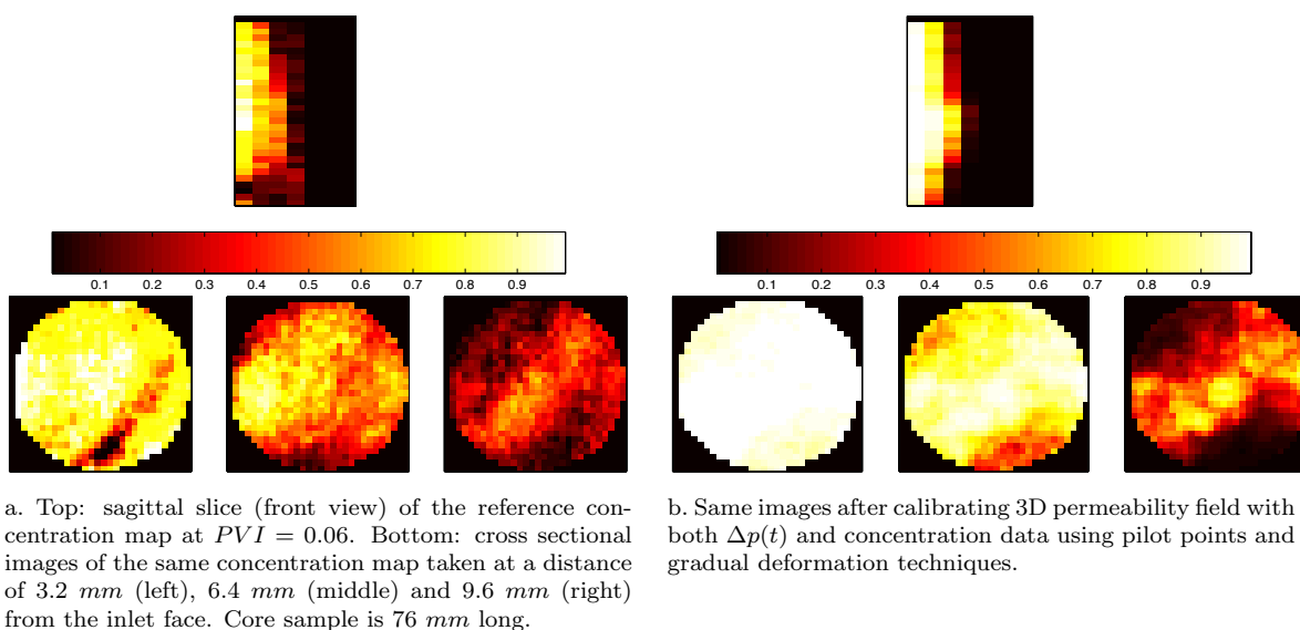
Figure 7.33: Comparison of the reference concentration map with the simulated one at PVI = 0.06 for the sample SG20. The injection is performed from right to left (inverse injection). The permeability field is calibrated to both \Delta p(t) and concentration data using the pilot point and the gradual deformation methods. The color bars show the injected fluid concentrations.
