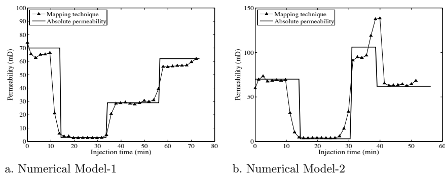
Figure 4.15: Comparison of the processed numerical permeabilities (triangles) with the absolute permeability of each block (lines) for Model-1 (a) and Model-2 (b) when performing miscible displacement.
