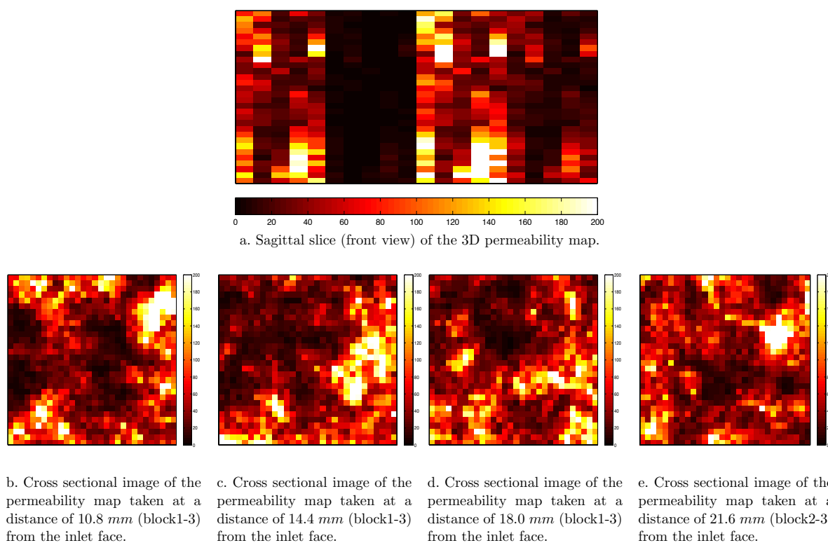
Figure 6.2: Cross sectional images of the 3D permeability map for Model-3. The Model is 72.0 mm long. The color bars show permeability.
