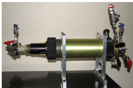
a. The X-ray core-holder used for CT imaging during our experiments.
