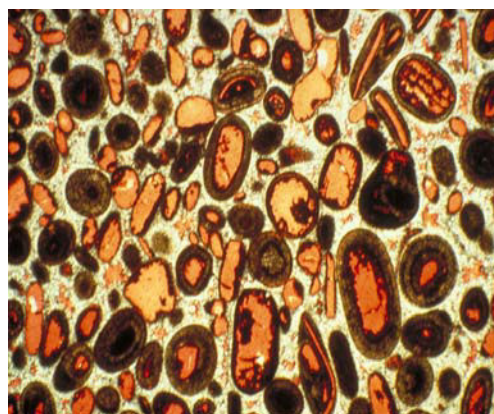
c. Thin section of Brauvilliers limestone.
