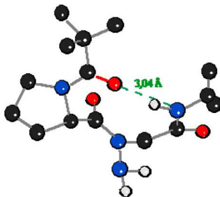
Figure 45 Structure cristalline du N -aminodipeptide PivProψ[CON(NH 2 )]GlyNHPr
