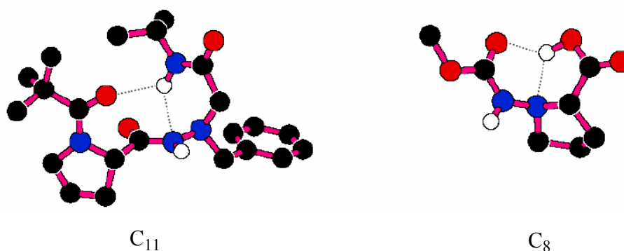
Figure 26 Repliements d'hydrazinopeptides
