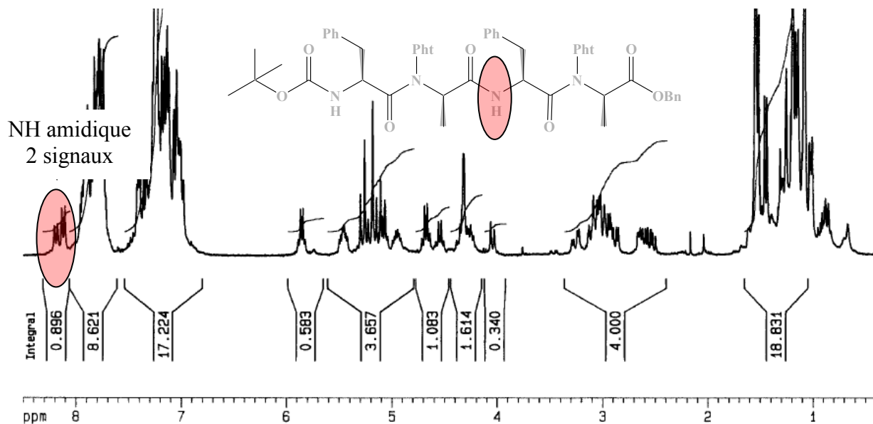
Figure 64 Spectre RMN ^1\text{H} ( \text{CDCl}_3 ) de Boc(Phe \psi [CON(Ph)])(R)Ala _2 OBn 9b
