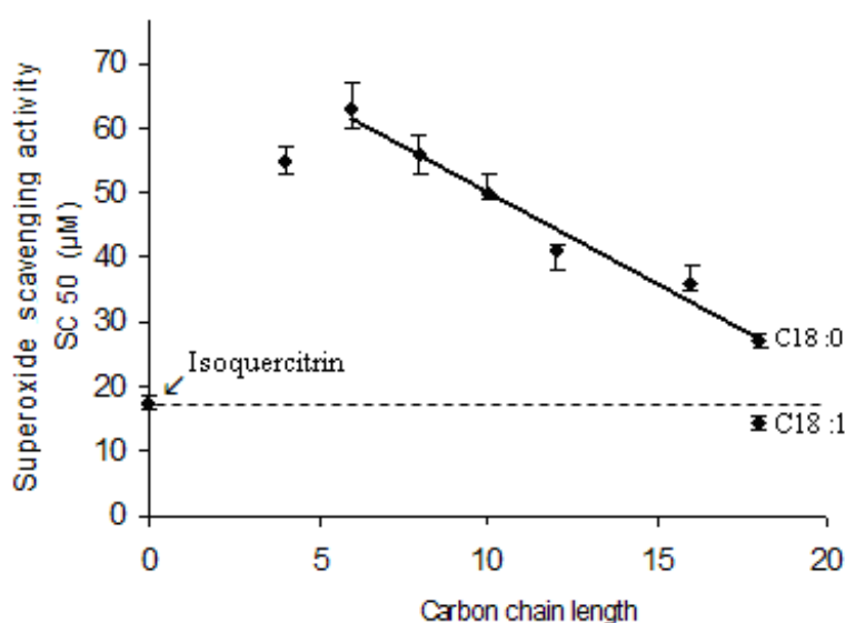
Figure 4: Superoxide scavenging potential of isoquercitrin and its esters depending on acyl chain length, expressed as SC 50 values (µM).
