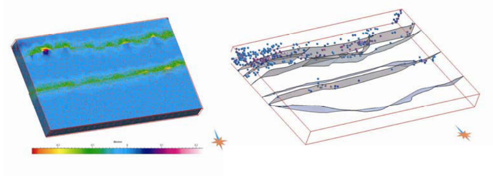
B) Compression on the Wasa Fault and the CLLF
