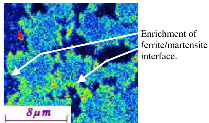
Figure IV.2. NanoSIMS carbon ion map for the 790°C-annealed sample.
