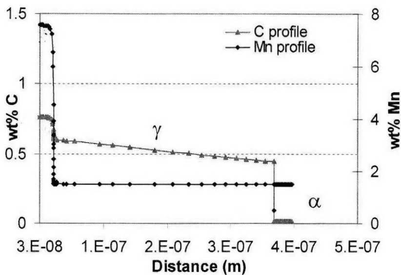
Figure IV.8. Carbon and Mn profiles in the \gamma calculated by DICTRA ® package after complete dissolution of cementite. Fe-0.15C-1.58Mn steel [GOUN05].
