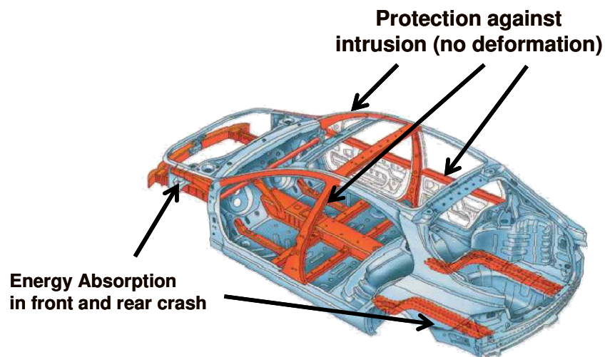
Figure 1. Typical applications of high strength steels for crash resistance (ArcelorMittal credit).
