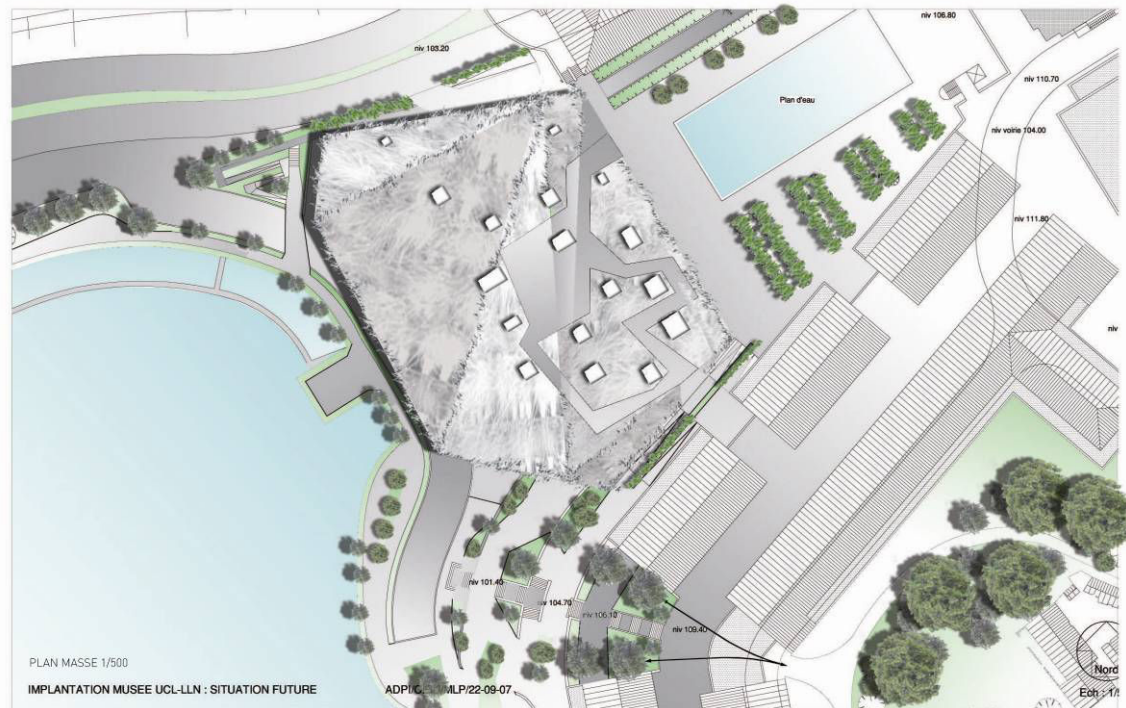
Figure 255. Plan masse.
