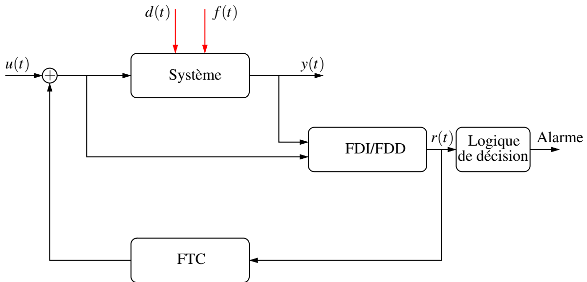
Figure 5.13 – Architecture FTC
