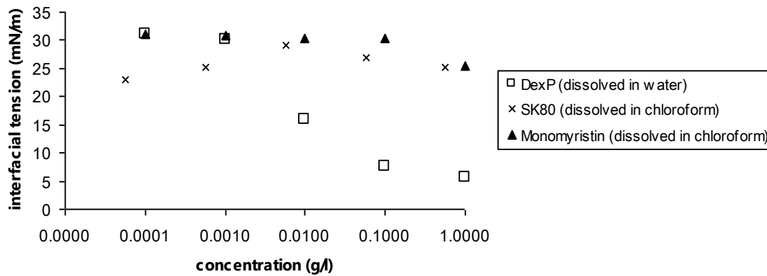
Figure 32 Chloroform to water interfacial tension of solution of DexP 20 , Glycerol ester of oleic acid (SK80) and monomyristin
