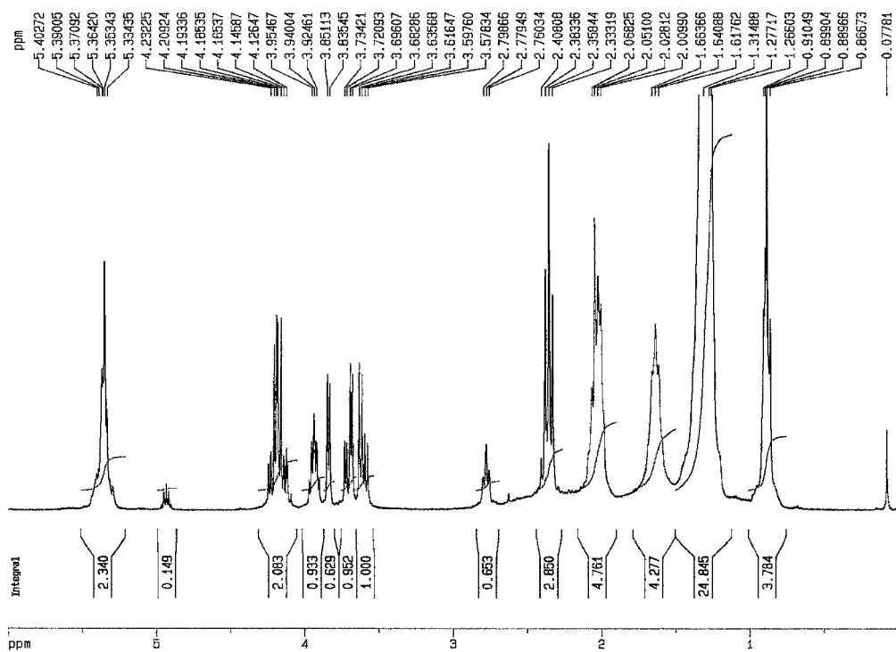
Figure 22 ^1\text{H} NMR spectrum of purified biosurfactant, in \text{CDCl}_3 , 300 MHz
