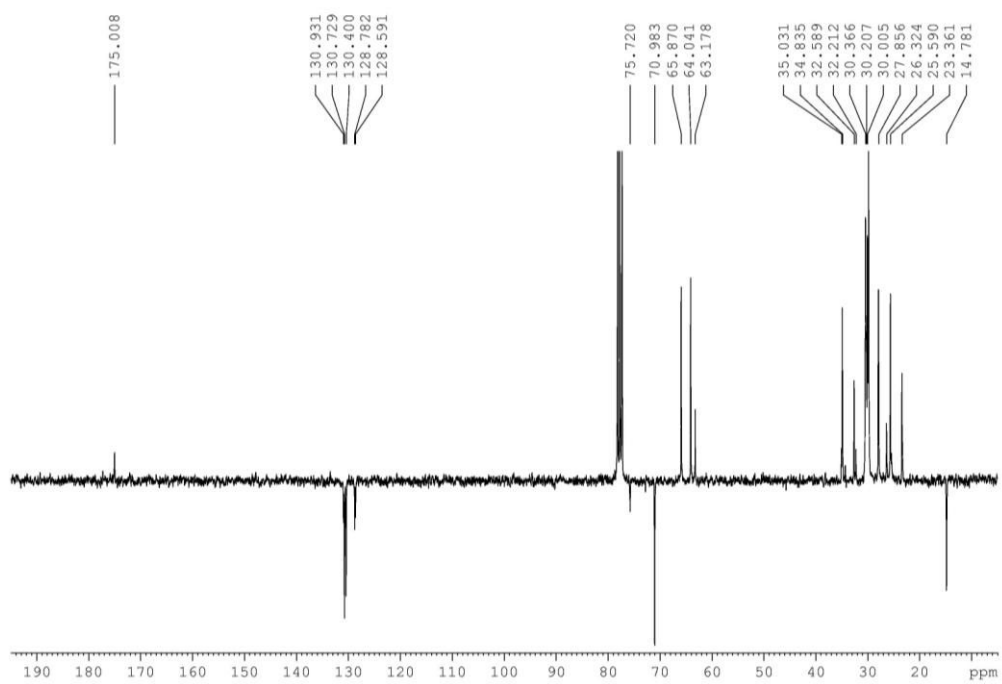
Figure 23 ^{13}\text{C} NMR spectrum of purified biosurfactant, in \text{CDCl}_3 , 300 MHz
