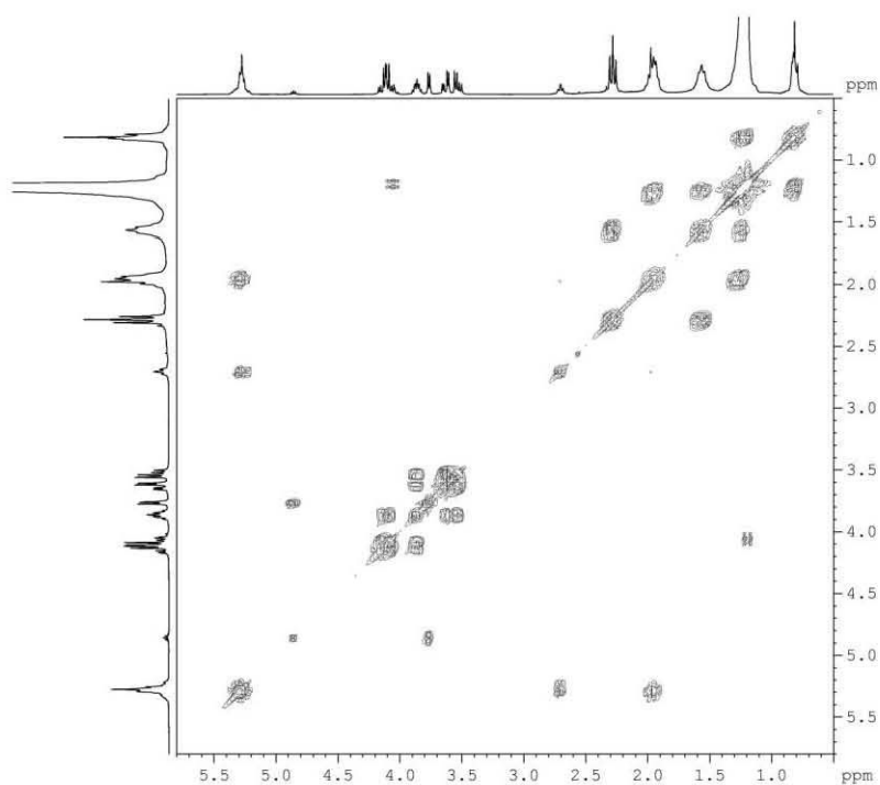
Figure 24 2D spectrum (HSQC) of purified biosurfactant, in CDCl 3 , 300 MHz
