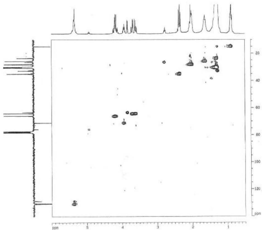
Figure 24 2D spectrum (HSQC) of purified biosurfactant, in CDCl 3 , 300 MHz
