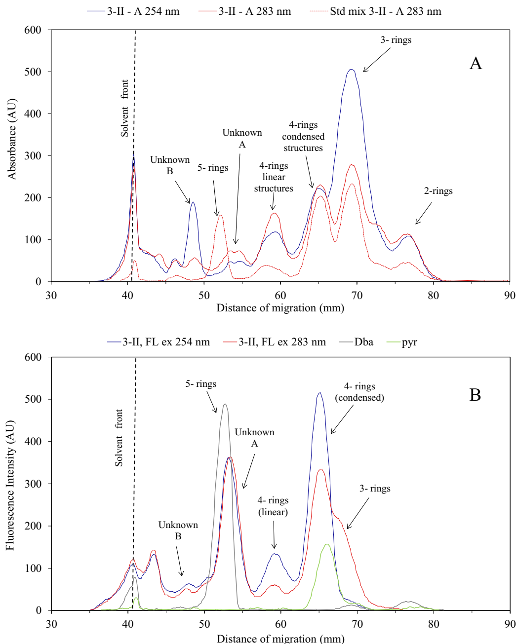
Figure 23: Chromatograms of sample 3-II (Fe/olivine), and the synthetic sample 3-II on HPLTC Silica gel 60 RP-18 with concentrating zone plate (migration at -23^{\circ}\text{C} ), recorded at different wavelengths in absorption and fluorescence mode (table 1 –j)
