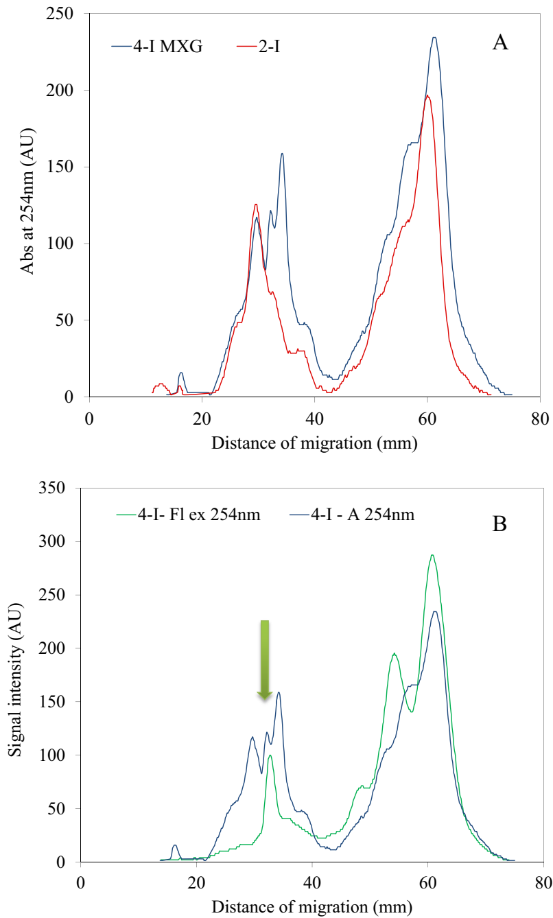
Figure 15: (A) Chromatograms of samples 2-I (almond shells, olivine, \approx 800^{\circ}\text{C} ) and 4-I (MXG, olivine, 800^{\circ}\text{C} ) on HPLC Nano-SIL 20 plate recorded at \lambda = 254\text{ nm} . (B) Chromatograms of sample 4-I on HPLC Nano-SIL 20 plate in fluorescence and absorption mode.
