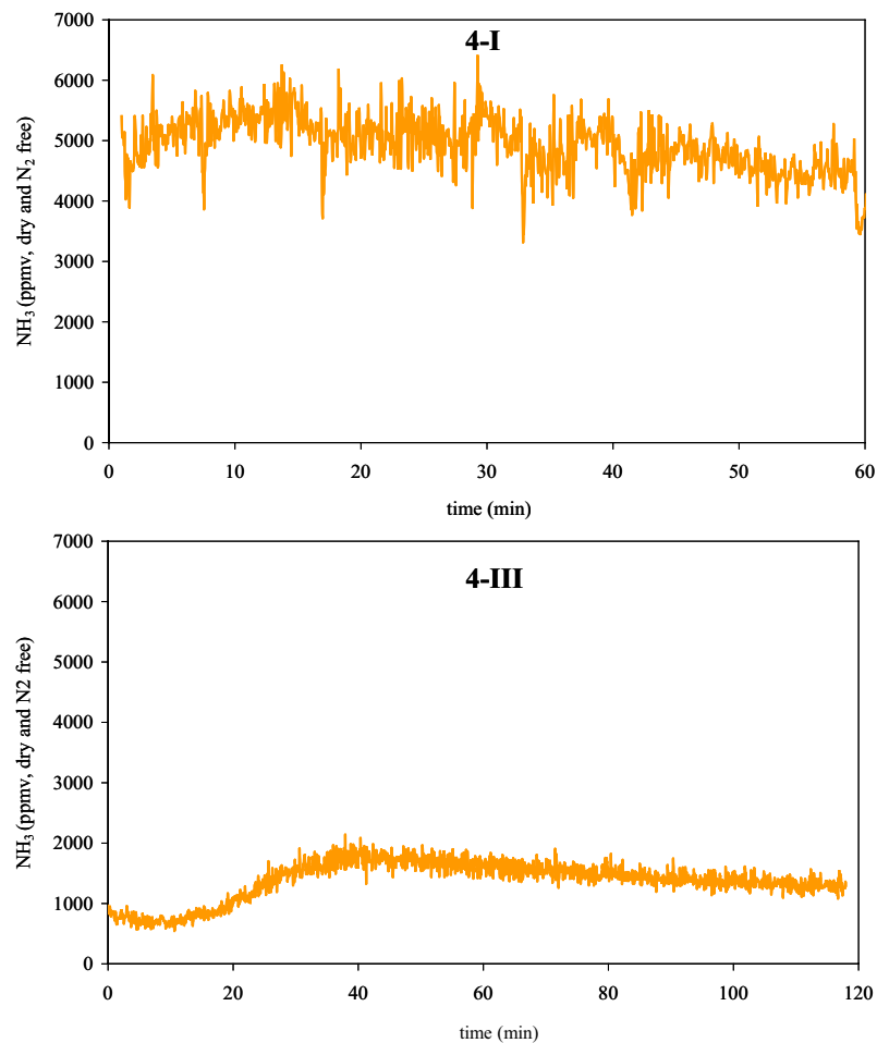
Figure 27: Ammonia concentration as a function of gasification time for test 4-I (800°C – olivine) and test 4-III (800°C – 4wt % Ni/olivine)
