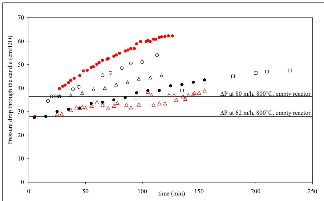
Figure 24: Pressure drop across the catalytic filter candle, as a function of time; filtration velocity: (○) 81 m/h, (Δ) 79 m/h, (●) 63 m/h, (□) 62 m/h (previous tests); (●) 77m/h – test 3-IV, (Δ) 60 m/h – test 3-V.
