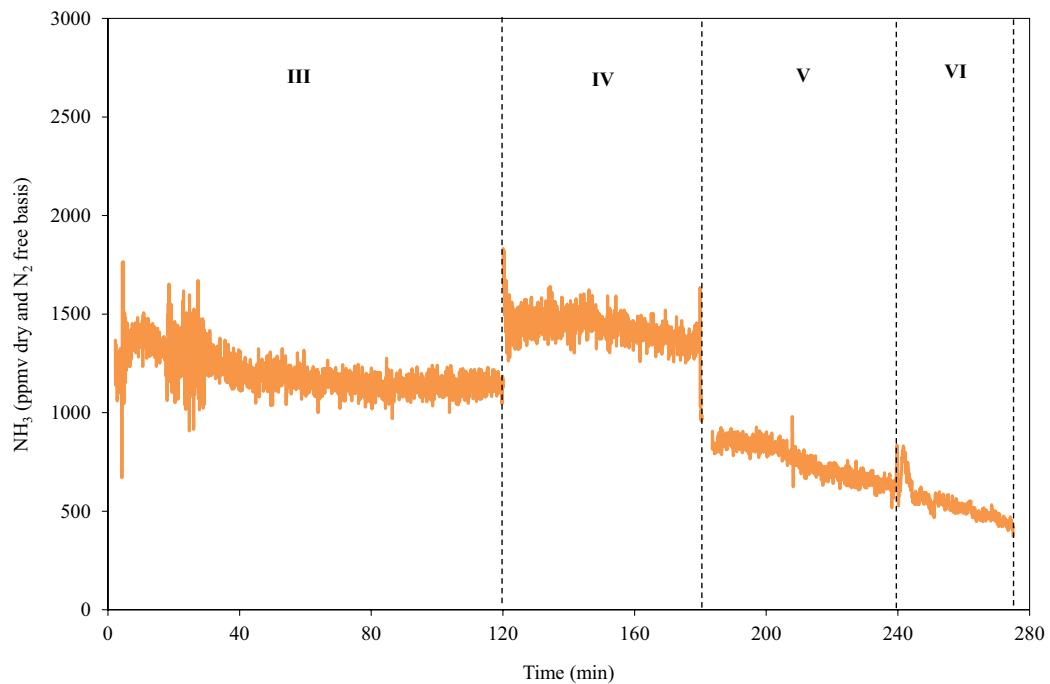
Figure 13: NH 3 in the syngas as a function of gasification time. Tests 1-III – 1-VI: Steam gasification with the catalytically activated filter candle with “catalytic layer” design
