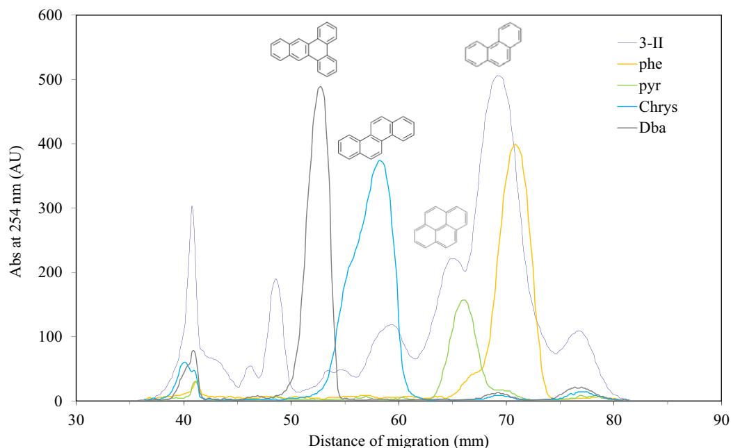
Figure 21: Chromatograms of sample 3-II (Fe/olivine) and four selected standards on HPTLC Silica gel 60 RP-18 with concentrating zone plate (migration at -23^{\circ}\text{C} ), recorded at \lambda = 254 \text{ nm} (table 1 –j)
