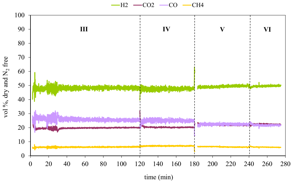
Figure 12: Syngas composition as a function of gasification time. Tests 1-III-VI: Steam gasification of almond shell with olivine bed inventory + catalytically activated filter candle with “catalytic layer” design
