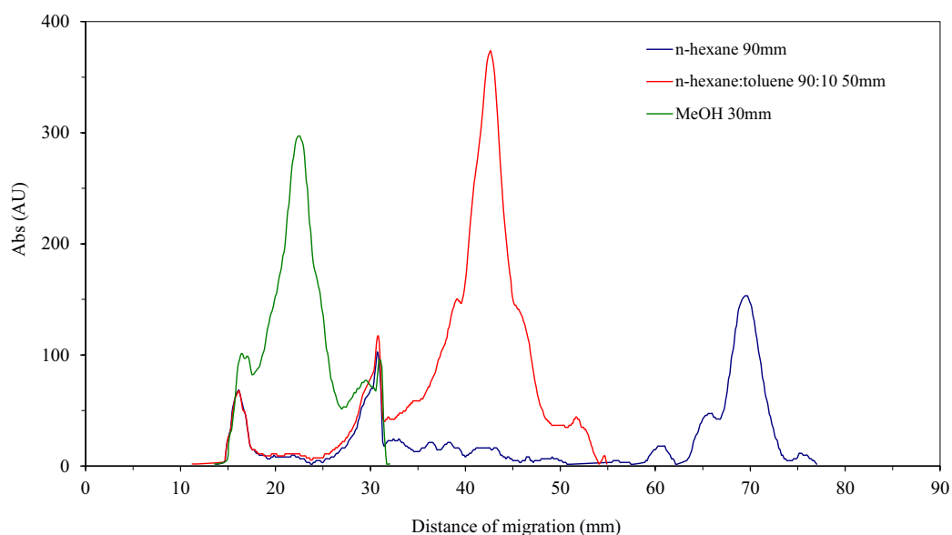
Figure 14: Chromatograms of sample 2-I (olivine) on RP-18 F 254 plate for nano-TLC recorded at \lambda = 254 nm after each steps of a three-stage elution with 1 st MeOH over 30 mm, 2 nd n-Hex:Tol (90/10 V/V) over 50 mm and 3 rd n-Hex over 90 mm
