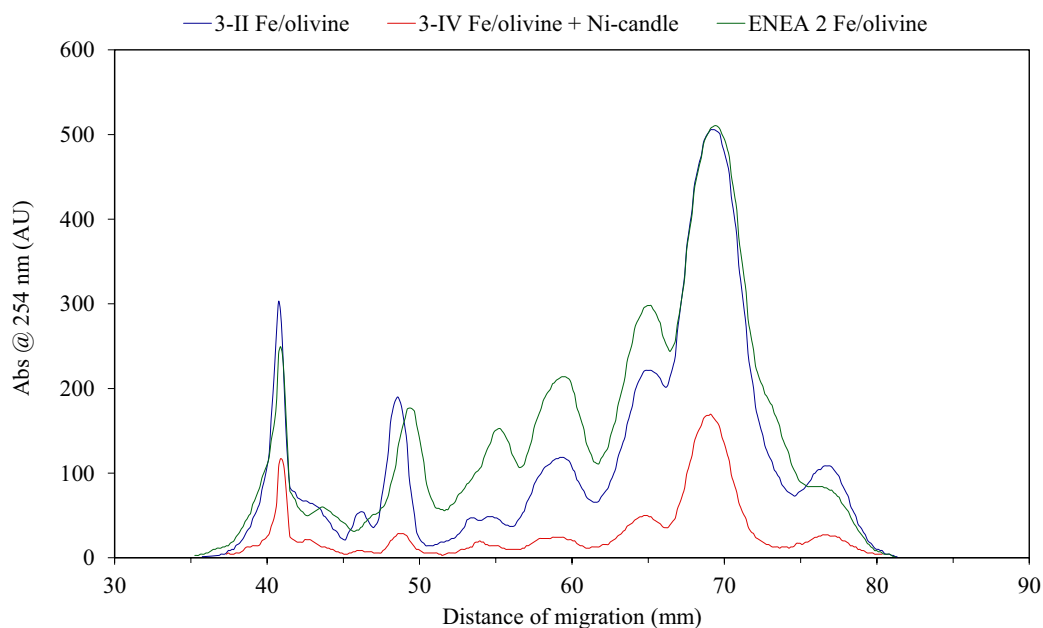
Figure 22: Chromatograms of sample 3-II (Fe/olivine), 3-IV (Fe/olivine + Ni-candle) and sample 2 from ENEA on HPLTC Silica gel 60 RP-18 with concentrating zone plate (migration at -23^{\circ}\text{C} ), recorded at \lambda = 254 \text{ nm} (table 1 –j)
