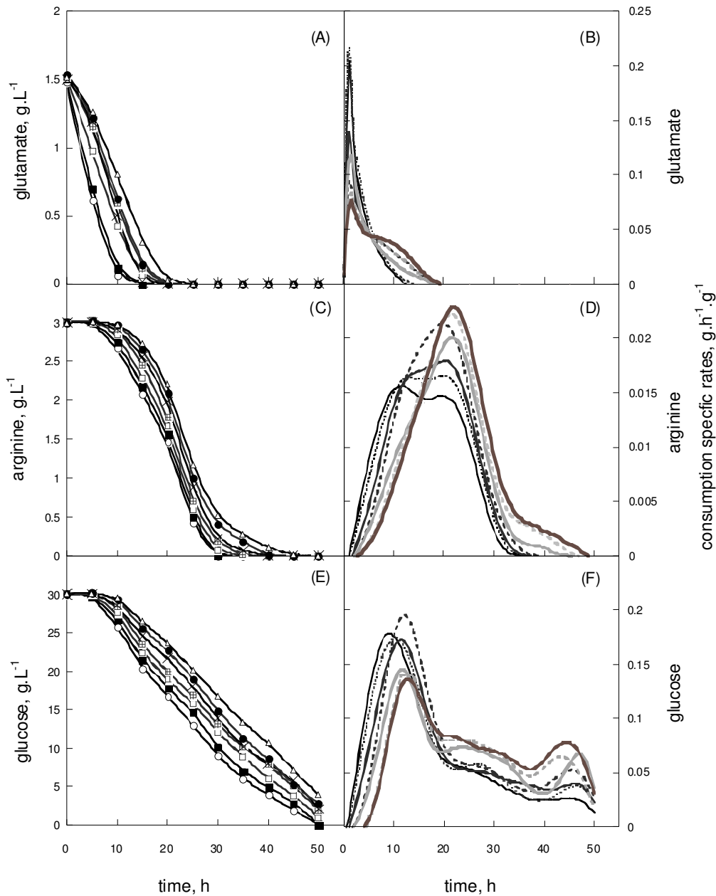
Figure III-3. I. Kinetics of carbon-substrates consumption under various conditions of power dissipation for glutamate (A), arginine (C) and glucose (E). Values of P / V ( \text{kW.m}^{-3} ) and k_{LA} ( \text{h}^{-1} ) were respectively: (6.1; 244, ○), (3.3; 137, ■), (2.2; 98, □), (1.6; 77, ⊕), (0.8; 66, ×), (0.65; 52, ●), (0.55; 43, △). II. Specific consumption rates for glutamate (B), arginine (D) and glucose (F). Values of P / V ( \text{kW.m}^{-3} ) and k_{LA} ( \text{h}^{-1} ) were respectively: (6.1; 244, —), (3.3; 137, ----), (2.2; 98, ———), (1.6; 77, ······), (0.8; 66, ———), (0.65; 52, ······), (0.55; 43, ———).
