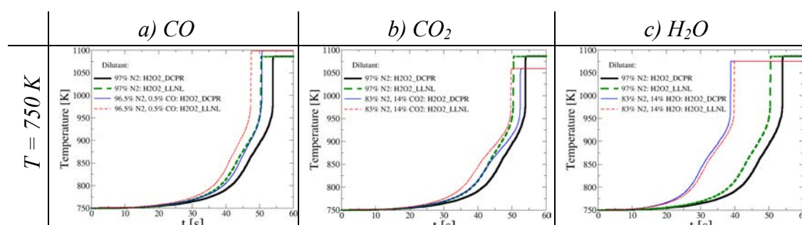
Figure 5-11 Temperature evolutions during stoichiometric hydrocarbon oxidation for the Reference-case and the cases of partial-dilution by a) CO, b) CO 2 and c) H 2 O computed with the reaction kinetics of H 2 O 2 dissociation applied by Naik et al. 2005 (LLNL) and in the presented reaction mechanism (DCPR).
