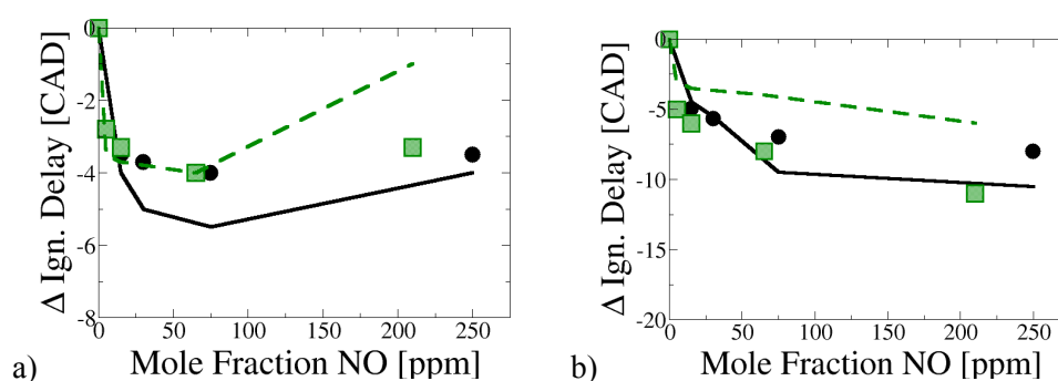
Figure 4-4 Experimental (symbols) and simulated (lines) sensitivity to NO addition of (a) cool flame and (b) main flame in [CAD] obtained in an HCCI-engine (Risberg et al. 2006) for the oxidation of Fuel_Ris_1 (black circles • and thick full line), Fuel_Ris_2 (green squares □ and dotted lines ---).
