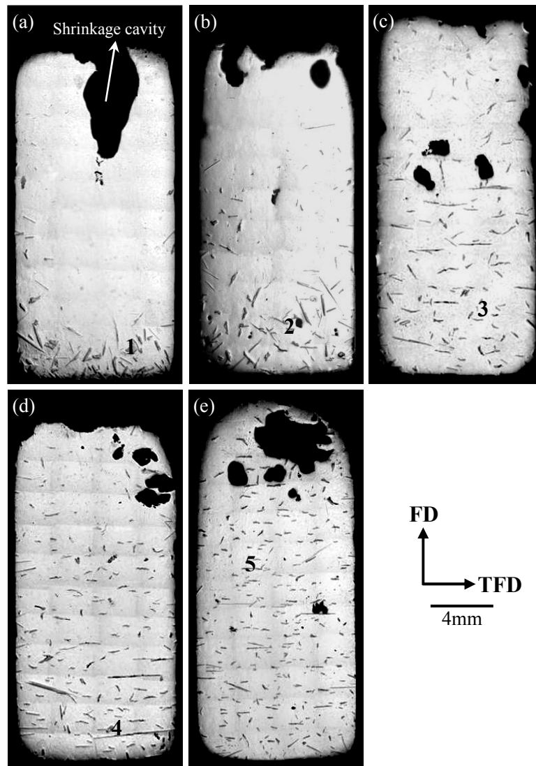
Figure 3.3 Macrostructures in the longitudinal sections of the specimens with B = (a) 0, (b) 2, (c) 5, (d) 8, (e) 12 Tesla (cooling rate: 10\text{ }^{\circ}\text{C}/\text{min} ; position: uniform magnetic field zone Z_0 ). FD and TFD denote the magnetic field direction and the transverse magnetic field direction, respectively.
