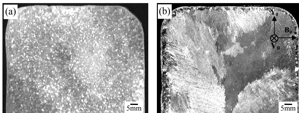
Figure 4.3 Macrostructures in the cross sections (to the casting direction V_0 ) of the slices cast without (a) and with (b) a 0.2-Tesla DC magnetic field.
