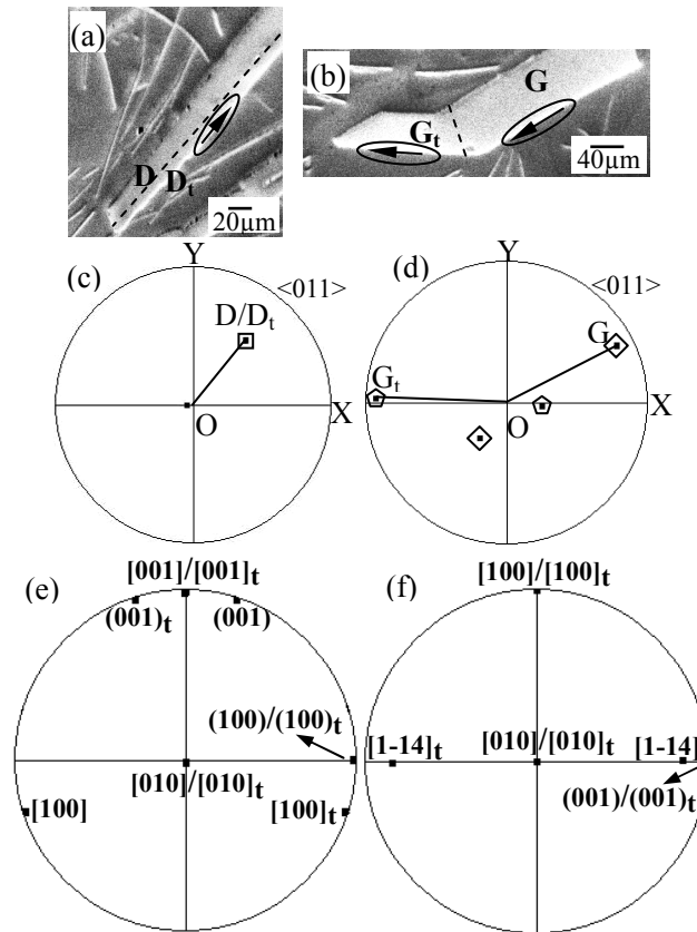
Figure 2.3 SEM images of two twinned primary Al 3 Fe crystals extending along \langle 011 \rangle but with a (a) straight and (b) bent morphology; \langle 011 \rangle stereographic projections on the observation plane corresponding to (c) D and D t and (d) G and G t ; standard stereographic projections of the twinning elements corresponding to (e) D and D t and (f) G and G t . The poles enclosed in the same shaped frames in (c) and (d) are from the same part of the crystal.
