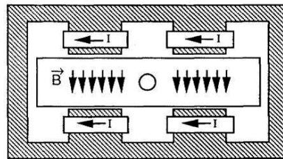
Figure 1.3 Schematic top view of the arrangement of DC magnets [16].
