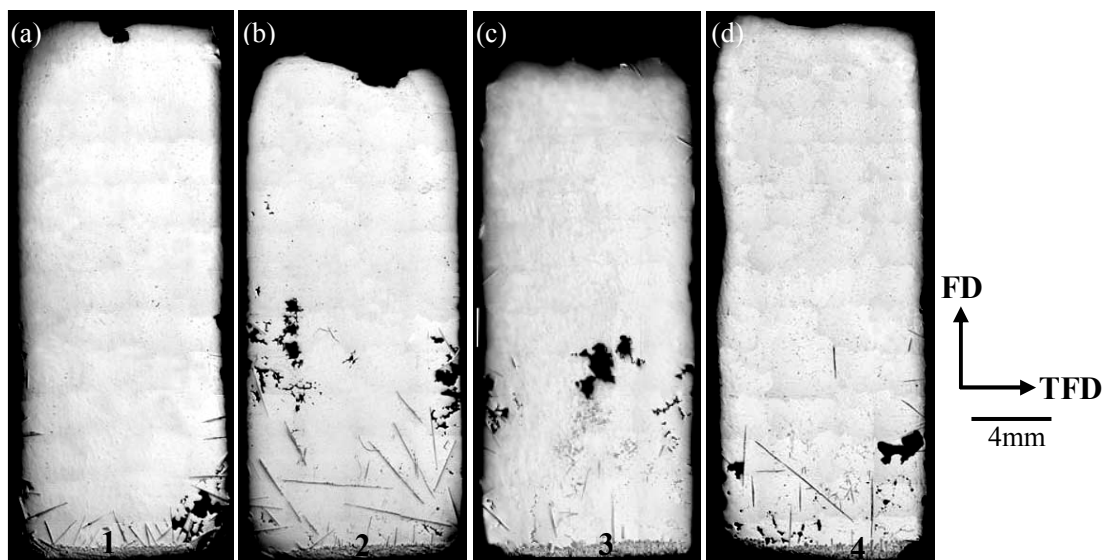
Figure 3.15 Macrostructures in the longitudinal sections of the specimens with magnetic flux densities B of (a) 0, (b) 2, (c) 5 and (d) 12 Tesla. FD and TFD denote the field direction and the transverse field direction, respectively.
