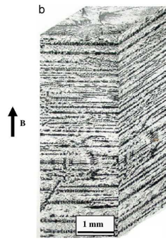
Figure 1.8 Three-dimensional macrostructure of Al-Ni alloy directionally solidified under a magnetic field of 12 Tesla [55].
