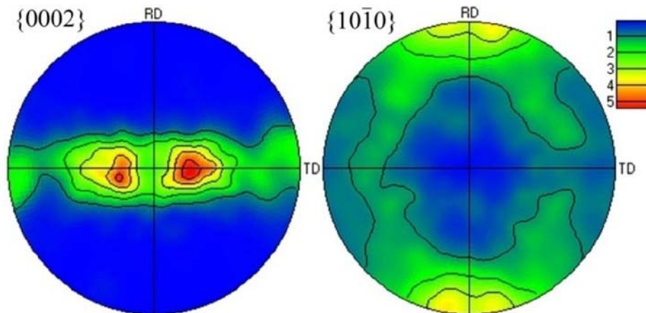
Figure. 1: The initial texture presented in the pole figures of \{0002\} and \{10\bar{1}0\} .
