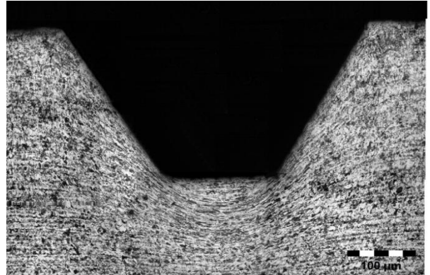
M20 - 18MnCr11 /p=36[bar]/n=1600[tours/min]
