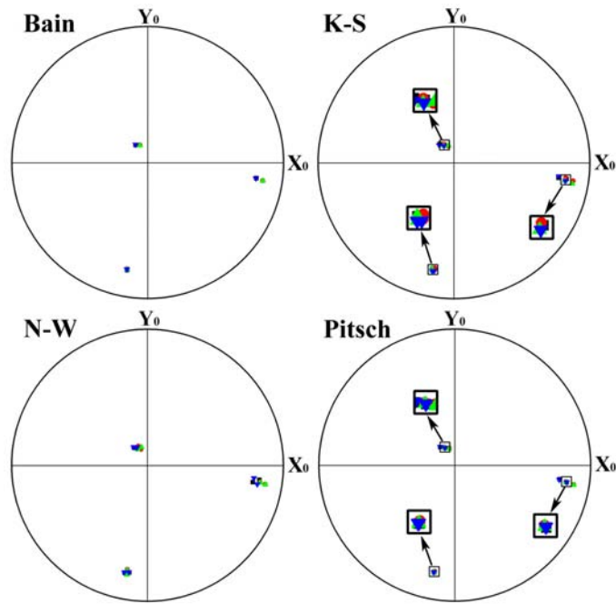
Fig. 3.6. \{001\} standard stereographic projections of austenite orientations in the macroscopic sample coordinate frame calculated from the four martensite variants in variant group gI under Bain, K-S, N-W and Pitsch relations, respectively. The common poles are enclosed in squares.
