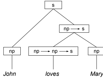
Figure 5.2: Syntactic parse tree of sentence John loves Mary .
