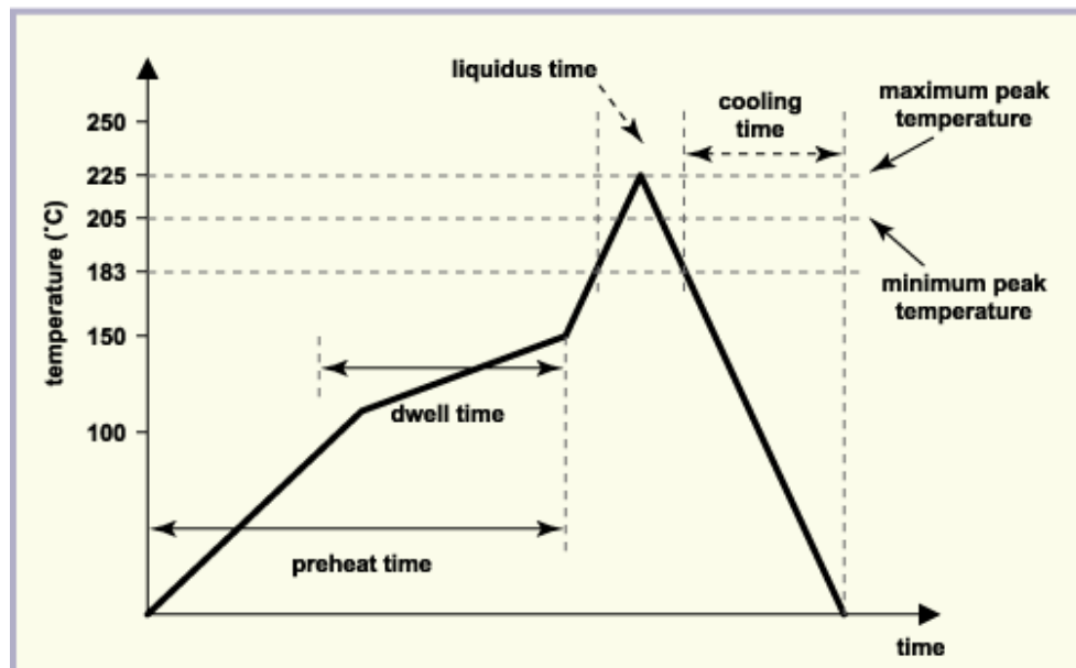
Figure 2.2: Target reflow profile for a typical RMA-style flux [Martin Tarr Reflow Soldering]
