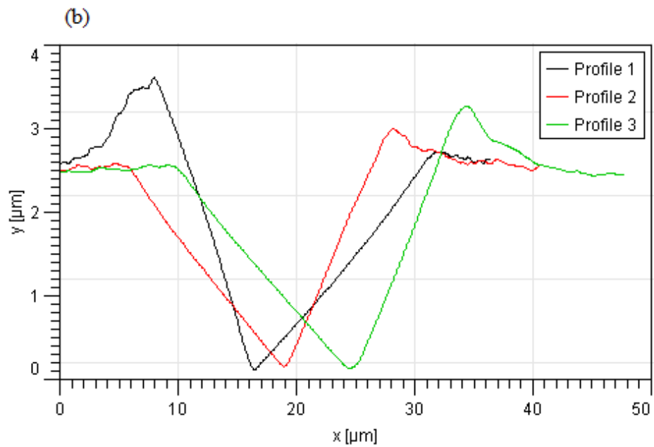
Figure 8.12: (a) Equilateral triangles and (b) Pile-up profiles
