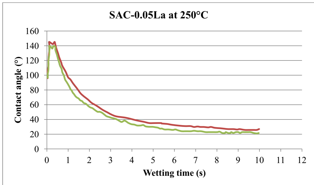
Figure 9.23: SAC-0.05La contact angle vs. wetting time at 250°C
