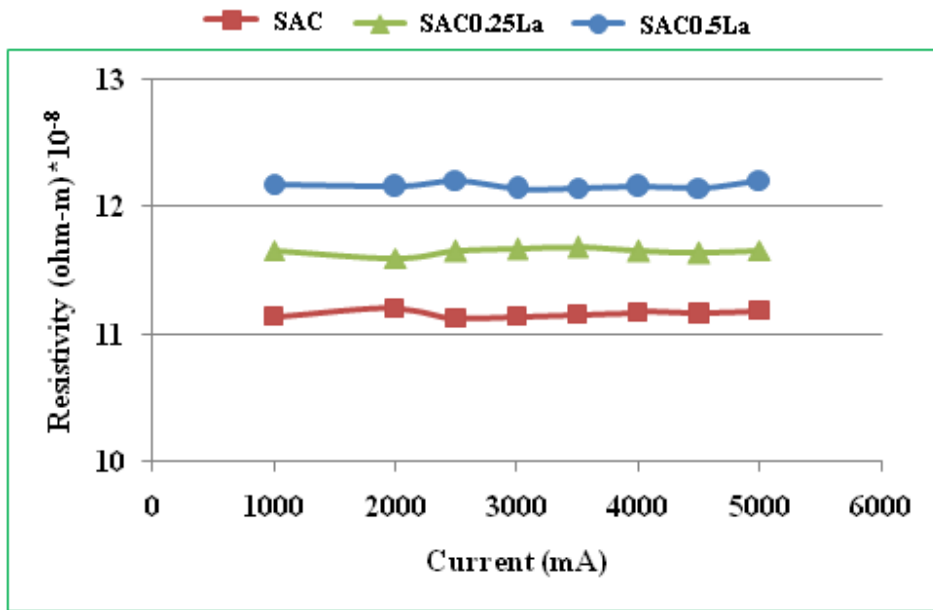
Figure E.9: Electrical resistivity after 100 hours aging at 200°C
