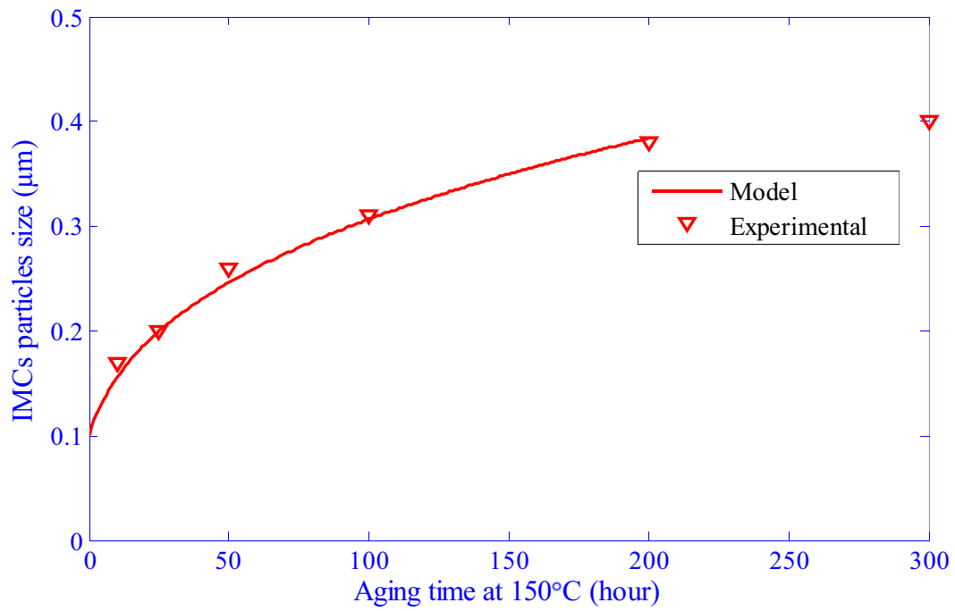
Figure 5.2: SAC-0.05La coarsening at 150°C
