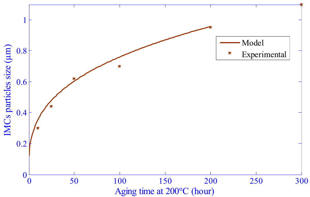
Figure 5.6: SAC coarsening at 200^\circ\text{C}
