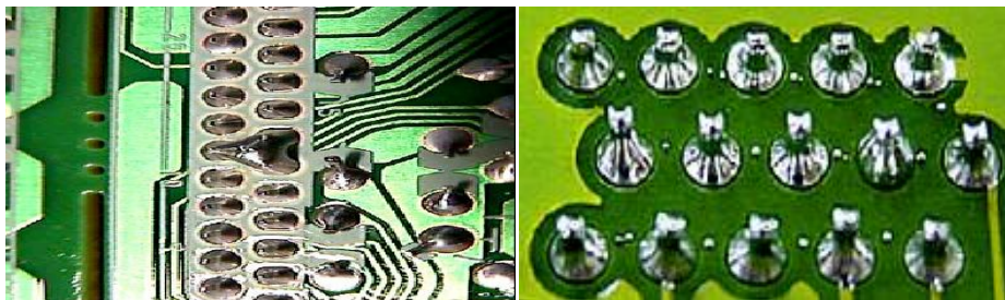
Figure 2.9: (a) too little flux and (b) too much flux
