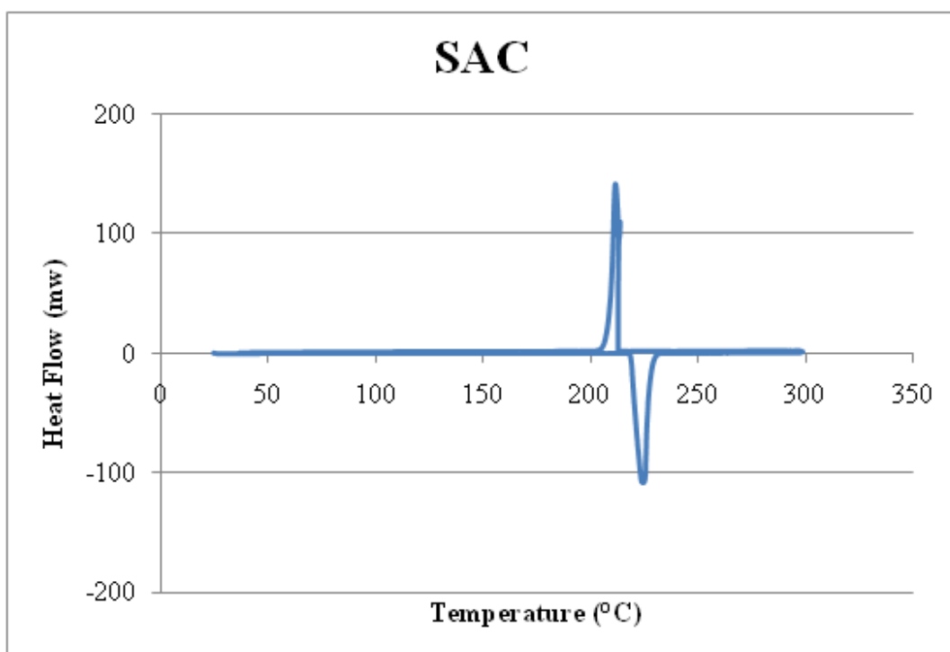
Figure C.1: SAC-0.05La DSC curve
