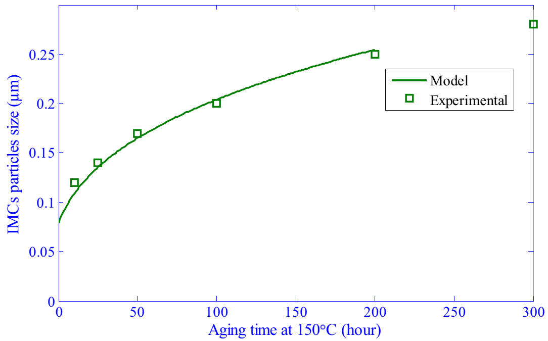
Figure 5.3: SAC-0.25La coarsening at 150°C
