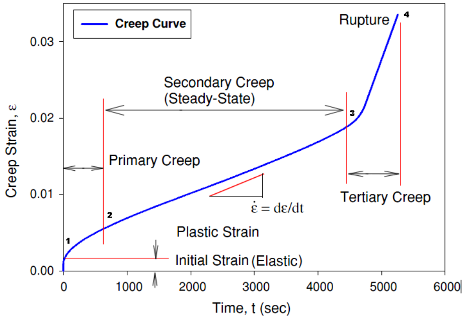
Figure 7.2: Typical creep zones [Zhang 2010]
