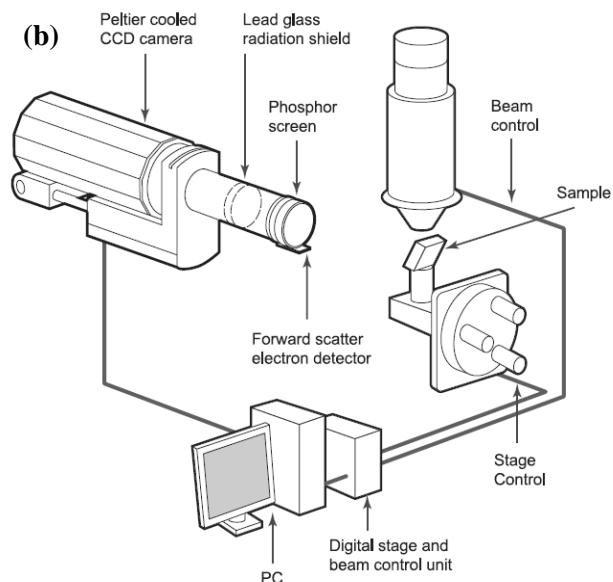
Figure 2.6 Photo (a) and schema (b) of the field emission gun SEM- Jeol JSM 6500 F .
