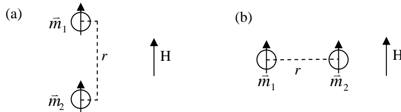
Figure 3.4 Illustration of the dipolar interaction between magnetic dipoles.
