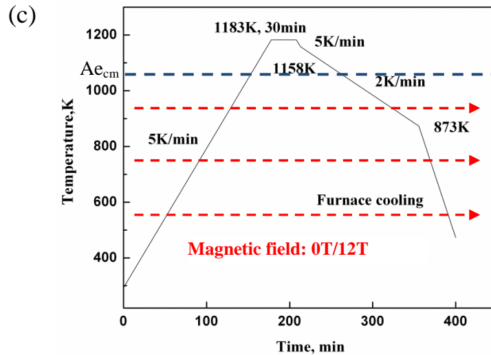
Figure 2.3 Heat treatment parameters for Fe-C alloys (a) Fe-0.12C (b) Fe-0.36C and (c) Fe-1.1 C. The respective Ae_3 and Ae_{cm} temperatures are calculated by Thermo-Calc, but the Ae_1 temperatures are from the common accepted theoretical value (1000K).
