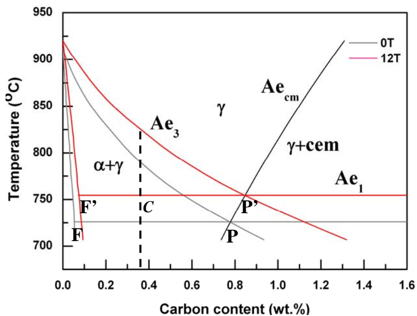
Figure 3.6 Effects of magnetic field on Fe-C phase equilibrium [49].
