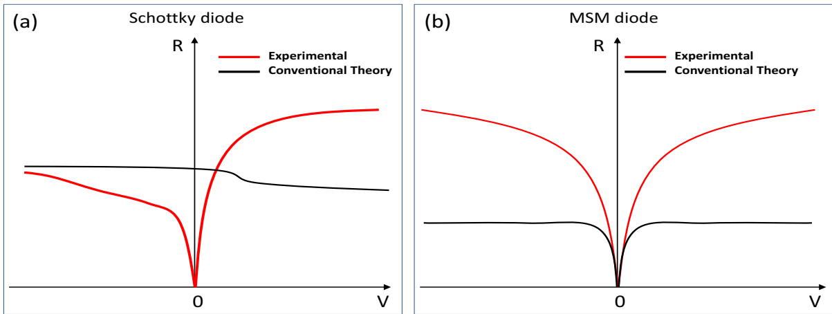
Figure 2.18: Voltage dependence of the responsivity in Schottky and MSM PDs based on the model proposed by Katz et al. [162].
