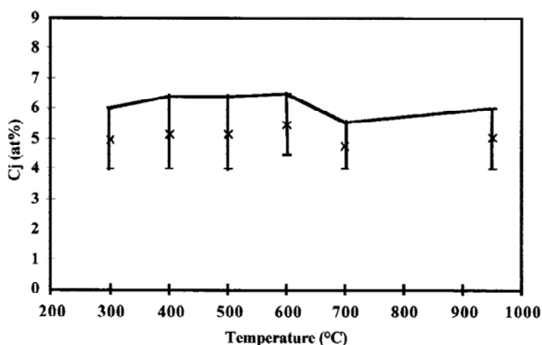
Figure.I- 15 Effect of temperature on the intergranular concentration of boron. Fe-45Al+400 appm B alloy; annealing during 24 h [63].
