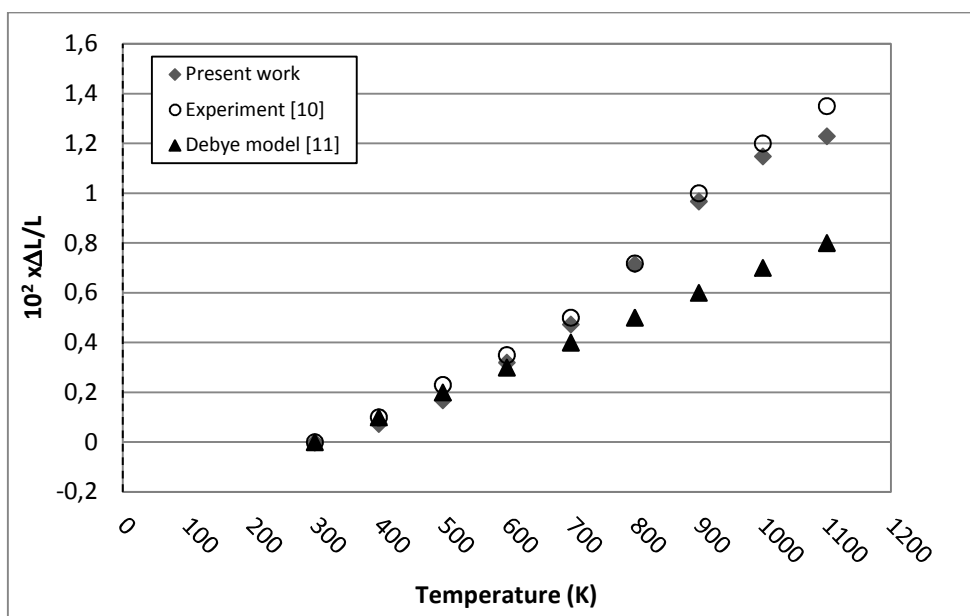
Figure. IV-7. Fractional length change data of D0_3 - Fe_3Al .
