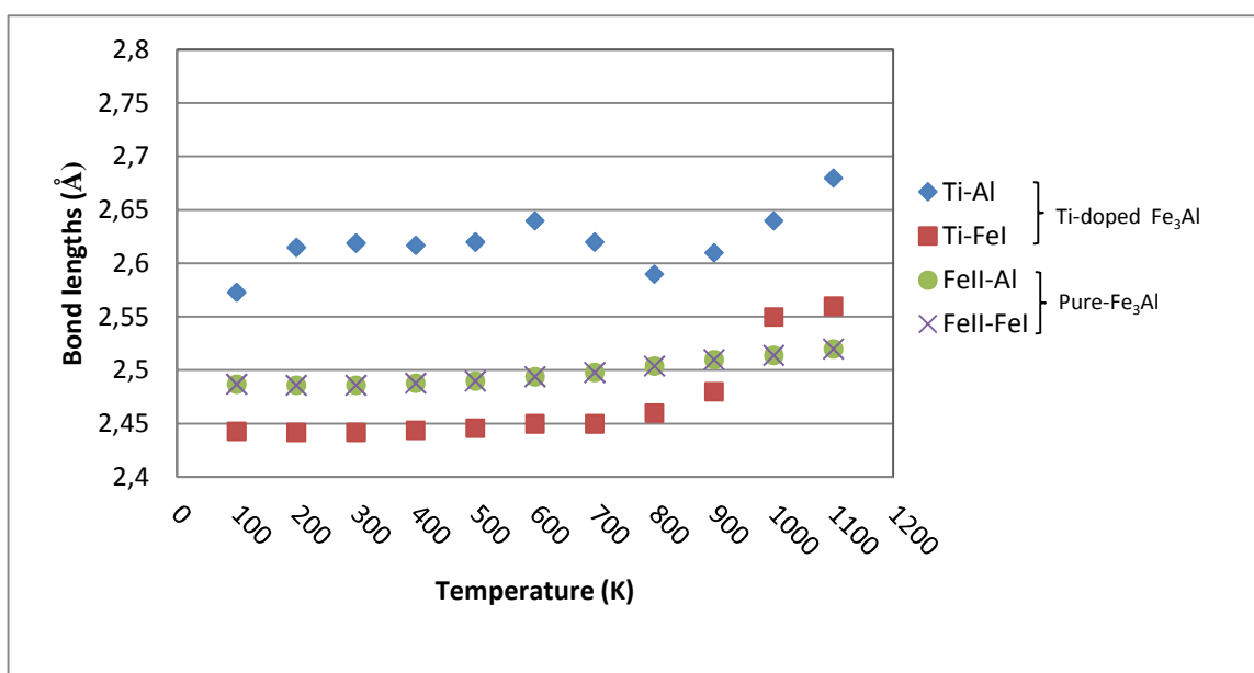
Figure. IV-3. The bond lengths in the relaxed pure and Ti-doped \text{Fe}_3\text{Al} supercells.
