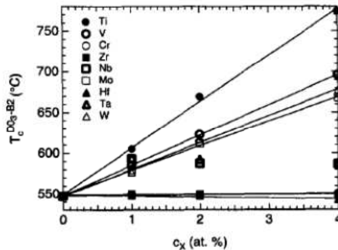
Figure.I- 9 Effect of ternary concentrations on \Delta T_0^{D03-B2} [43].
