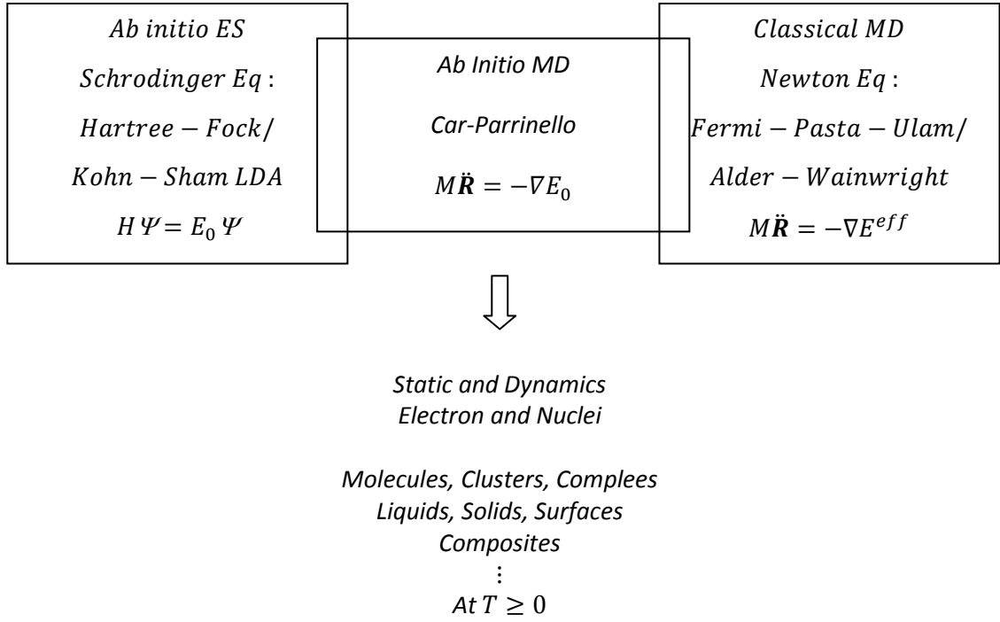
Figure. II- 1 Ab initio molecular dynamics unifies approximate ab initio electronic structure theory (i.e solving Schrodinger's wave equation numerically using, for instance, Hartree-Fock theory or the Local Density Approximation (LDA) within Kohn-Sham theory) and classical molecular dynamics (i.e solving Newton's equation of motion numerically for given interaction potential as reported by Fermi, Pasta, Ulam, and Tsingou for one-dimensional anharmonic chain model of solids and published by Alder and Wainwright for the three-dimensional hard-sphere model of fluids [5]).
