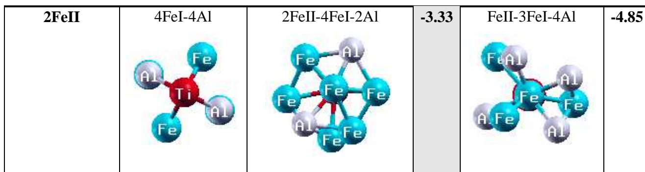
Figure.IV-23. Snapshots of the structural environment of the impurities before and after relaxation in the \Sigma 5 (310)[001] grain boundary.
