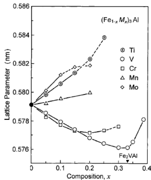
Figure.I- 13 Lattice parameters of the D0_3 phase in (Fe_{1-x}M_x)_3Al as a function of composition x for M=Ti, V, Cr, Mn and Mo . The D0_3 single-phase state is obtained in the range shown by the solid lines [41].
