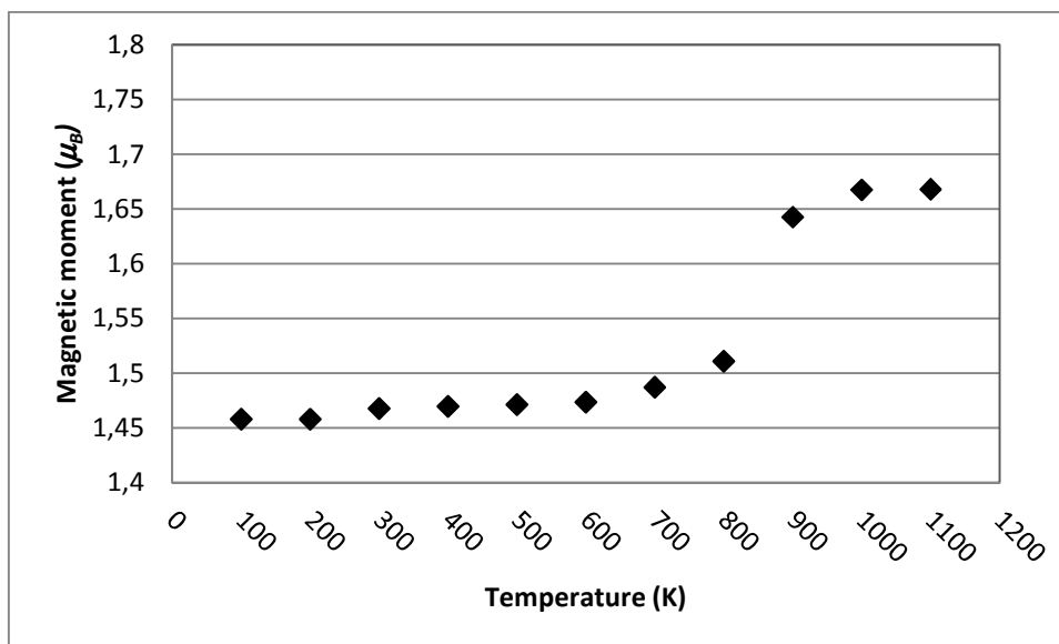
Figure. IV-6. the temperature dependence of the total magnetic moment in the D0_3 - Fe_3Al .
