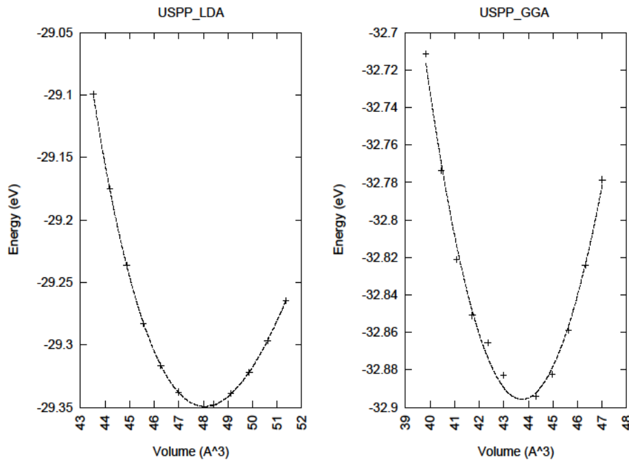
Figure. III- 1 The total energy within LDA and GGA according to the pseudopotential calculations.
