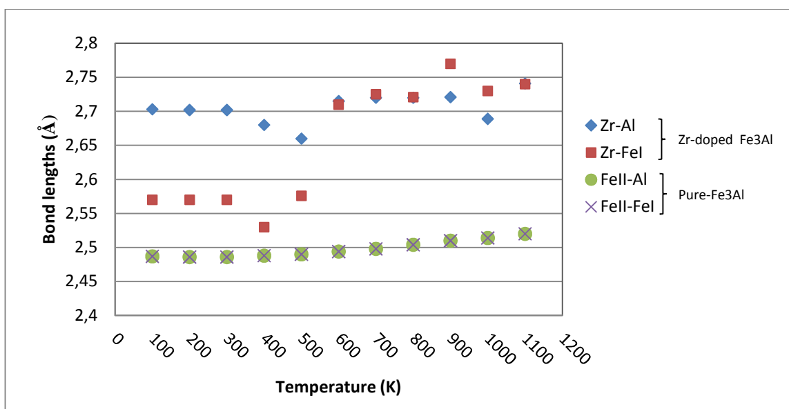
Figure. IV-4. The bond lengths in the relaxed pure and Zr-doped \text{Fe}_3\text{Al} supercells.
