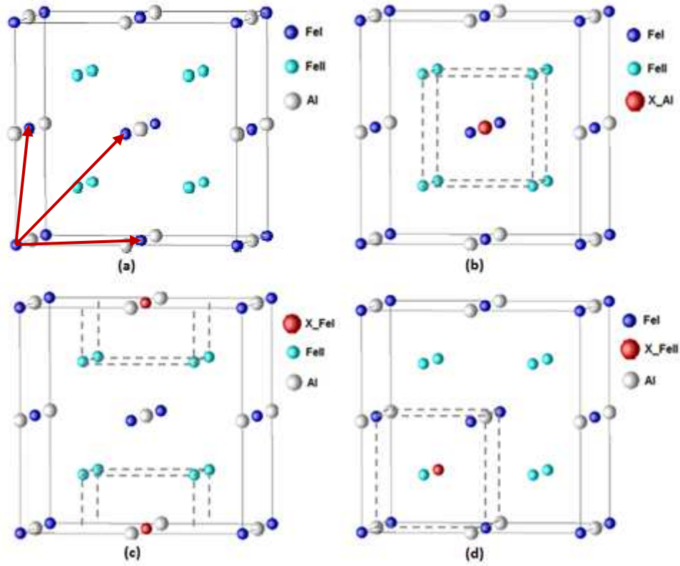
Figure. III- 2 (a) The un-doped structure of the bulk \text{Fe}_3\text{Al} and the three point defects substitutions as well as vacancies on (b) the Al site (c) the FeI site and (d) the FeII site.
