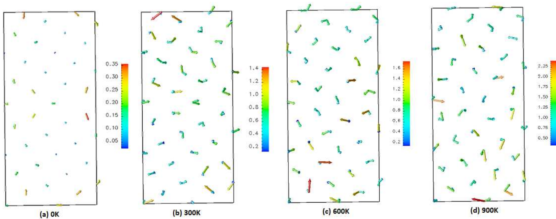
Figure.IV-20. The displacement of the atoms from in the relaxed grain boundary supercell from their initial positions (a) at 0K (b) at 300K (c) at 600K and (d) at 900K.
