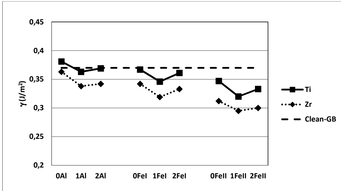
Figure. III- 7 Interface energies (in \text{J/m}^2 ) for impurity-doped grain boundaries and the clean-grain boundary.
