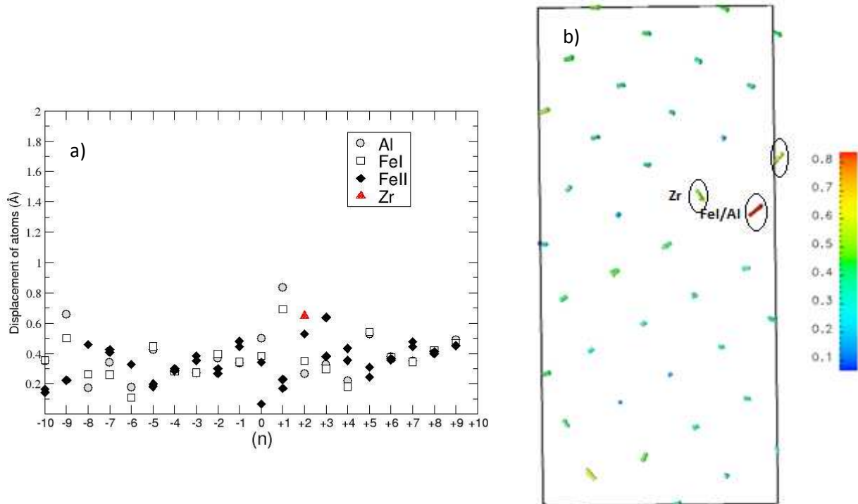
Figure. III- 20 (a) The displacement of the atoms in the relaxed supercell with Zr substitutions on the 2FeII site as function of the positions of the planes parallel to the grain boundary interface. These displacements are represented with solid arrows in (b).
