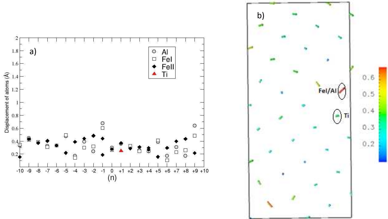
Figure. III- 17 (a) The displacement of the atoms in the relaxed supercell with Ti substitutions on the 1FeI site as function of the positions of the planes parallel to the grain boundary interface. These displacements are represented with solid arrows in (b).
