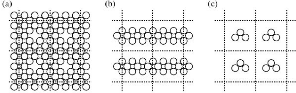
Figure. II-2. Schematic illustration of a supercell geometry (a) for a vacancy in a bulk crystalline solid, (b) surface, and (c) for a isolated molecule. The boundaries of the supercells are shown by dashed lines.
