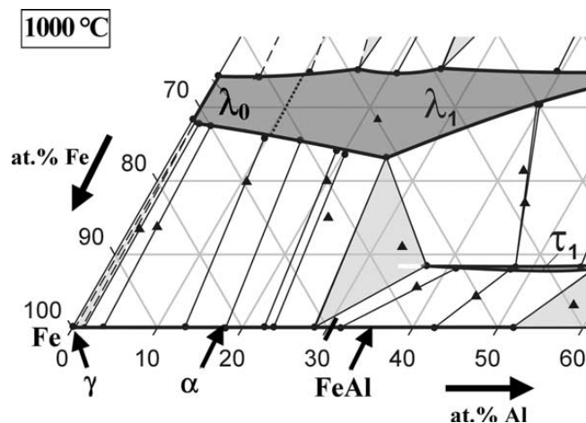
Figure.I- 4 Partial isothermal section of the Fe–Al–Zr system at 1000 °C [21]. The two ternary compounds, which are in equilibrium with the Fe–Al phases, are either a Laves phase ( \lambda , with \lambda_0 denoting the cubic C15 structure and \lambda_1 denoting the hexagonal C14 structure) or the tetragonal \text{ThMn}_{12} - type phase (\text{Fe,Al})_{12}\text{Zr} ( \tau_1 ).
