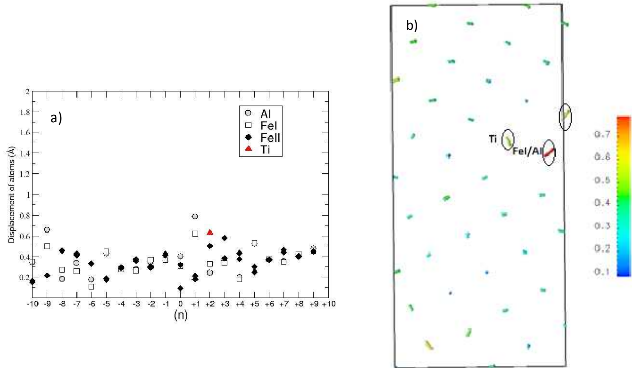
Figure. III- 19 (a) The displacement of the atoms in the relaxed supercell with Ti substitutions on the 2FeII site as function of the positions of the planes parallel to the grain boundary interface. These displacements are represented with solid arrows in (b).
