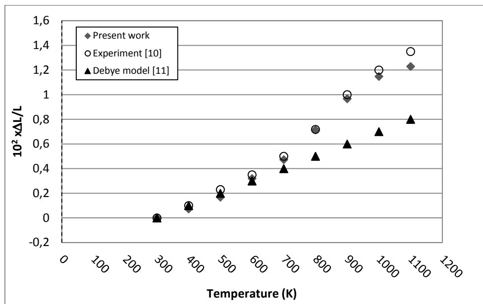
Figure. IV-7. Fractional length change data of D0_3\text{-Fe}_3\text{Al} .
