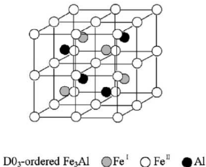
Figure.I- 10 The unit cell of D0 3 ordered Fe 3 Al.
