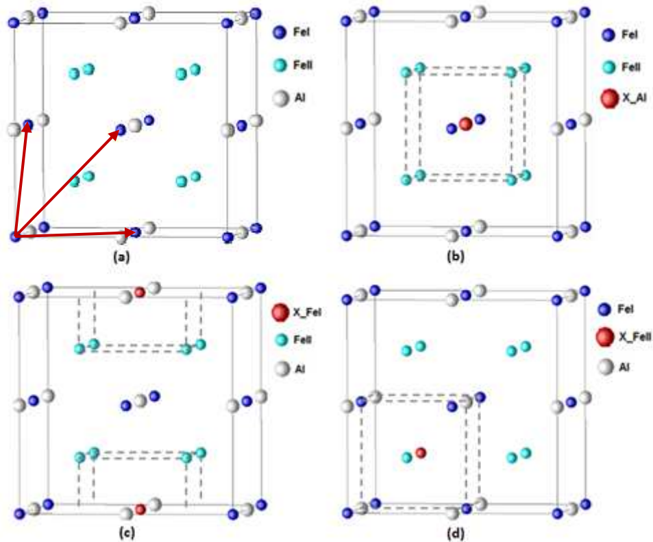
Figure. III- 2 (a) The un-doped structure of the bulk Fe 3 Al and the three point defects substitutions as well as vacancies on (b) the Al site (c) the FeI site and (d) the FeII site.
