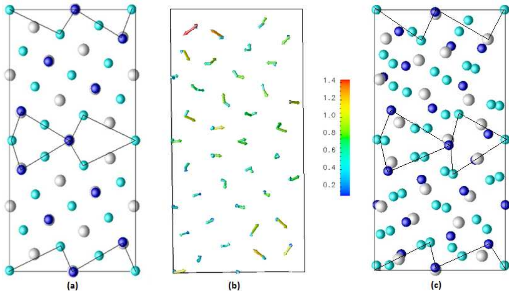
Figure. IV-22. (a) The initial positions of the relaxed grain boundary at 0K (b) the displacement of the atoms from the initial positions in the relaxed grain boundary at 300K and (c) the final positions of the atoms in the relaxed grain boundary at 300K.
