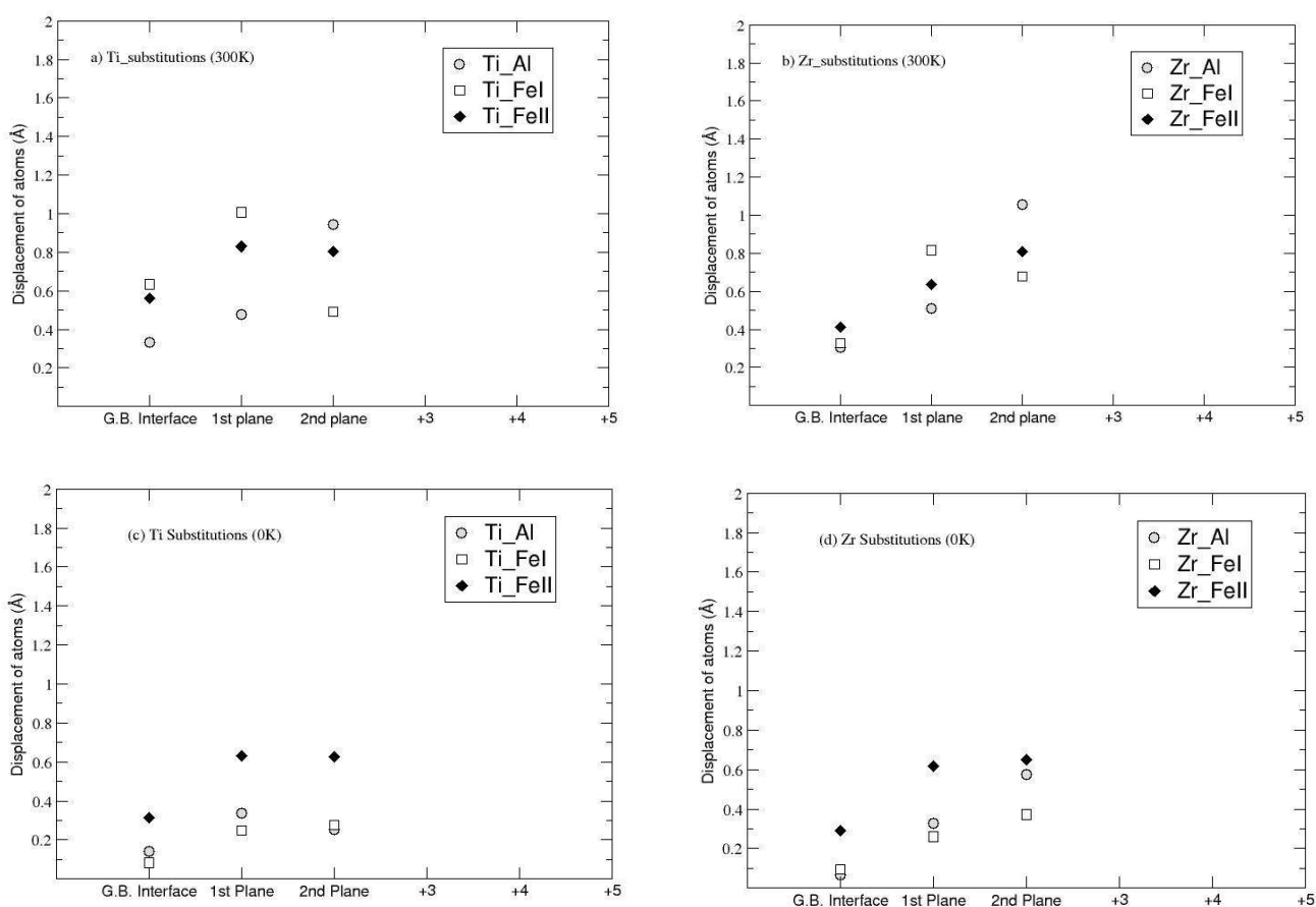
Figure. IV-23. The displacements of the impurities (a) Ti (b) Zr at 300K, (c) Ti and (d) Zr at 0K on different substitutional configurations.
