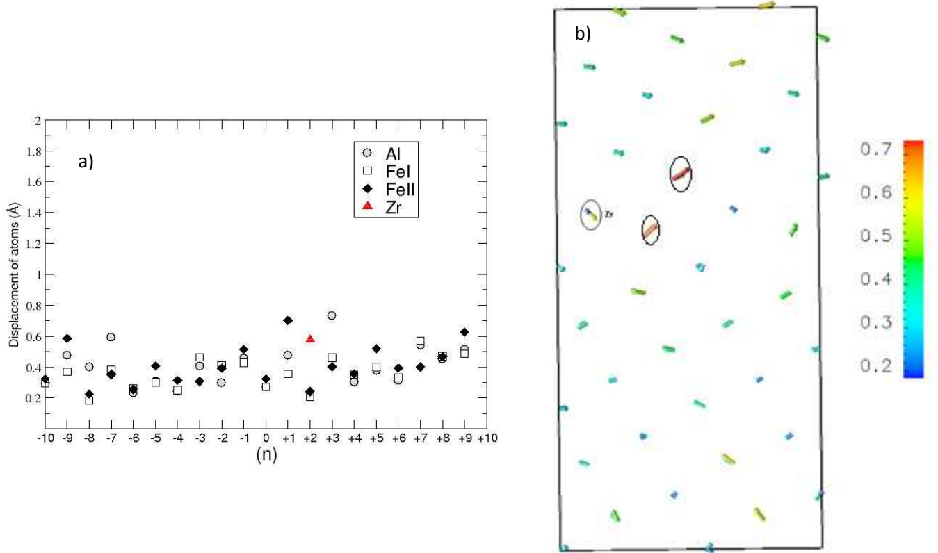
Figure. III- 13 (a) The displacements of the atoms in the relaxed supercell with solid arrows for the case of Zr substitution on the 2Al site. These displacements are represented with solid arrows in (b).
