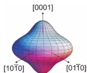
Figure.I- 5 Quantum-mechanically calculated directional dependence of single-crystalline Young's modulus of \text{Fe}_2\text{Nb} with the hexagonal C14 structure. Shape deviations from an ideal sphere identify elastic anisotropy of the studied Laves phase compound.
