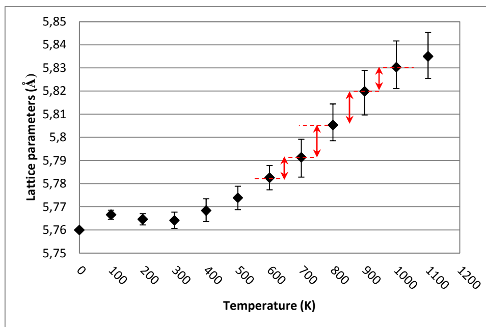
Figure. IV-5. The calculated lattice parameters at different temperatures for pure D0_3 - Fe_3Al . The error bars represent the statistical uncertainty.
