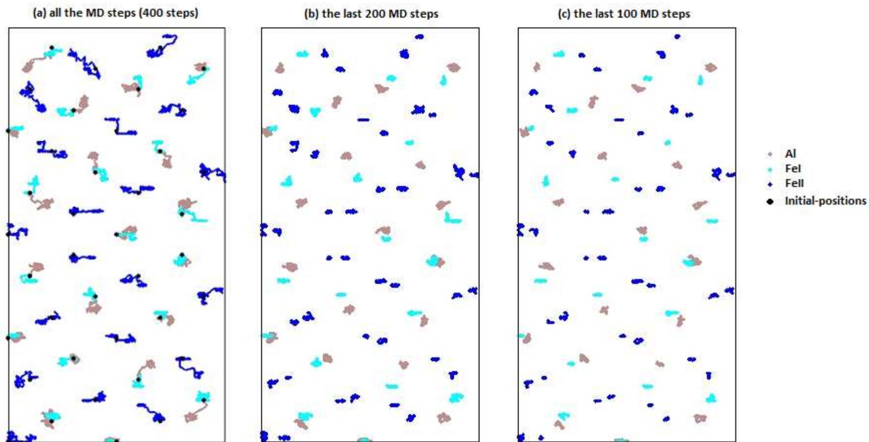
Figure.IV-19. The atomic positions in pure grain boundary \Sigma 5 (310) for (a) 400 MD steps (b) the last 200 MD steps and (c) the last 100 MD steps.
