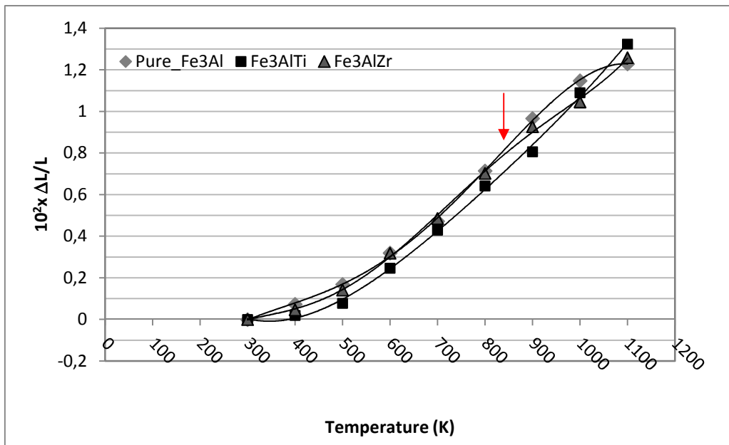
Figure. IV-9. Fractional length change data of \text{D0}_3\text{-Fe}_3\text{Al} , Ti-doped \text{Fe}_3\text{Al} and Zr-doped \text{Fe}_3\text{Al} (Ti and Zr are placed on the FeI site).
