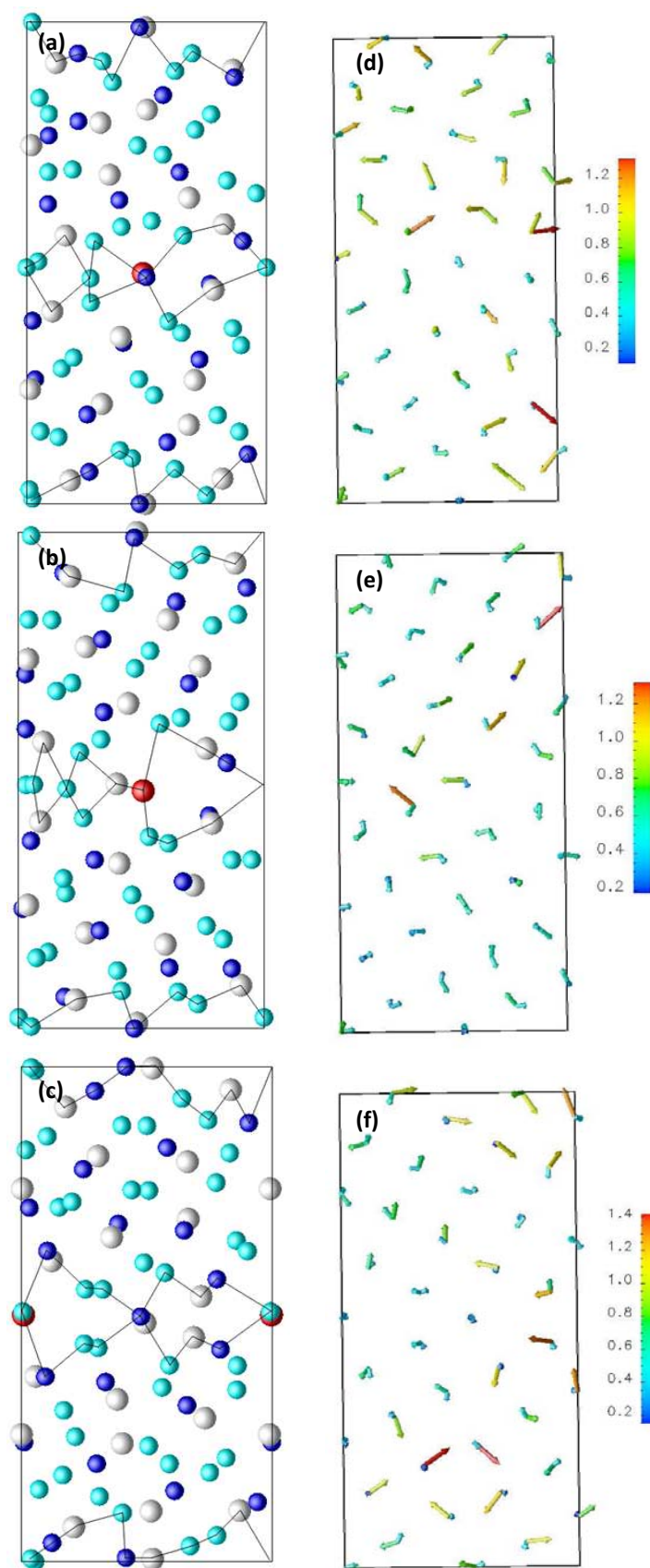
Figure. V-25. The left plots (a), (b) and (c) are the relaxed grain boundary geometries with Zr substitution on the most stable configurations 0Al, 1FeI and 2FeII, respectively. The right plots (d), (e) and (f) the displacement of each atom in the grain boundaries represented in (a), (b) and (c) from its initial positions.
