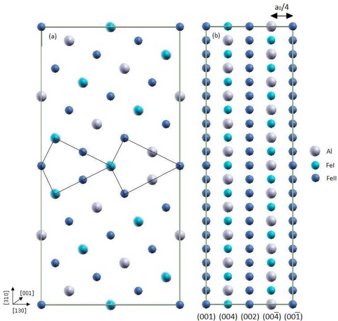
Figure. III- 4 Atomic structure of the \text{Fe}_3\text{Al} \Sigma 5 (310) [001] grain boundary (a) viewed along the [001] direction (b) viewed along the (130) direction.
