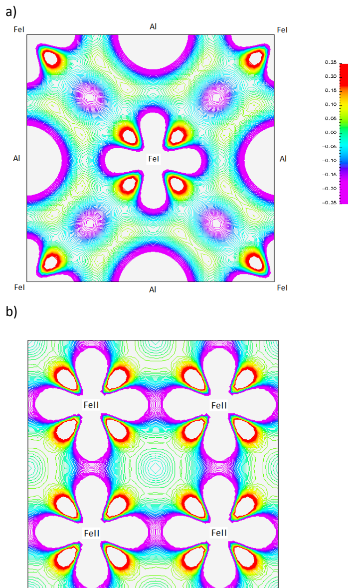
Figure. III- 8 Difference charge density of bulk \text{Fe}_3\text{Al} on (a) the (004) FeI/Al mixed plane and (b) the (001) pure FeII plane. Positive (negative) contours represent contours of increased (decreased) charge density. Contours start from \pm 0.25 e/(\text{\AA})^3 and increase successively by a factor of root 0.008.
