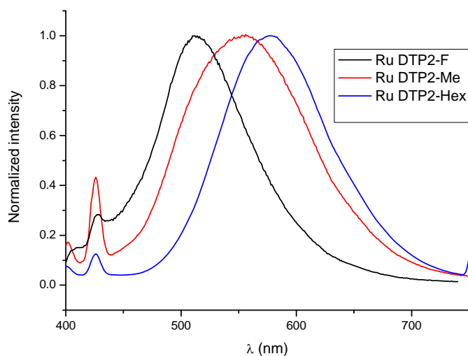
Figure 6.5: Emission spectra of the \text{Ru-DTP}_2 series upon 380 nm excitation. No emission was observed by direct excitation of the low energy band \lambda > 480 nm)
