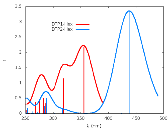
Figure 5.13: Computed spectra of bpy(DTP 1 -Hex) and bpy(DTP 2 -Hex) .
