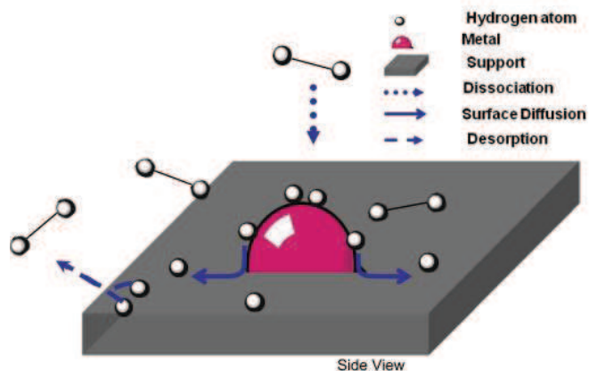
Figure 29 Hydrogen spillover processes [150~156]
