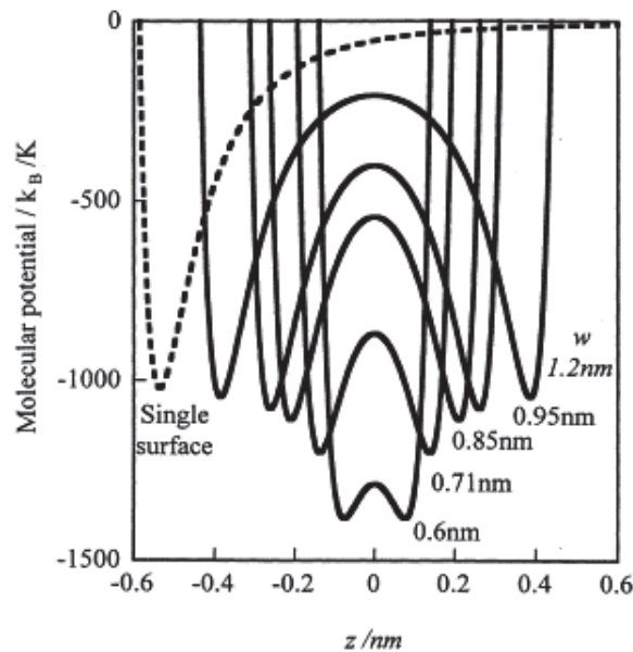
Figure 24 Overlapping of adsorption forces from the opposite walls of the micropores (from [176]).
