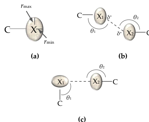
Figure II.2 (a) Anisotropic distribution of \rho(\mathbf{r}) around halogen atom (X), showing different atomic radii ( r_{\min}/r_{\max} ) along polar and equatorial directions (b) Type-I interaction ( \theta_1 \approx \theta_2 ); (c) Type-II interaction ( \theta_1 \approx 90^\circ , \theta_2 \approx 180^\circ ). 61
