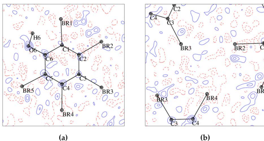
Figure III.5 Residual electron density maps for the experimental model of C 6 Br 5 OH drawn (a) in the plane of the molecule and (b) in the plane of the Br 3 -synthon. Contours are at \pm 0.05 \text{ eÅ}^{-3} level: full lines in blue – positive, dotted lines in red – negative. Resolution range is 0 \leq (\sin \theta/\lambda) \leq 0.9 \text{ Å}^{-1} .
