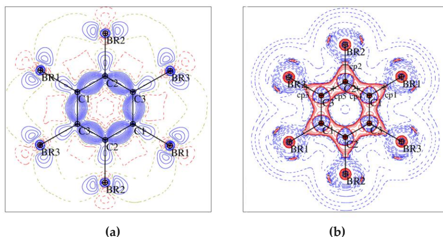
Figure III.3 (a) Static deformation density \Delta\rho(\mathbf{r}) and (b) negative Laplacian L(\mathbf{r}) maps for the theoretical multipolar model of C_6Br_6 drawn in the plane of the molecule. \Delta\rho(\mathbf{r}) contours are at \pm 0.05 \text{ e}\text{\AA}^{-3} level: full lines in blue – positive, dotted lines in red – negative. L(\mathbf{r}) contours ( \text{e}\text{\AA}^{-5} ) are in logarithmic scale, red – positive, blue – negative.
