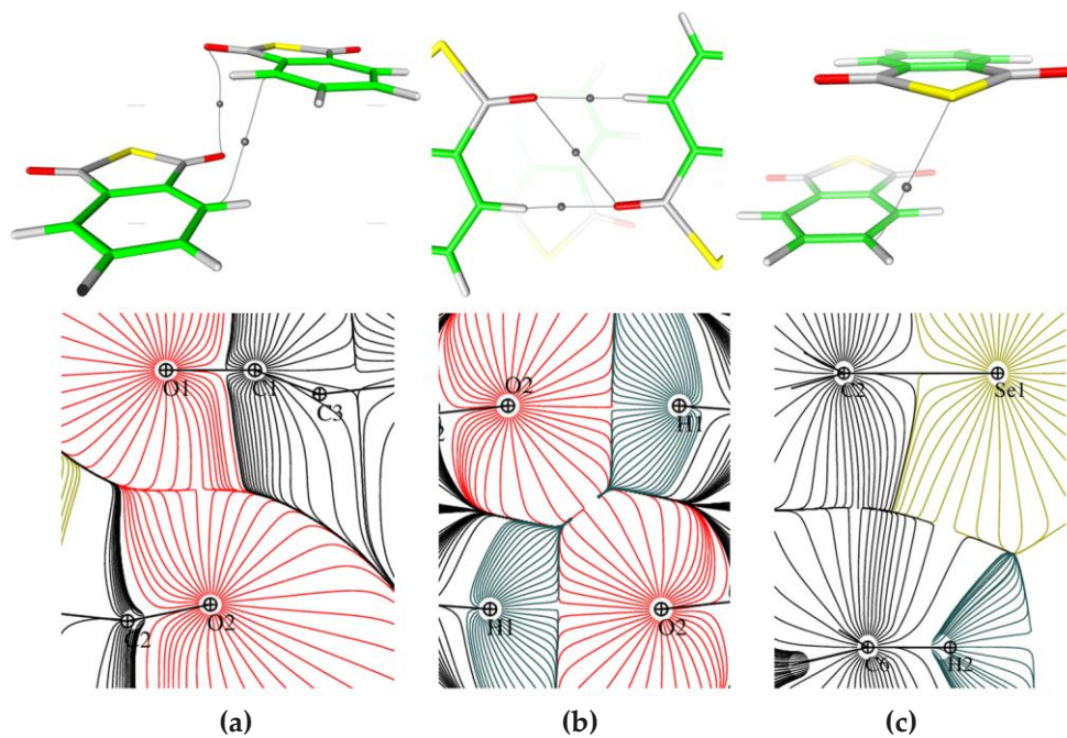
Figure V.10 Intermolecular interactions involving O- and Se-atoms in the crystal structure \text{CsO}_2\text{H}_4\text{Se} (experimental model), represented by the bond paths and the corresponding BCP's between the interacting atoms (top) and by the gradient \nabla\rho(\mathbf{r}) maps (bottom): (a) \text{O}_2\cdots\text{O}_1 , (b) \text{O}_2\cdots\text{O}_2 , (c) \text{Se}\cdots\text{C}_6 .
