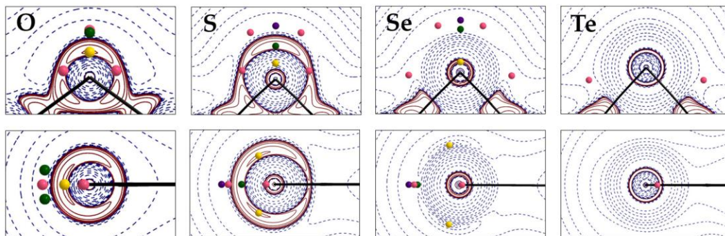
Figure V.3 Laplacian L(\mathbf{r}) = -\nabla^2\rho(\mathbf{r}) maps around chalcogen atoms in \text{C}_s\text{O}_2\text{H}_4\text{Chal} monomers (C-Chal-C plane (top) and perpendicular plane bisecting the \alpha(\text{C-Chal-C}) angle (bottom), obtained from gas-phase calculations. L(\mathbf{r}) contours ( \text{e}\text{\AA}^{-5} ) are in logarithmic scale, red – positive, blue – negative. The topology of L(\mathbf{r}) of the atomic valence shell is marked in colored circles: (3,-3) – yellow, (3,-1) – green, (3,+1) – pink, (3,+3) – violet.
