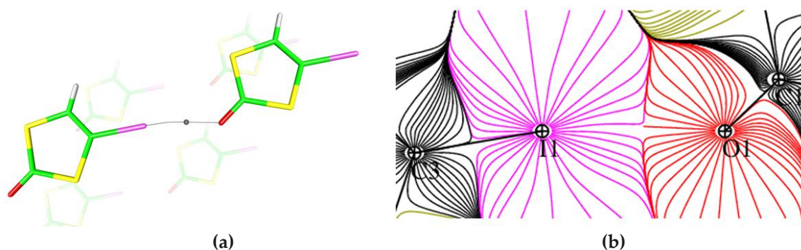
Figure IV.5 (a) Intermolecular halogen bonding interaction (I \cdots O) in the crystal structure of C 3 HIOS 2 with the corresponding bond path and BCP. (b) \nabla\rho(\mathbf{r}) map for the same interaction displaying the existence of the BCP by the zero value of \nabla\rho(\mathbf{r}) .
