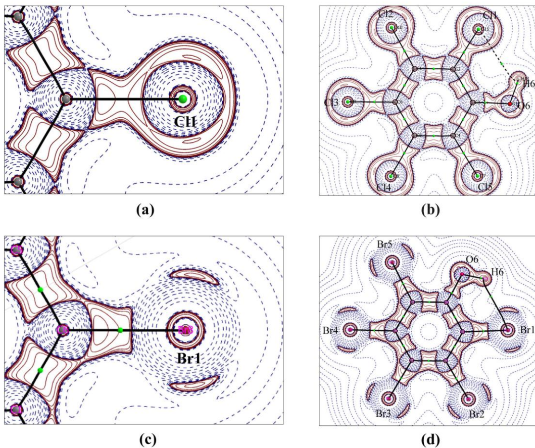
Figure 1. Contour maps of L(\mathbf{r}) drawn in the plane of the molecule obtained from the theoretical calculations performed for the isolated molecules in the gas phase for (a) C_6Cl_6 (b) C_6Cl_5OH (c) C_6Br_6 and (d) C_6Br_5OH . Contours are (in a.u.): 0, \pm 1 \cdot 10^{-3}, \pm 2 \cdot 10^n, \pm 4 \cdot 10^n, \pm 8 \cdot 10^n , with n = -3, -2, -1, 0, 1, 2 . Positive contours: red lines, negative contours: blue dashed lines.
