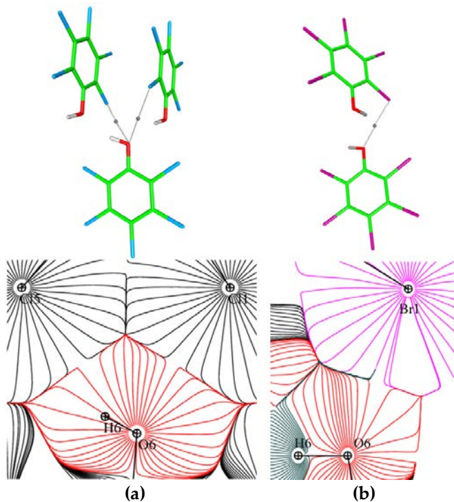
Figure V.11 Intermolecular interactions involving O-atoms in the crystal structures of (a) \text{C}_6\text{Cl}_5\text{OH} ( \text{O}_6\cdots\text{Cl}_1/\text{Cl}_5 ) and (b) \text{C}_6\text{Br}_5\text{OH} ( \text{O}_6\cdots\text{Br}_1 ), represented by the bond paths and the corresponding BCP's between the interacting atoms (top) and by the gradient \nabla\rho(\mathbf{r}) maps (bottom).
