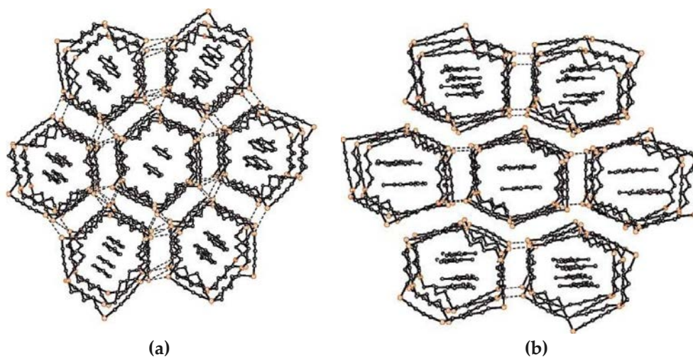
Figure II.12 Top view of columnar arrangement of (a) hexaselenacyclohexayne based self-assembling tube with inclusion of toluene and (b) mesitylene; short Se...Se interactions are indicated. 106c
