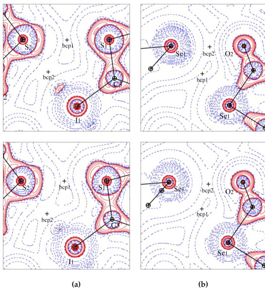
Figure V.8 Experimental (top) and theoretical (bottom) L(\mathbf{r}) = -\nabla^2\rho(\mathbf{r}) maps in the intermolecular region for (a) C 8 O 2 H 4 Se and (b) C 3 HIOS 2 . L(\mathbf{r}) contours ( \text{e}\text{\AA}^{-5} ) are in logarithmic scale, red – positive, blue – negative.. Intermolecular bcp's and CD/CC sites (see Figure V.6 for colors description), involved in the intermolecular interaction are depicted.
