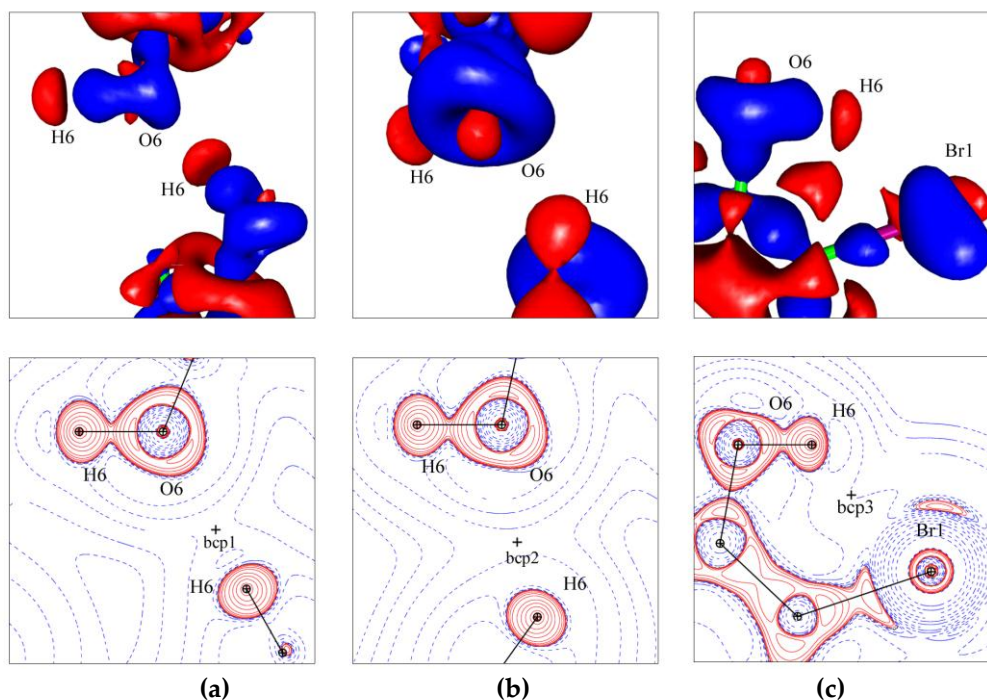
Figure VI.2 Static deformation density \Delta\rho(\mathbf{r}) (top) and L(\mathbf{r}) (bottom) maps showing the intermolecular hydrogen bonding for C_6Cl_5OH (a) and C_6Br_5OH (b), and the intramolecular hydrogen bonding for C_6Br_5OH (c). \Delta\rho(\mathbf{r}) iso-surfaces are drawn at \pm 0.05 \text{ e}\text{\AA}^{-3} : blue – positive, red – negative. L(\mathbf{r}) contours ( \text{e}\text{\AA}^{-5} ) are in logarithmic scale, red – positive, blue – negative.
