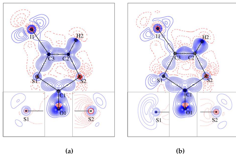
Figure III.16 Static deformation density \Delta\rho(\mathbf{r}) maps for \text{C}_3\text{HIO}_2\text{S}_2 drawn in the plane of the molecule and in the two perpendicular planes bisecting the \text{C-S-C} angles: (a) experimental and (b) theoretical models. Contours are at \pm 0.05 \text{ e}\text{\AA}^{-3} level: full lines in blue – positive, dotted lines in red – negative.
