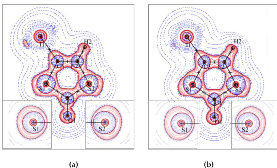
Figure III.17 L(\mathbf{r}) maps for C_3HIOS_2 drawn in the plane of the molecule and in the two perpendicular planes bisecting the C–S–C angles: (a) experimental and (b) theoretical models. Contours ( e\text{\AA}^{-5} ) are in logarithmic scale, red – positive, blue – negative.
