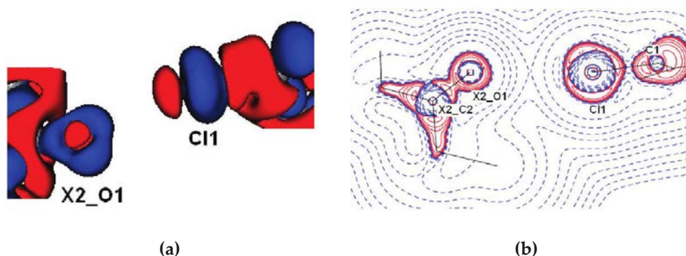
Figure II.7 (a) 3D static deformational density and (b) L(r) maps representing an electrostatically attractive Cl( \delta^+ /CD) \cdots O( \delta^- /CC) interaction. Iso-surface of \Delta\rho(\mathbf{r}) at \pm 0.05 e \text{\AA}^{-3} , blue – positive, red – negative ; L(r) contours (e \text{\AA}^{-5} ) are in logarithmic scale, red – positive, blue – negative 94
