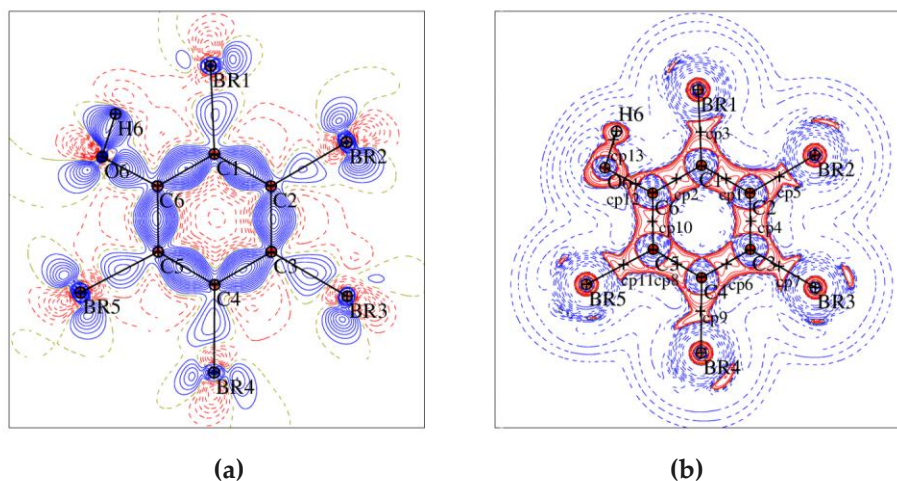
Figure III.6 (a) Static deformation density \Delta\rho(\mathbf{r}) and (b) negative Laplacian L(\mathbf{r}) maps for the experimental multipolar model of \text{C}_6\text{Br}_5\text{OH} drawn in the plane of the molecule. \Delta\rho(\mathbf{r}) contours are at \pm 0.05 \text{ e}\text{\AA}^{-3} level: full lines in blue – positive, dotted lines in red – negative. L(\mathbf{r}) contours ( \text{e}\text{\AA}^{-5} ) are in logarithmic scale, red – positive, blue – negative.
