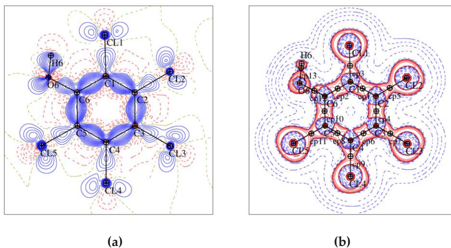
Figure III.9 (a) Static deformation density \Delta\rho(\mathbf{r}) and (b) negative Laplacian maps L(\mathbf{r}) for the experimental multipolar model of C_6Cl_5OH drawn in the plane of the molecule. \Delta\rho(\mathbf{r}) contours are at \pm 0.05 \text{ e}\text{\AA}^{-3} level: full lines in blue – positive, dotted lines in red – negative. L(\mathbf{r}) contours ( \text{e}\text{\AA}^{-5} ) are in logarithmic scale, red – positive, blue – negative.
