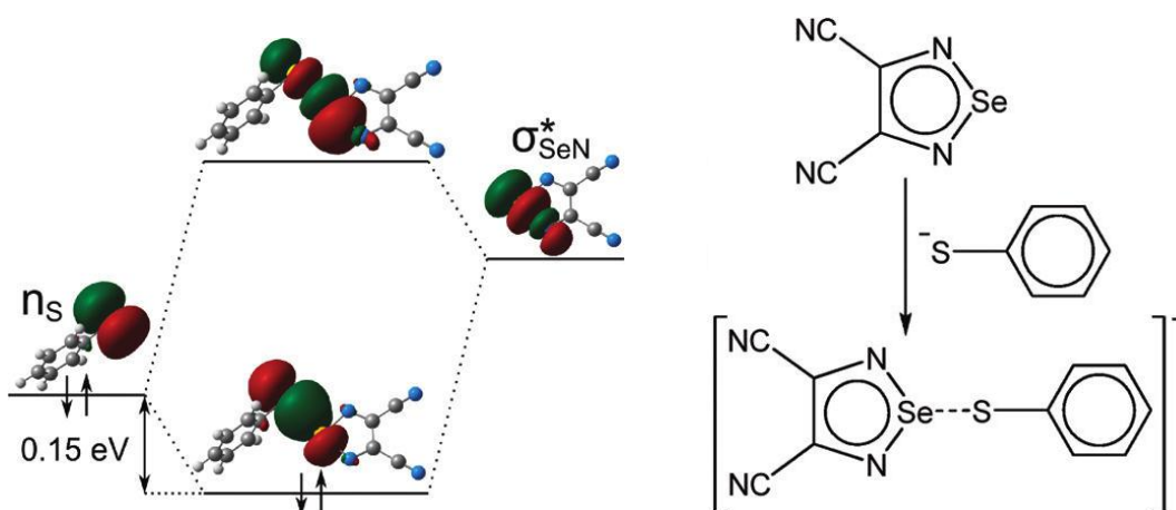
Figure II.13 NBO diagram for Se...S bond formation 113a
