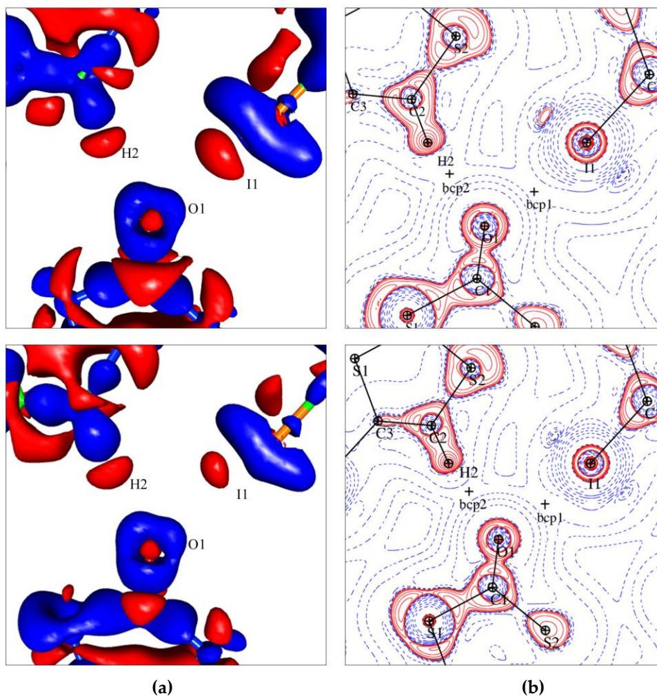
Figure VI.4 Experimental (top) and theoretical (bottom) maps in the intermolecular space of the competing halogen (O \cdots H) and hydrogen (O \cdots I) bondings in the crystal structure of C 3 HIO 5 S 2 : (a) 3D static deformation density maps \Delta\rho(\mathbf{r}) , iso-surface are drawn at \pm 0.05 \text{ e}\text{\AA}^{-3} , blue – positive, red – negative; (b) L(\mathbf{r}) maps, contours ( \text{e}\text{\AA}^{-5} ) are in logarithmic scale, red – positive, blue – negative.
