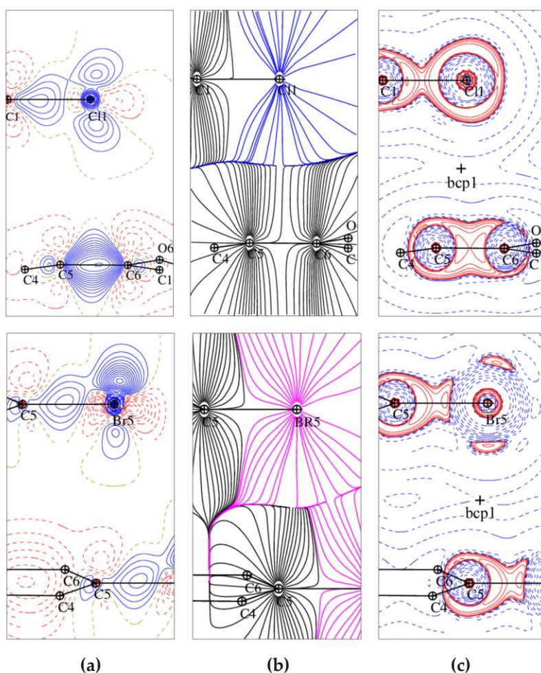
Figure IV.8 Intermolecular interactions Cl 1 ...C 5 in C 6 Cl 5 OH (top) and Br 5 ...C 5 in C 6 Br 5 OH (bottom): (a) static deformation density maps, contours are at \pm 0.05 \text{ e}\text{\AA}^{-3} , blue – positive, red – negative, (b) \nabla\rho(\mathbf{r}) map and (c) L(\mathbf{r}) maps, contours ( \text{e}\text{\AA}^{-5} ) are in logarithmic scale, red – positive, blue – negative.
