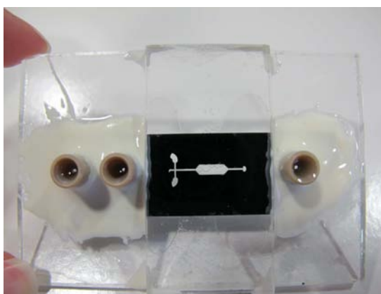
FIGURE 2.8 – Jonction flow-focusing 250 \mu\text{m}
