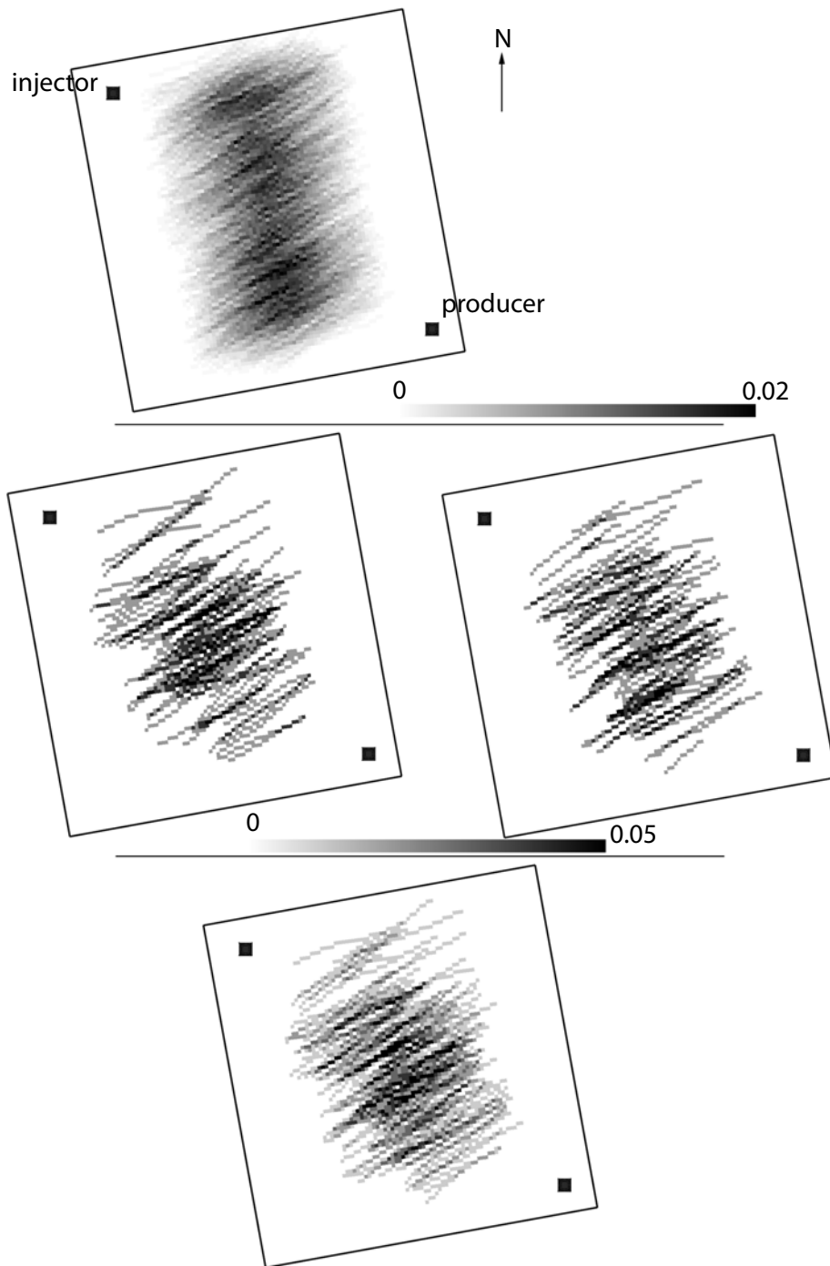
FIGURE 3.18 – Probability maps of faults belonging to family B . Top : the map obtained from the 2000 prior models. Middle : posterior models computed using the inversion scheme from the best 50 models (left) and from the 50 following models (right). Bottom : posterior probability map built from the 100 posterior models. The posterior map highlights an area on the main flow path which is related to the reference with a fault playing the role of flow barrier.
