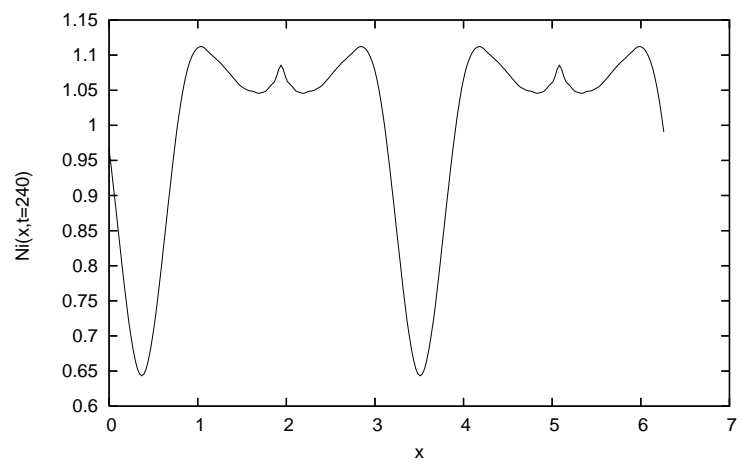
(c) N_i(x,t=240)
