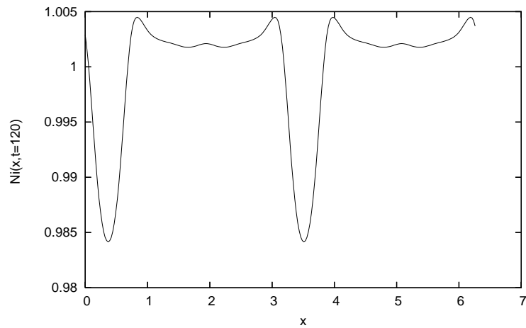
(b) N_i(x,t=120)
