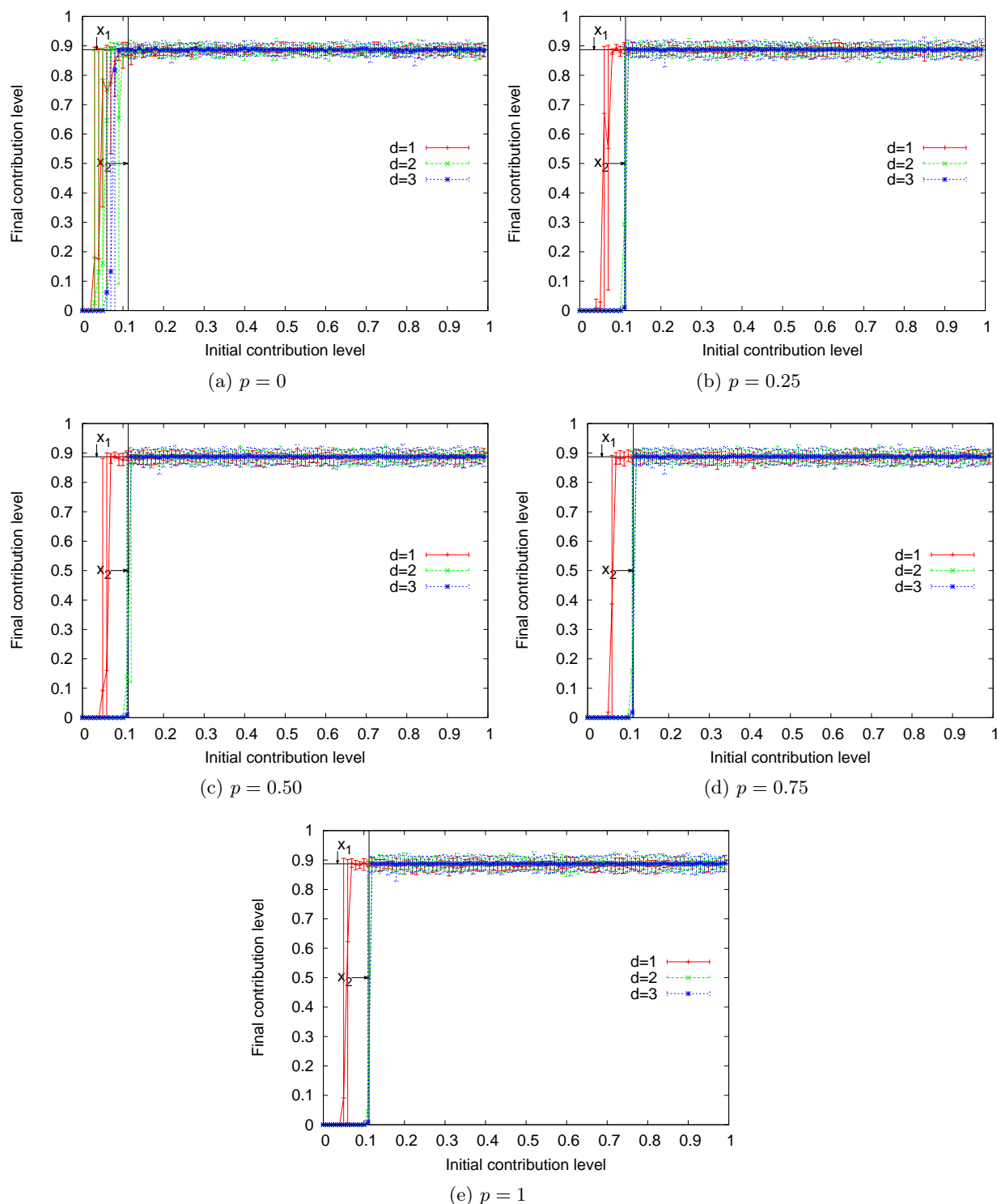
Figure 4.3 – Summary of results of preliminary study on the target. Each figure shows the global dynamics of the network in terms of the “contribution level”. Each image depicts the average contribution level found after 200 time steps and after conducting 1000 repetitions.
