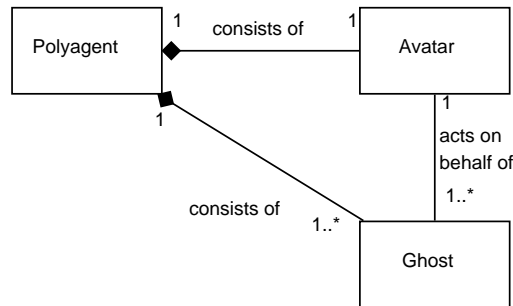
Figure 2.6 – A polyagent represents a domain entity with an avatar and several ghosts.
