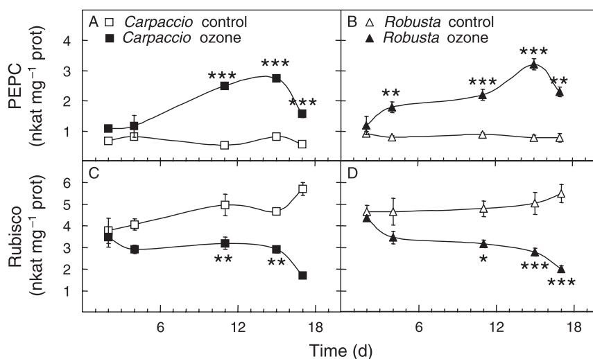
Fig. 5. Effect of O_3 treatment on PEPC activity (A, B) and on Rubisco (C, D) activity (nkat mg^{-1} protein) in leaf protein extracts of Carpaccio (A, C) and Robusta (B, D) genotypes ( n = 4 \pm se ). Significant differences between the O_3 -treated and control leaf extracts are indicated by * ( P < 0.05 ), ** ( P < 0.01 ) and *** ( P < 0.001 ).
