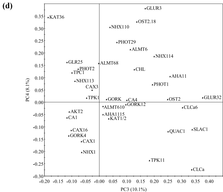
Fig. 5 Principal Component Analysis score plot of PC1 and PC2 (a), PC3 and PC4 (b) and the corresponding PCA loading plots (c and d) of the normalized gene expression in guard cells of the upper (upp) or lower (low) sides of leaves of three poplar genotypes, Carpaccio (orange circles), Cima (green squares) and Robusta (blue triangles) submitted to ambient (A) or ozone treatment (O) after 18 days.
