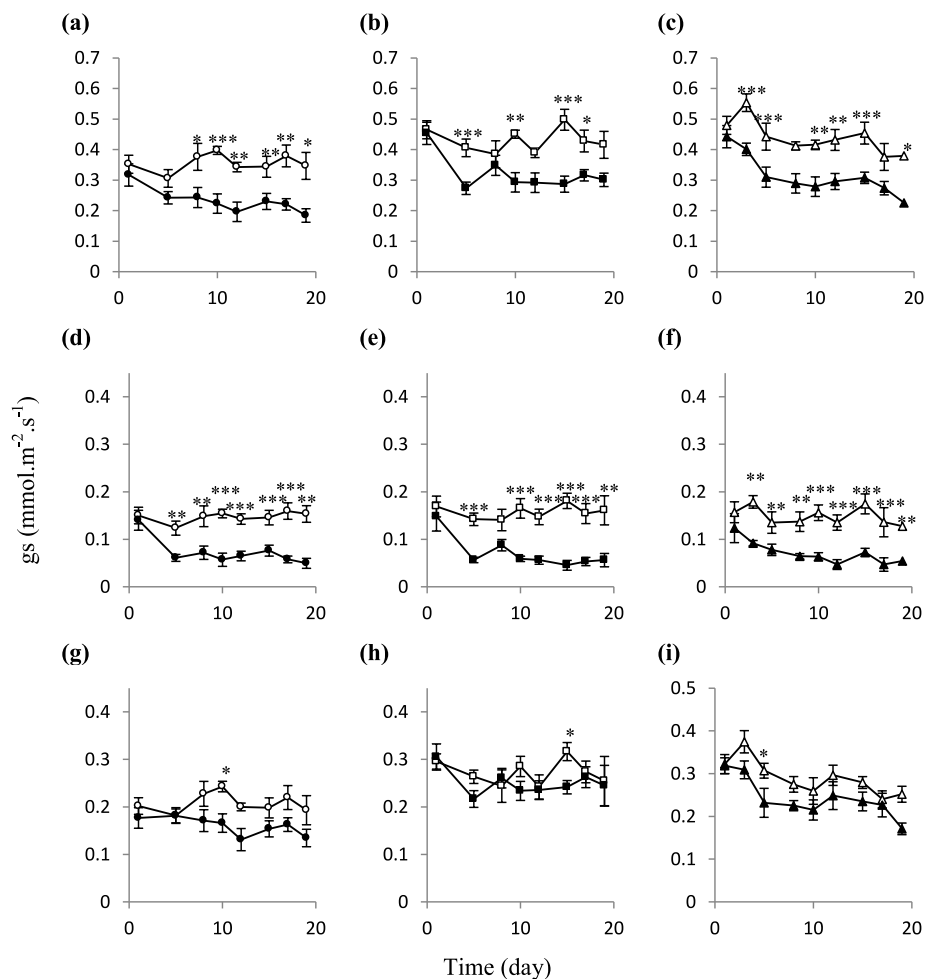
Fig. 1 Effects of ozone (control in white and ozone in black) on stomatal conductance ( g_s ) of leaf ( a , b , c ), of the upper side only ( d , e , f ) and the lower side only ( g , h , i ) of Carpaccio ( a , d , g ) (circles), Cima ( b , e , h ) (squares) and Robusta ( c , f , i ) (triangles). Significant differences between the two treatments are indicated by * ( p < 0.05 ) ** ( p < 0.01 ) or *** ( p < 0.001 ).
