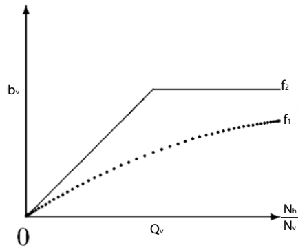
Figure 4.1 – A graphical comparison between f_1 and f_2
