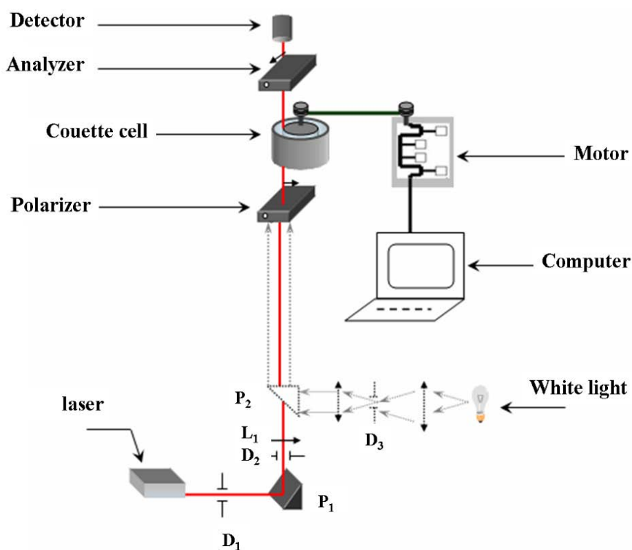
Figure II.9 Schematic diagram of the polarimetric bench
