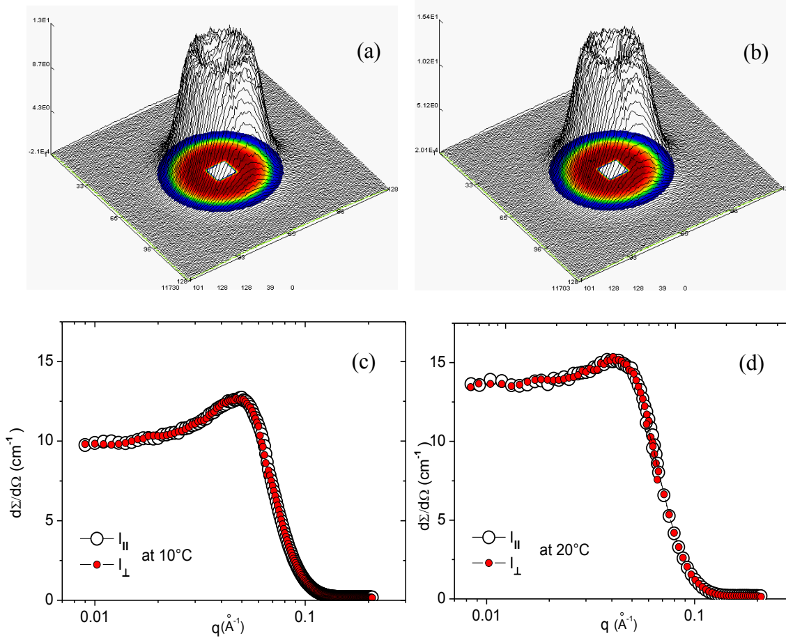
Figure IV.10 Absolute contour plot 3D for the 20 wt % R_7^F(\text{EO})_8 micellar solution (in heavy water) at (a) 10°C at \dot{\gamma} = 0.1 \text{ s}^{-1} and (b) 20°C at rest. The scattered intensity I_{\parallel}(q) and I_{\perp}(q) , at (c) 10°C at \dot{\gamma} = 0.1 \text{ s}^{-1} and (d) 20°C at rest.
