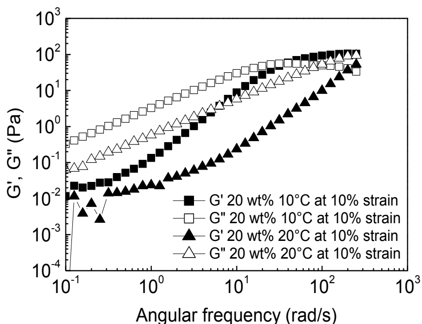
Figure A.3 Storage modulus G' (solid symbols) and loss modulus G'' (open symbols) as a function of the angular frequency \omega by using RFS3: (a) at a constant temperature 20^\circ\text{C} and different R_7^F(\text{EO})_8 concentrations in \text{D}_2\text{O} ; at the concentrations of 20 wt% at 10 and 20^\circ\text{C} .
