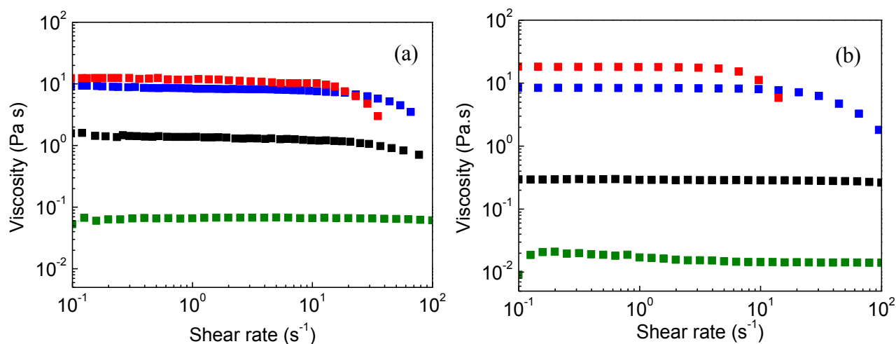
Figure V.2 The viscosity curves as a function of shear rate of R_7^F(EO)_8 at 10^\circ\text{C} ; (a) with NaI solution (b) without NaI salt. At various concentrations 10 wt% (■ green), 20 wt% (■ black), 30 wt% (■ blue) and 40 wt% (■ red).
