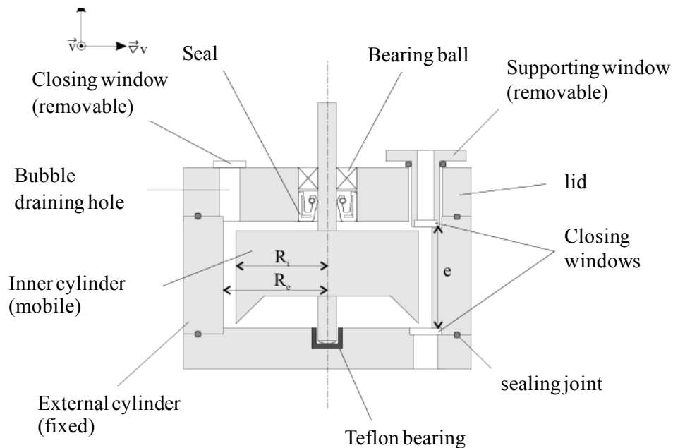
Figure II.10 Couette cell
