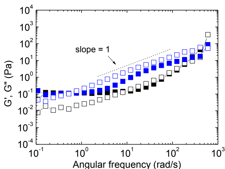
Figure IV.23 Storage modulus G' (solid symbols) and loss modulus G'' (open symbols) as a function of the angular frequency \omega . The concentrations are: 20 (■, □) and 30 (■, □) wt% of R_8^F(\text{EO})_9 in 3M NaCl solution at the constant temperature 10°C.
