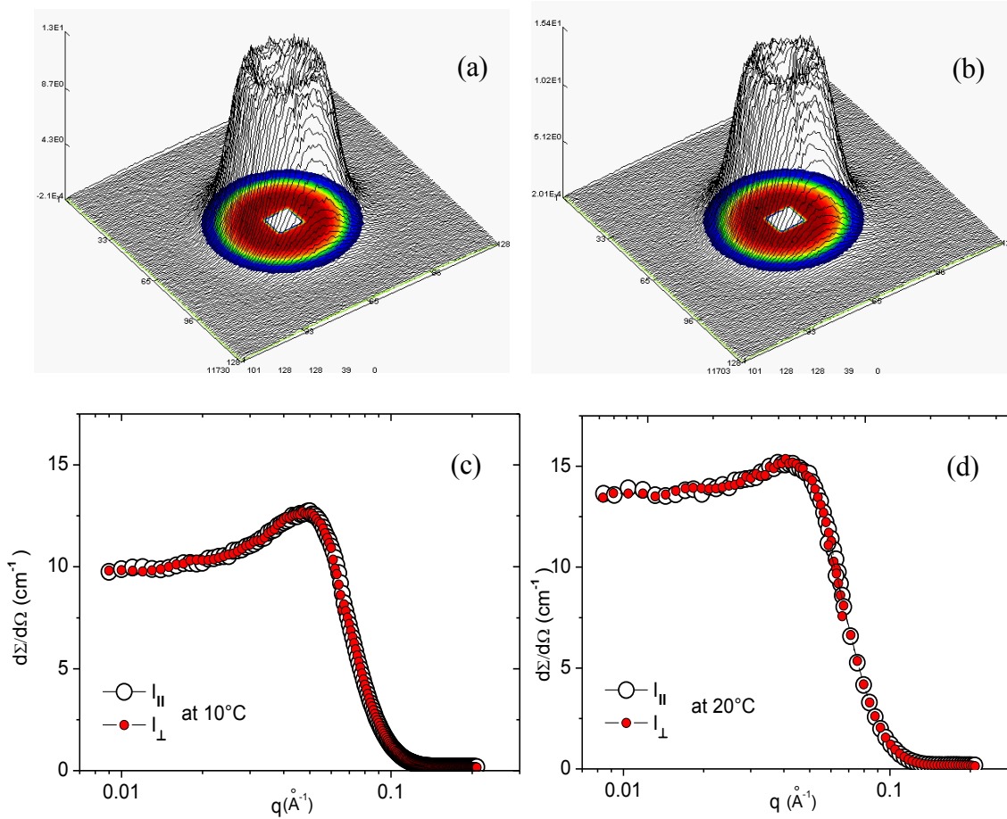
Figure IV.10 Absolute contour plot 3D for the 20 wt % R_7^F(EO)_8 micellar solution (in heavy water) at (a) 10°C at \dot{\gamma} 0.1 s -1 and (b) 20°C at rest. The scattered intensity I_{||}(q) and I_{\perp}(q) , at (c) 10°C at \dot{\gamma} 0.1 s -1 and (d) 20°C at rest.
