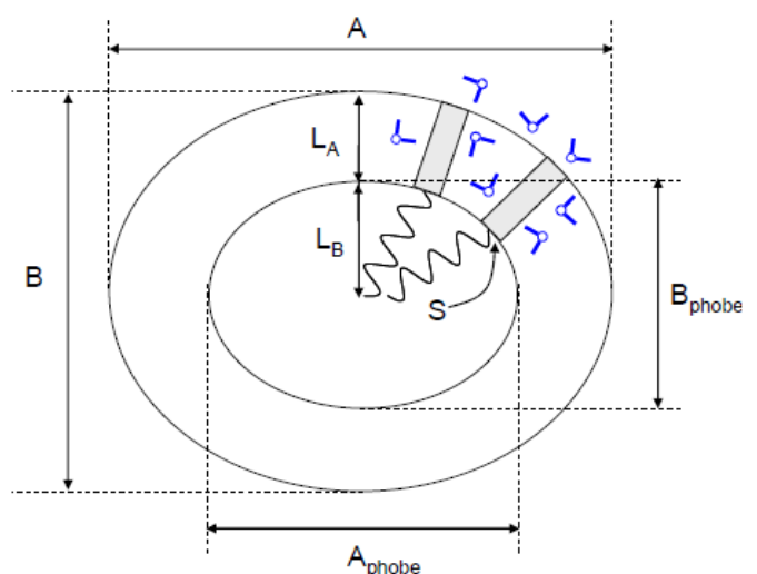
Figure IV.8 Schematic diagrams showing the various parameters defining the geometry of a micelle solution with A , B : size of the particle, A_{\text{phobe}} , B_{\text{phobe}} : dimensions of the hydrophobic core, L_A , L_B : hydrophilic and hydrophobic parts of the micelle and S polar head surface at the hydrophilic / hydrophobic interface.
