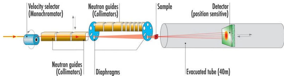
Figure II.16 The D11 line, archetype of a long, pinhole geometry instrument for SANS [10].
