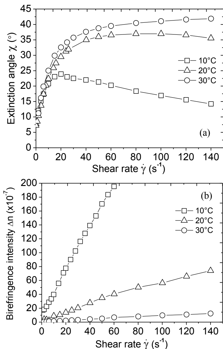
Figure IV.7 Flow birefringence experiments: (a) extinction angle \chi , (b) birefringence intensity \Delta n vs. the shear rate. The concentration is 20 wt % R_7^F(\text{EO})_8 in water and the temperature 10°C ( \square ), 20°C ( \triangle ) and 30°C ( \circ ).
