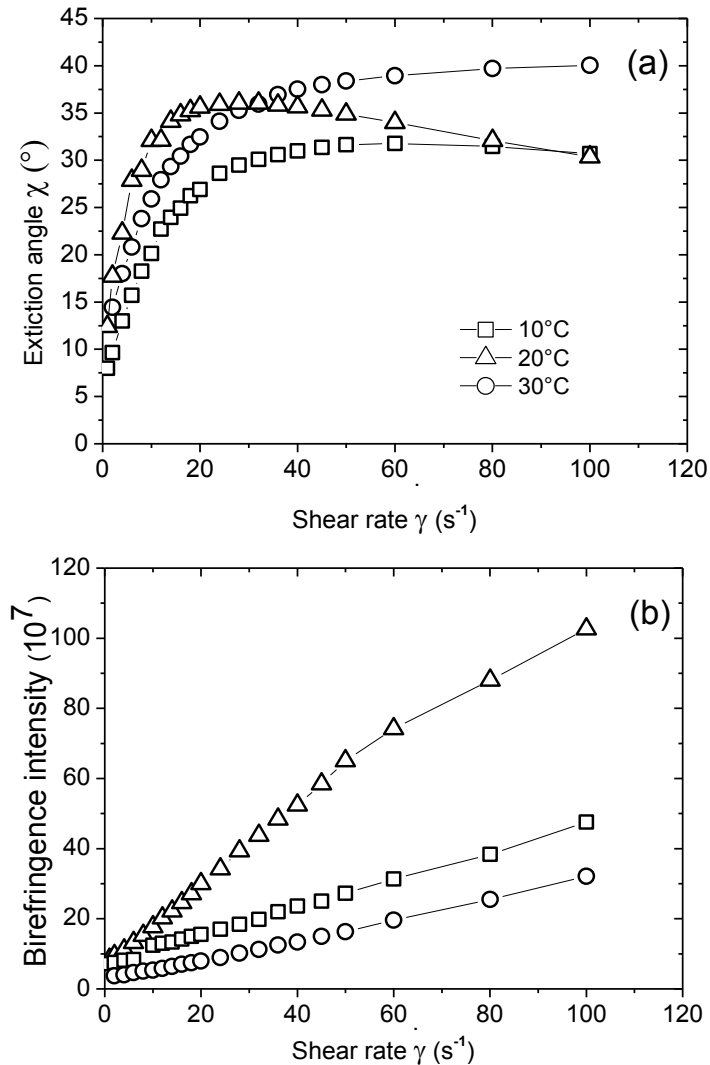
Figure IV.19 Flow birefringence experiments: (a) extinction angle \chi , (b) birefringence intensity \Delta n vs. the shear rate \dot{\gamma} . The concentration is 20 wt % R_7^F(\text{EO})_8 1M NaI solution and the temperatures: 10^\circ\text{C} ( \square ), 20^\circ\text{C} ( \triangle ) and 30^\circ\text{C} ( \circ ).
