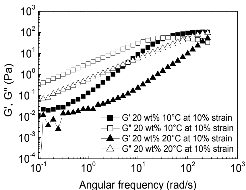
Figure A.3 Storage modulus G' (solid symbols) and loss modulus G'' (open symbols) as a function of the angular frequency \omega by using RFS3: (a) at a constant temperature 20^\circ C and different R_7^F(EO)_8 concentrations in D_2O ; at the concentrations of 20 wt% at 10 and 20^\circ C .
