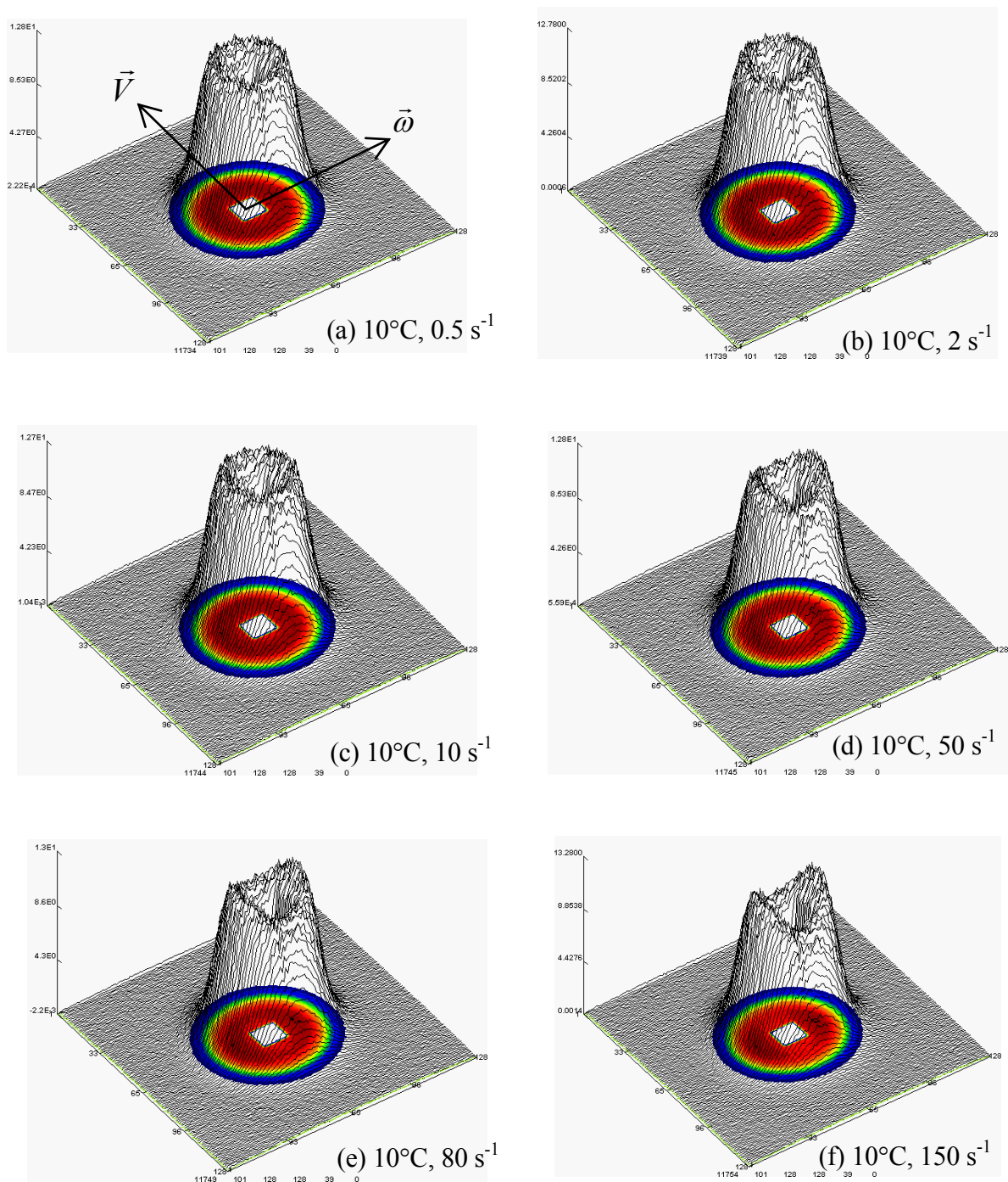
Figure IV.12 Iso-intensity surface plots at the temperature of 10^{\circ}\text{C} for the 20 wt % micellar solution (in heavy water). Six values of the shear rates \dot{\gamma} were used: (a) 0.5\text{ s}^{-1} , (b) 2\text{ s}^{-1} , (c) 10\text{ s}^{-1} , (d) 50\text{ s}^{-1} , (e) 80\text{ s}^{-1} and (f) 150\text{ s}^{-1} .
