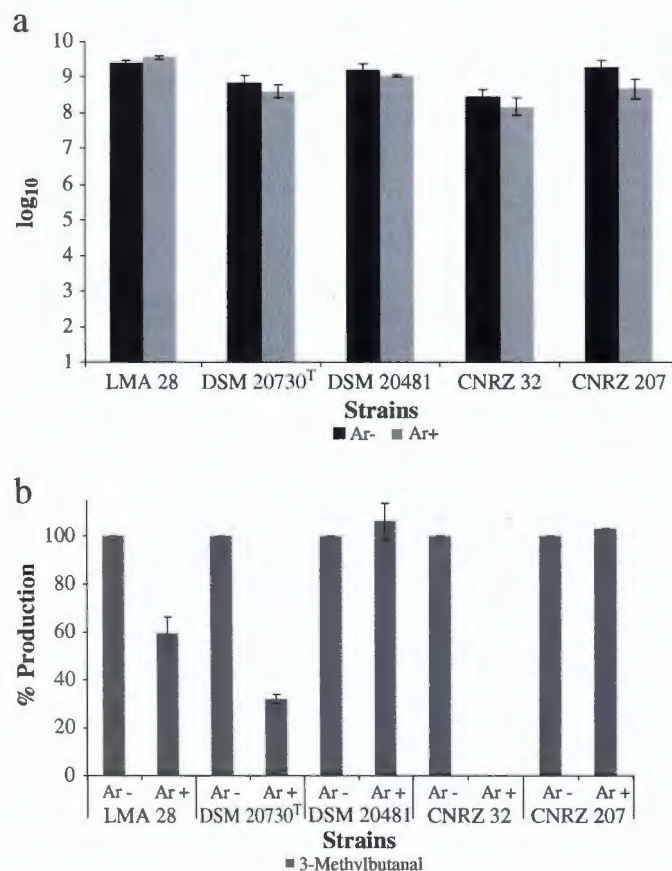
Fig. 2. a) Effect of NaAsO 2 (10 mM) on the bacterial cells' growth and b) on the production of 3-methylbutanal from leucine catabolism in a reaction medium containing leucine, α-KG, PLP in the absence (Ar-) or presence (Ar+) of NaAsO 2 by the strains studied after 48 h: LMA 28: Carnobacterium maltaromaticum ; DSMZ 20730 T : C. maltaromaticum ; DSMZ 20481: Lactococcus lactis ; CNRZ 32: Lactobacillus helveticus ; and CNRZ 207: Lb. delbrueckii subsp. lactis .
