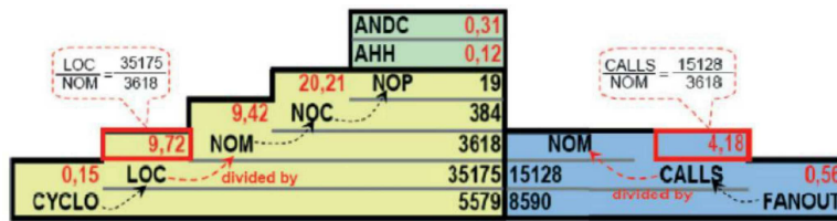
FIGURE 2.1 – Overview Pyramid [LM06]
