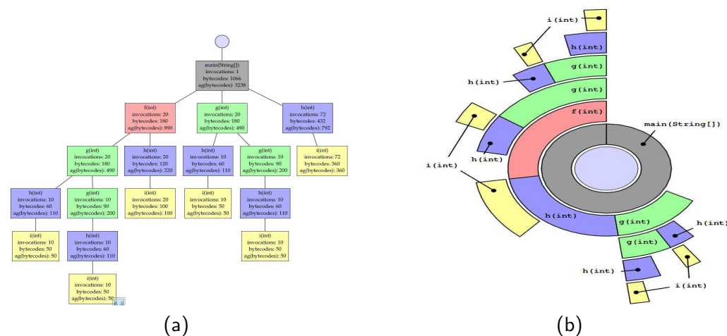
FIGURE 5.3 – (a) Calling Context Tree, (b) Calling Context Ring Charts [MBAV09].
