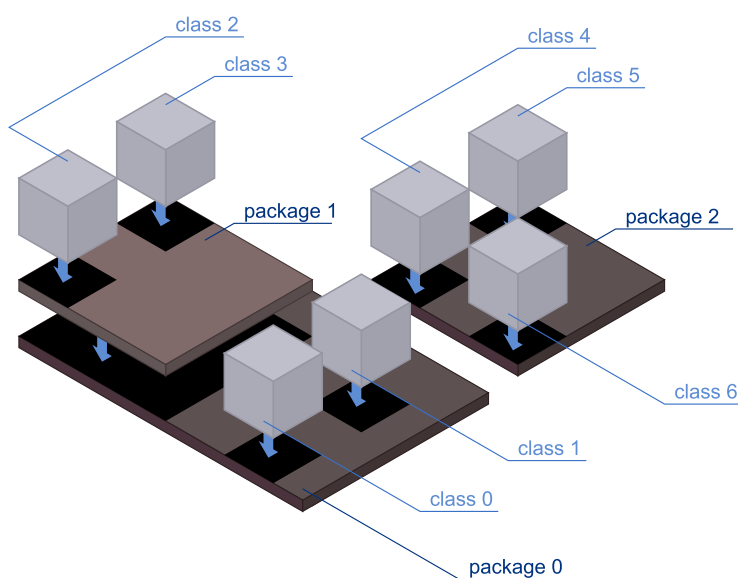
FIGURE 7.2 – Notre placement imbriqué
