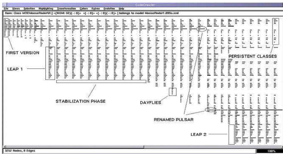
FIGURE 3.28 – Evolution Matrix from [LD02]
