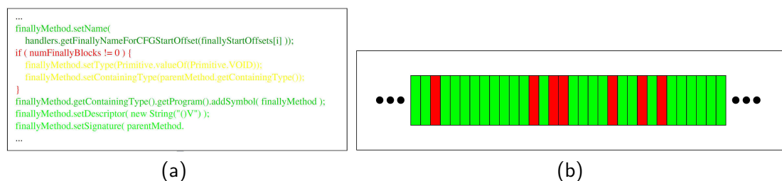
FIGURE 5.1 – (a) Code source coloré, (b) Execution Bar provenant de [OJH03].
