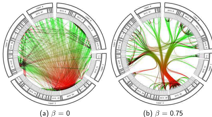
FIGURE 3.13 – Hierarchical Edge Bundles [Hol06].
