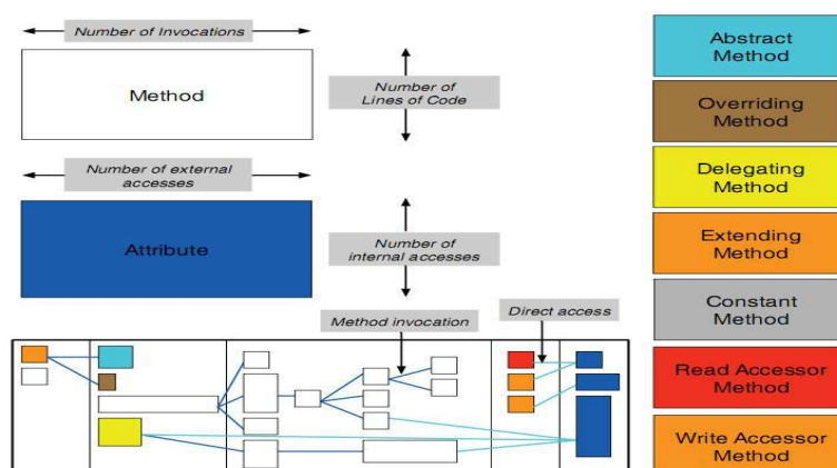
FIGURE 3.2 – Class Blueprint [LM06].
