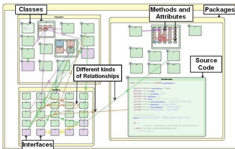
FIGURE 3.12 – Nested boxes visualization from SHriMP.
