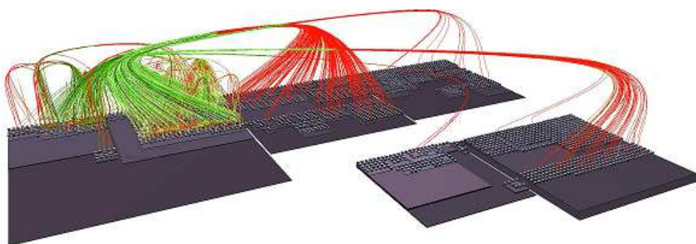
FIGURE 7.12 – \beta = 0.4
