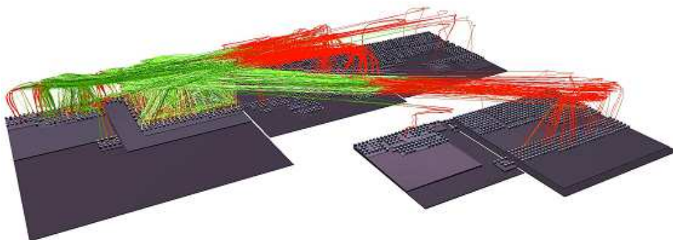
FIGURE 7.12 – \beta = 0.4
