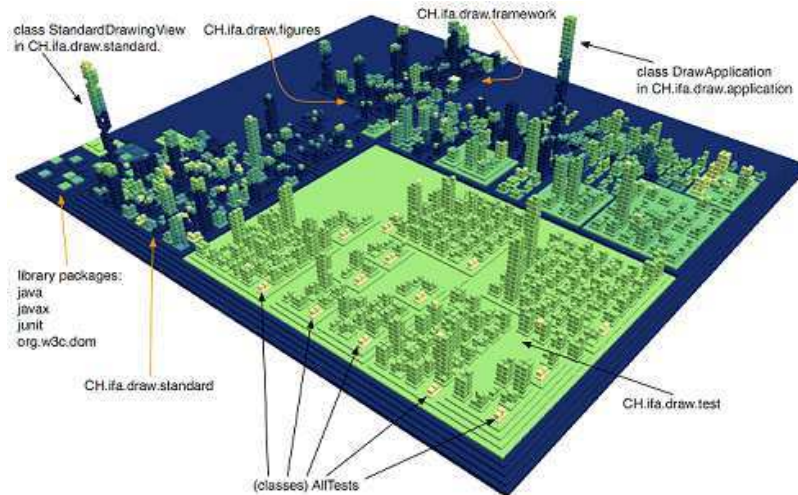
FIGURE 3.30 – Fine-grained Age Map of JHotDraw from [WL08a]
